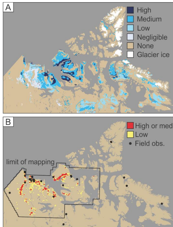
Figure 5. a) Modelled abundance of massive ice and; b) abundance of large (>1 ha) thaw slumps in northwest Canada (Kokelj et al., 2017; Segal et al., 2016), and field observations of massive ice from the literature (Table S3).
