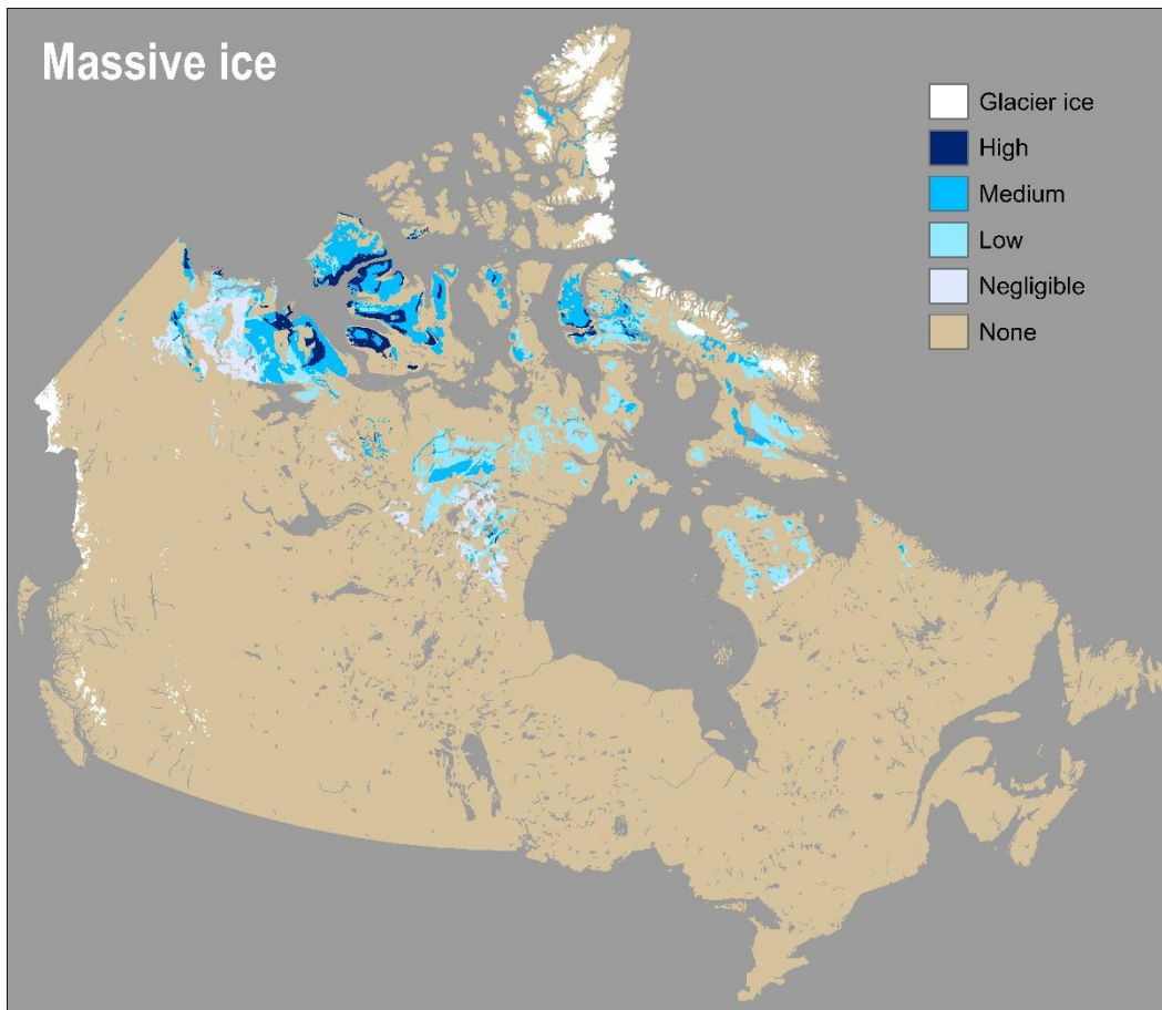
Figure 2. Modelled massive ice abundance.
