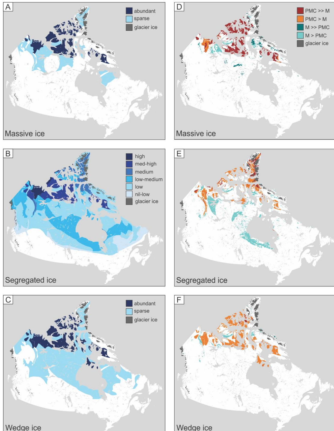
Figure 8. The Permafrost map of Canada (PMC) depictions of (a) massive ice, (b) segregated and intrusive ice, and (c) wedge ice (modified from Heginbottom et al., 1995); Comparison between the PMC and the models (M). PMC >> M indicates, for example, that the reclassified relative ground ice abundance on the PMC is 'high' and the modelled abundance is 'none'. M > PMC indicates the reclassified ground ice abundance is 'high' on the model output and 'low' on the PMC. See Table 2 and text.
