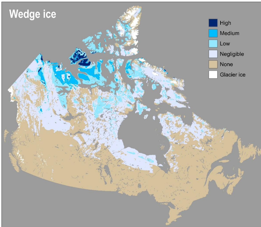
Figure 4. Modelled wedge ice abundance.
