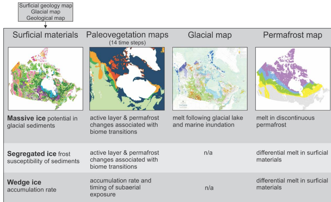
Figure 1. General model framework indicating datasets used and processes represented for the three ground ice types.
