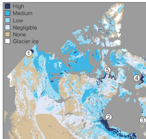
Figure 5. a) Modelled abundance of massive ice and; b) abundance of large (>1 ha) thaw slumps in northwest Canada (Kokelj et al., 2017; Segal et al., 2016), and field observations of massive ice from the literature (Table S3).
