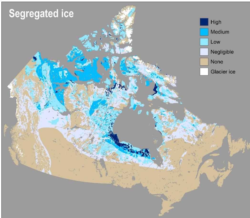
Figure 3. Modelled segregated ice abundance.
