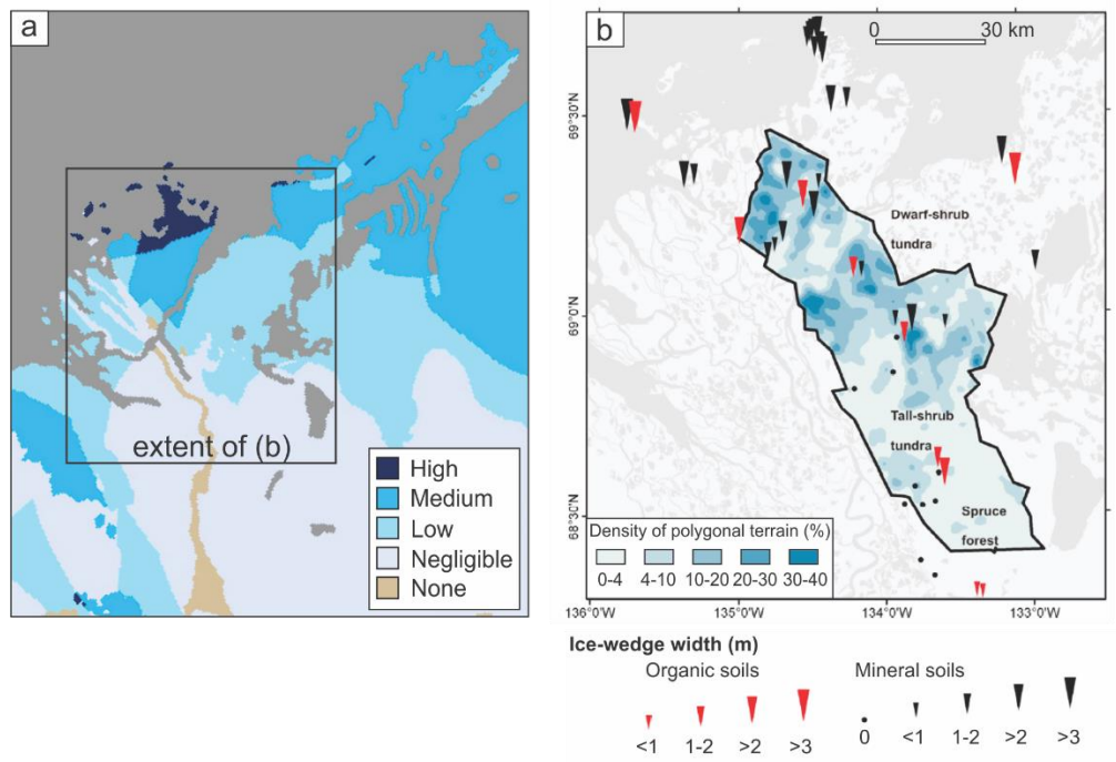
Figure 7. Comparison of (a) modelled wedge ice abundance to (b) wedge widths and the density of polygonal terrain in the western Canadian Arctic (modified from Kokelj et al., 2014, Fig. 6).
