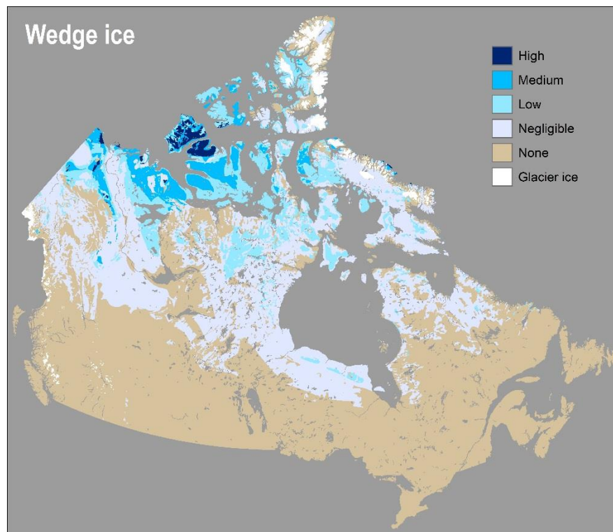
Figure 4. Modelled wedge ice abundance.
