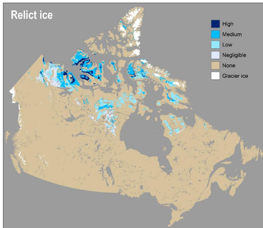
Figure 2. Modelled relict ice abundance.
