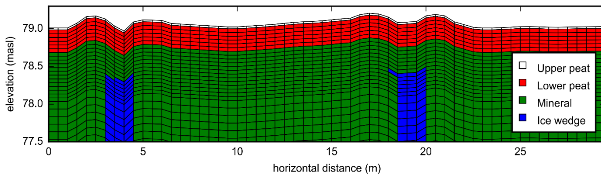
Figure 3. Schematic of the 2D mesh of the field site (vertical exaggeration=4)
