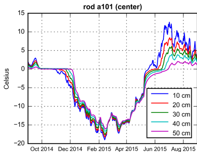
Figure 2. Sample of observed temperature data from rod a101 (polygon center).
