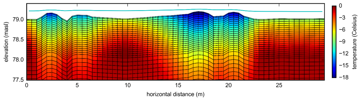
Figure 7. Snapshot of simulated snowpack surface (cyan line) and ground temperature on December 24, 2014 (vertical exaggeration=4).
