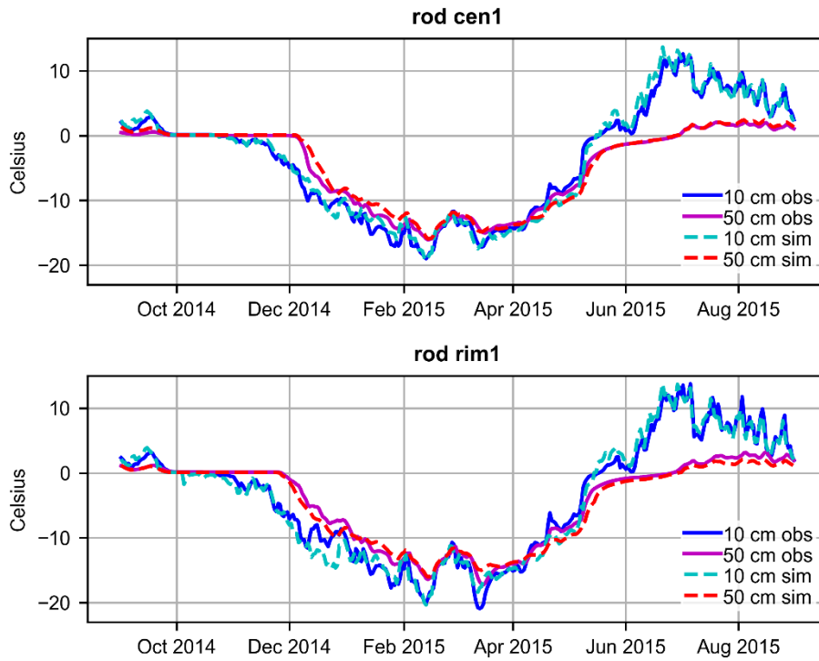
Figure 6. Observed and simulated ground temperature from calibrated 2D simulation, at rods cen1 and rim1.
