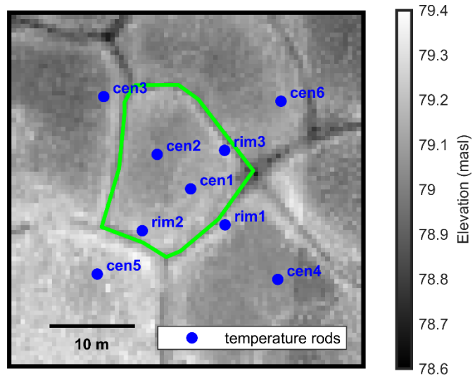
Figure 1. 50 cm resolution lidar DEM of field site.
