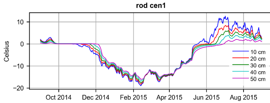
Figure 2. Sample of observed temperature data from rod a101 (polygon center).
