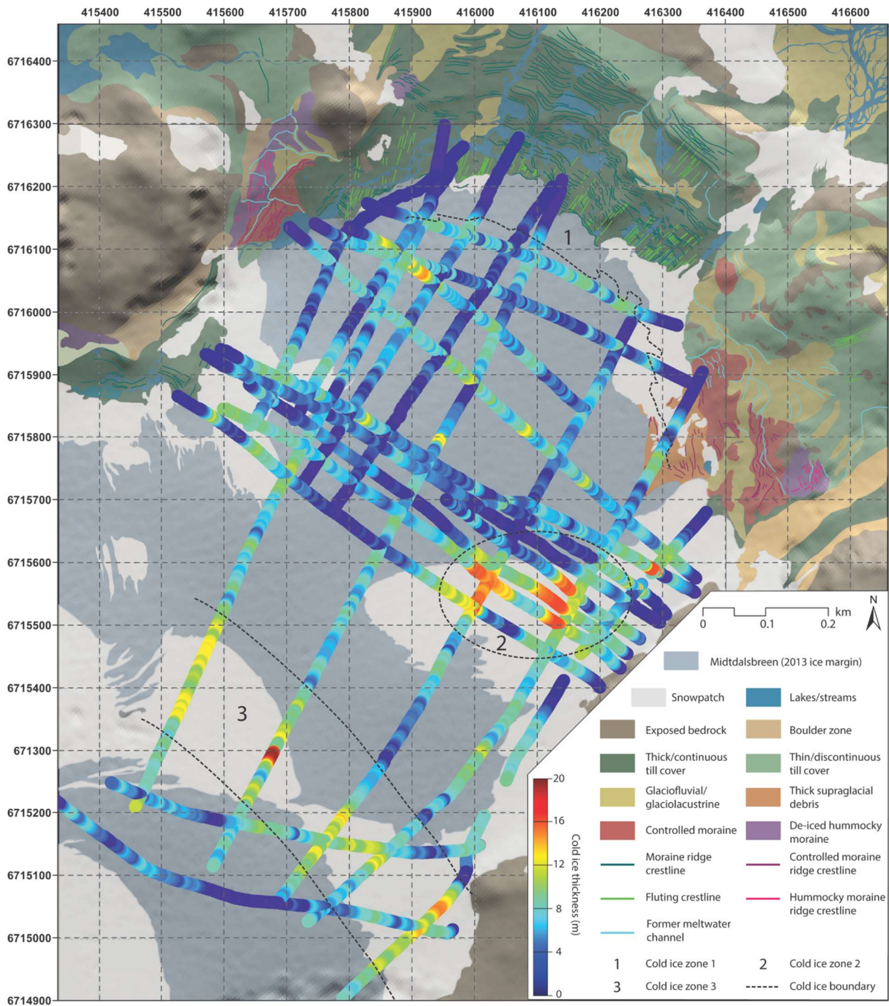
Figure 67: Estimates of cold-ice thickness estimates on Midtdalsbreen from selected GPR profile tracks. Three cold-ice zones, CIZ1-CIZ3 are indicated. A corridor of 40 to 50 m of cold-based frozen basal ice extending to the glacier bed is present at the glacier snout (CIZ1). Also included is a detailed geomorphological map of the glacier foreland which highlights the distinct difference between the NW and SE part of the foreland linked to the varying thermal regime measured in the GPR data.
