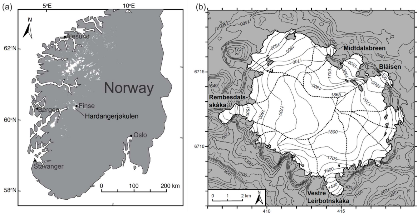
Figure 1: (a) Map of south central Norway with major ice bodies indicated in white (modified from Giesen, 2009). (b) Hardangerjøkulen icefield map created from a 1995 digital elevation model by Statens Kartverk (modified from Giesen, 2009). The reference system is UTM zone 32 (EUREF89), 50 m and the contour interval is 50 m. The dashed lines indicate the estimated extent of the drainage basins of the different outlet glaciers (Andreassen and Elvehøy, 2001).
