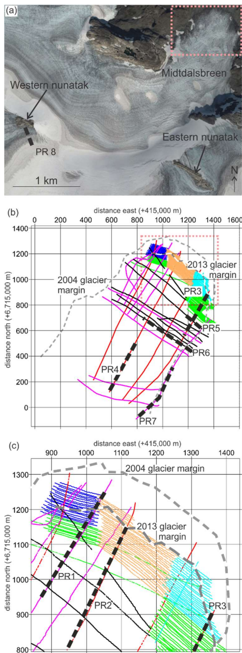
Figure 4: (a) Locations of western and eastern nunataks in the upper accumulation area of Midtdalsbreen, (from Google Earth imagery 0 taken on the 4/09th September/2014). Note by this time in the melt season most snow nearly all patches of snow have melted from the glacier surface. Dashed black line shows location of profile (PR) 8 (Fig. 9) shown in figure 8. Pink dashed box shows (b) locations of GPR surveys (coloured areas and solid lines) acquired on Midtdalsbreen (coloured areas and solid lines), between 20th-26/04th April/2014, with the 2004 and 2013 glacier margin (dashed grey) digitised from Google Earth. Thick black dashed line indicates locations of profiles (PR) 3-7 (displayed in Figs. 5c; 86a-d). Pink dashed box shows (c), enlarged window of dense
