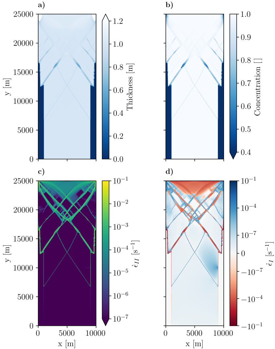
Figure 6. Sea ice thickness (a), concentration (b), maximum shear strain rate (c) and divergence (d) after 45 min of integration (2700 sec) in a uni-axial loading test. To make these longer simulations possible, both non-linear and linear iterations are limited to 150 per timestep. Results show the development of secondary fracture lines in all fields after the first fracture line has formed.
