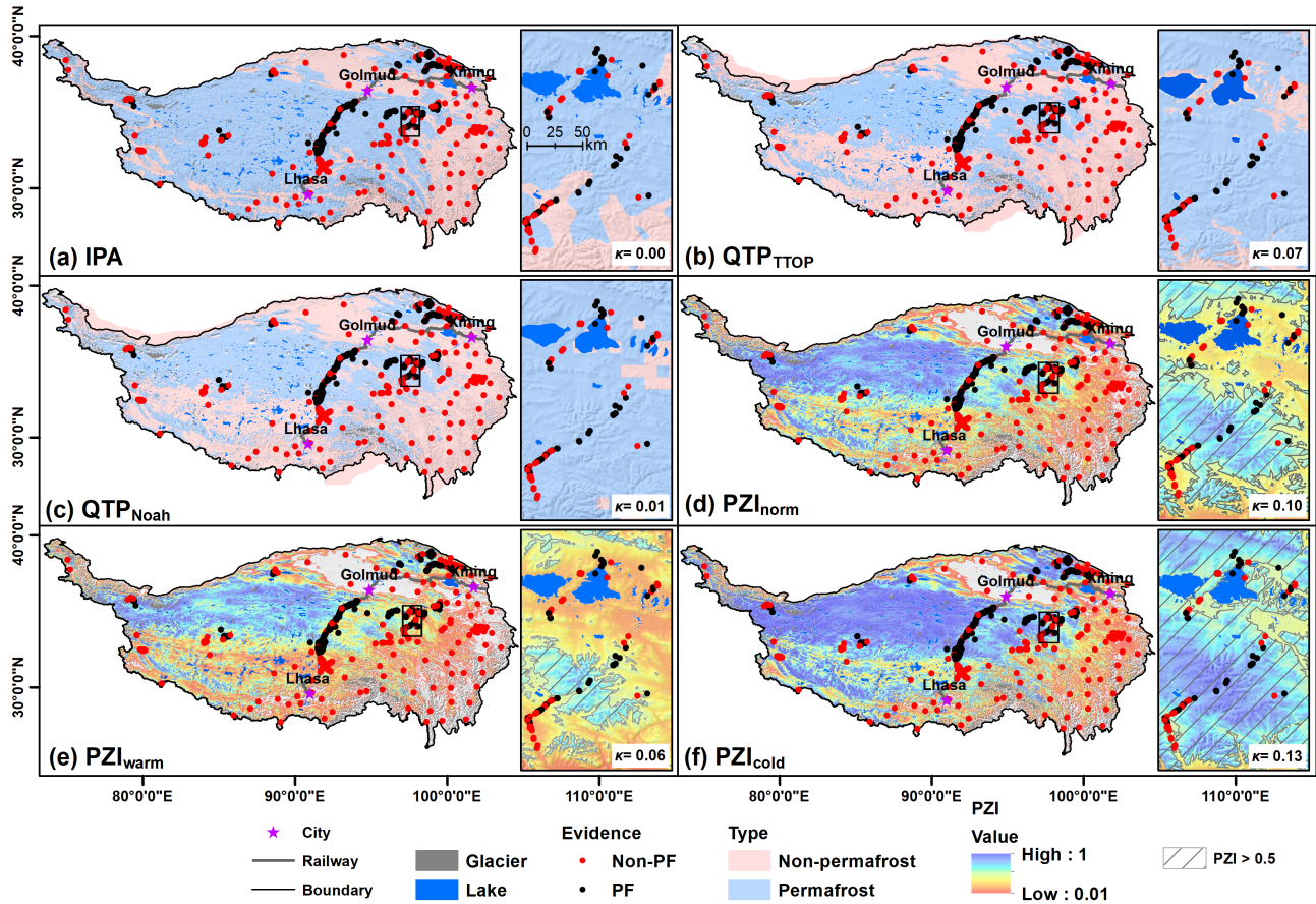
Figure 2. The permafrost classification results at in-situ evidence sites/plots in the (a) IPA, (b) QTP TTOP , (c) QTP Noah , (d) PZI norm , (e) PZI warm , and (f) PZI cold maps. \kappa and PCC are the evaluation results for the selected spatially highly variable landscapes (marked by black box). All the maps are re-sampled to the unprojected grid of SRTM30 DEM with a resolution of 30 arcsec ( \sim 1 km) to avoid maps bias of with different resolutions, geographic projection, and format. The boundary of QTP used in this study is marked by black line. Categorical classification is used for the QTP TTOP , QTP Noah , and IPA maps, while continuous PZI was present for the PZI norm , PZI warm , PZI cold maps. The blank part in PZI maps is area with PZI < 0.01. The \kappa and PCC_{tot} present in right small figures were evaluated in the selected areas with 106 evidence.
