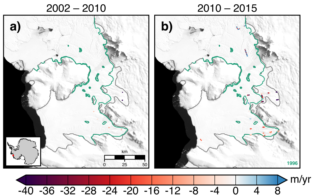
Fig. 1. Ice thickness change of the Dotson and Crosson Ice Shelves from a) 2002–2010 and b) 2010–2015
