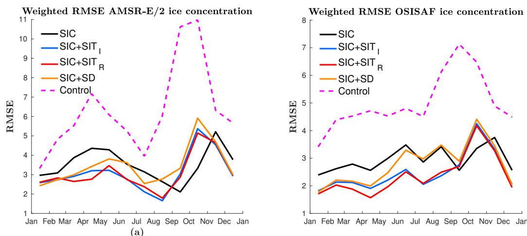
Figure 8. RMSE of a seven day monthly averaged ensemble average of modelled SIC forecast validated by a) AMSR-E/2 SIC observations and b) OSISAF SIC observations.
