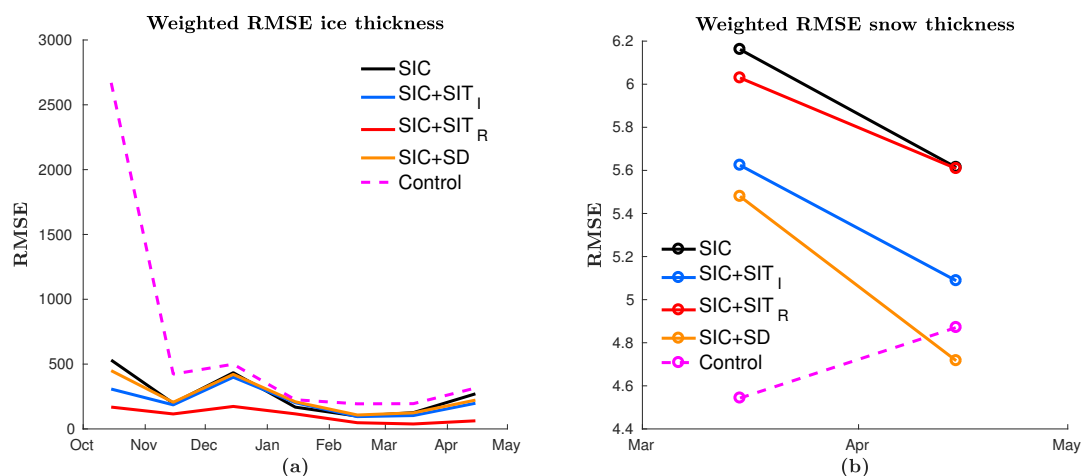
Figure 5. RMSE of monthly averaged model SIT and snow depth averaged over all ensemble members calculated against observed a) ice thickness and b) snow depth. The colour coding is as in Fig. 2.
