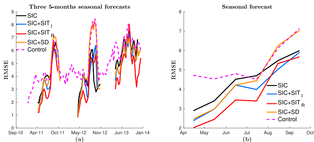
Figure 9. Seasonal forecast of summer sea-ice extent. Each forecast started at the beginning of April every year. The figures show SIC RMSE averaged over all ensemble members. The coloured lines represent the same as in figure 2. In a) Full period, in b) monthly averaged values.
