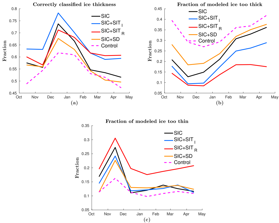
Figure 6. The monthly mean SIT averaged over all ensemble members is classified into four thickness categories and compared to the CryoSat-SMOS SIT observation product. The fraction of grid cells are shown with a) correctly classified thickness category, b) too thick ice, and c) too thin ice. As in Fig. 2 the coloured lines represent different experiments.
