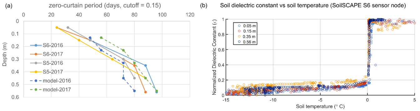
Figure 4: Soil freezing characteristics at the Prudhoe Meadow SoilSCAPE site: (a) comparisons of model and observed zero-curtain period at two sensor nodes (S5 and S6) using a cutoff threshold of 0.15 (Eq. 12) for both in-situ soil dielectric constant and model simulated unfrozen water content to determine soil freeze onset; b) changes in in-situ soil dielectric constant during soil freezing at the S6 node. The soil dielectric constant was normalized using the maximum and minimum value of soil dielectric constant during the observation period.
