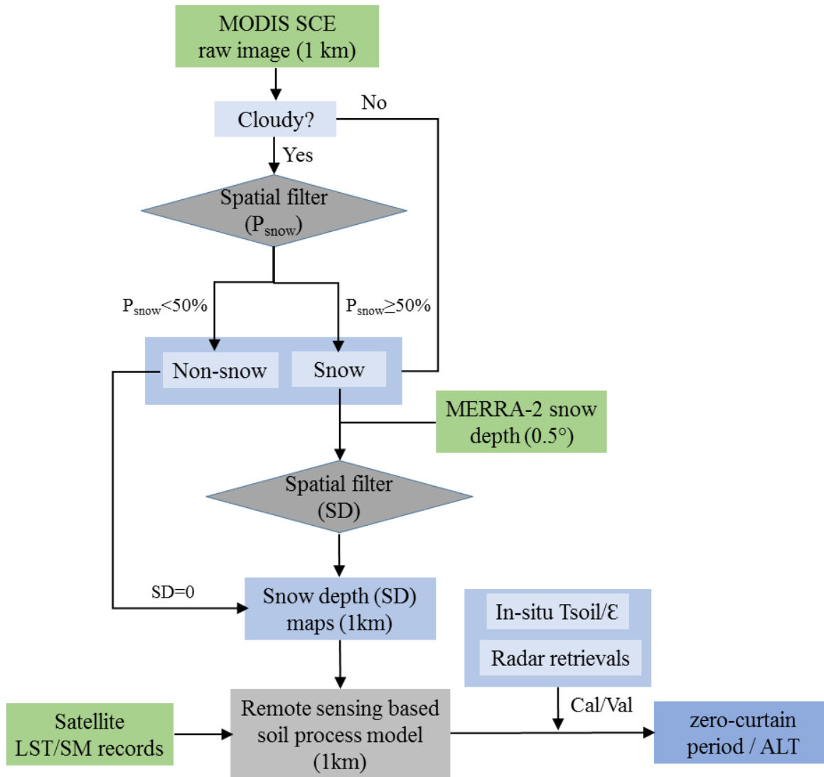
5 Figure 1: Flow diagram describing the snow data processing and soil modelling procedure. A spatial filter was used to predict the snow occurrence probability for MODIS cloud-contaminated pixels. Based on the cloud-free MODIS SCE imagery, the snow depth of each snow-covered 1-km pixel was estimated from the snow depth of the neighbouring MERRA-2 grid cells with weights predicted using another spatial filter. The downscaled 1-km snow depth data was then used to drive a remote sensing based soil process model to simulate the zero-curtain period and ALT. Both the snow data processing and soil modelling were carried out at 8-day time step.
