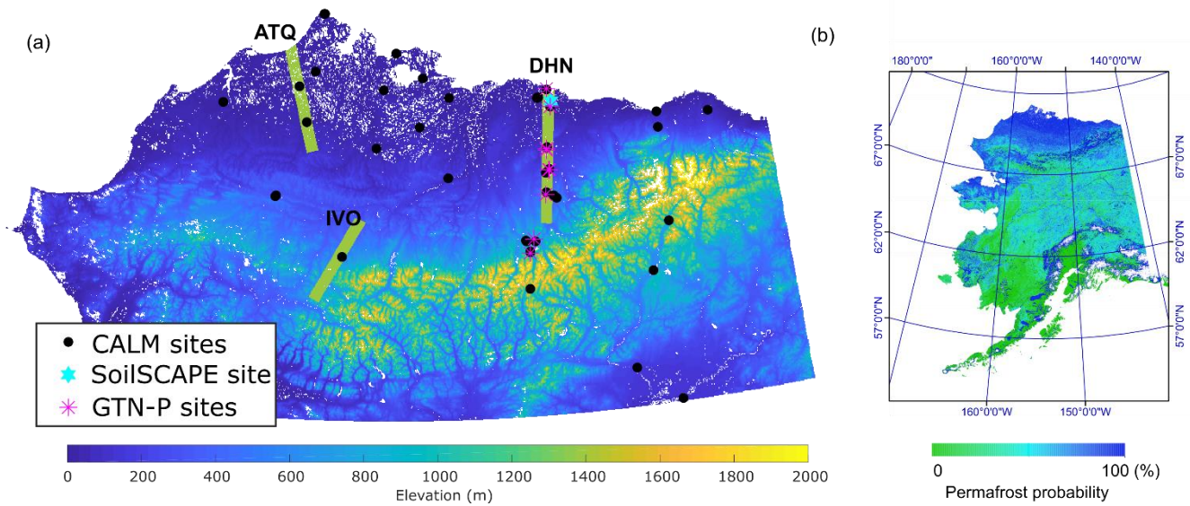
Figure 2: a) The study area (Arctic Alaska, >66.55^\circ N) used for the soil model simulations and the locations of in situ sites used for model calibration and validation; b) an Alaska permafrost probability map (Pastick et al., 2015) is also shown, indicating higher permafrost occurrence in Arctic Alaska. The in-situ sites include the Prudhoe Meadow SoilSCAPE site, GTN-P soil temperature sites and CALM ALT sites. Airborne P-band radar data (denoted by green lines) were obtained in late August and early October in 2014 and 2015. Another radar flight line was collected over the Barrow area (not shown), but was not included in this analysis due to a large percent of surface water in this area.
