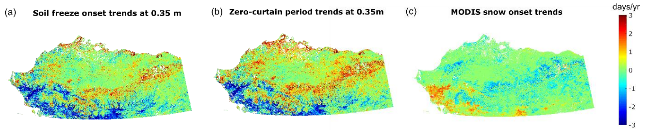
Figure 9: Trends in model simulated soil freeze onset (a) and zero-curtain period (b) at 0.35 m depth from 2001 to 2016. The autumn snow onset trend for the same period derived from the MODIS SCE data is shown in (c).
