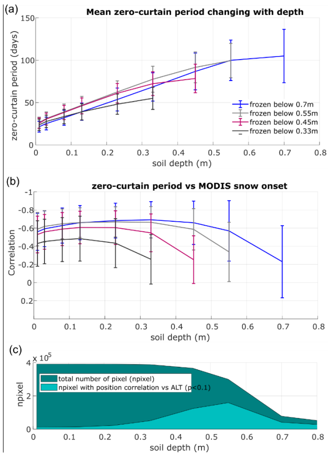
Figure 10: Regional statistics of model simulated zero-curtain period (a) and its sensitivity to MODIS snow onset and model simulated ALT (b-c) from 2001 to 2016: a) regional mean of model simulated zero-curtain period at different depths; b) changes in correlations between snow onset and zero-curtain period with depths; for both a) and b), the study area was divided into 4 groups: soil column froze below 0.33 m, 0.45 m, 0.55 m, and 0.7 m. The soil column for the majority of the study area froze below 0.7m. c) The proportion of pixels with significant positive correlation between zero-curtain period and ALT at different depths. The total number of unfrozen pixel was shown as “npixel”.
