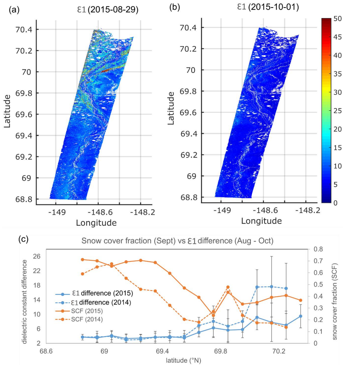
5 Figure 7: Soil freeze process indicated by the radar retrieved (Chen et al., in press) soil dielectric constant ( \epsilon_1 ) of surface soils ( \sim 0.10 m) at the DHN transect in August (a) and October (b), and changes in \epsilon_1 in relation to MODIS SCF (c). The \epsilon_1 differences between August and October were binned to 0.1^{\circ} latitudinal bin, while SCF was calculated as the percentage of snow covered pixels indicated by MODIS SCE data for each 0.1^{\circ} bin. The standard deviation of \epsilon_1 differences for each 0.1^{\circ} bin was shown as error bars.
