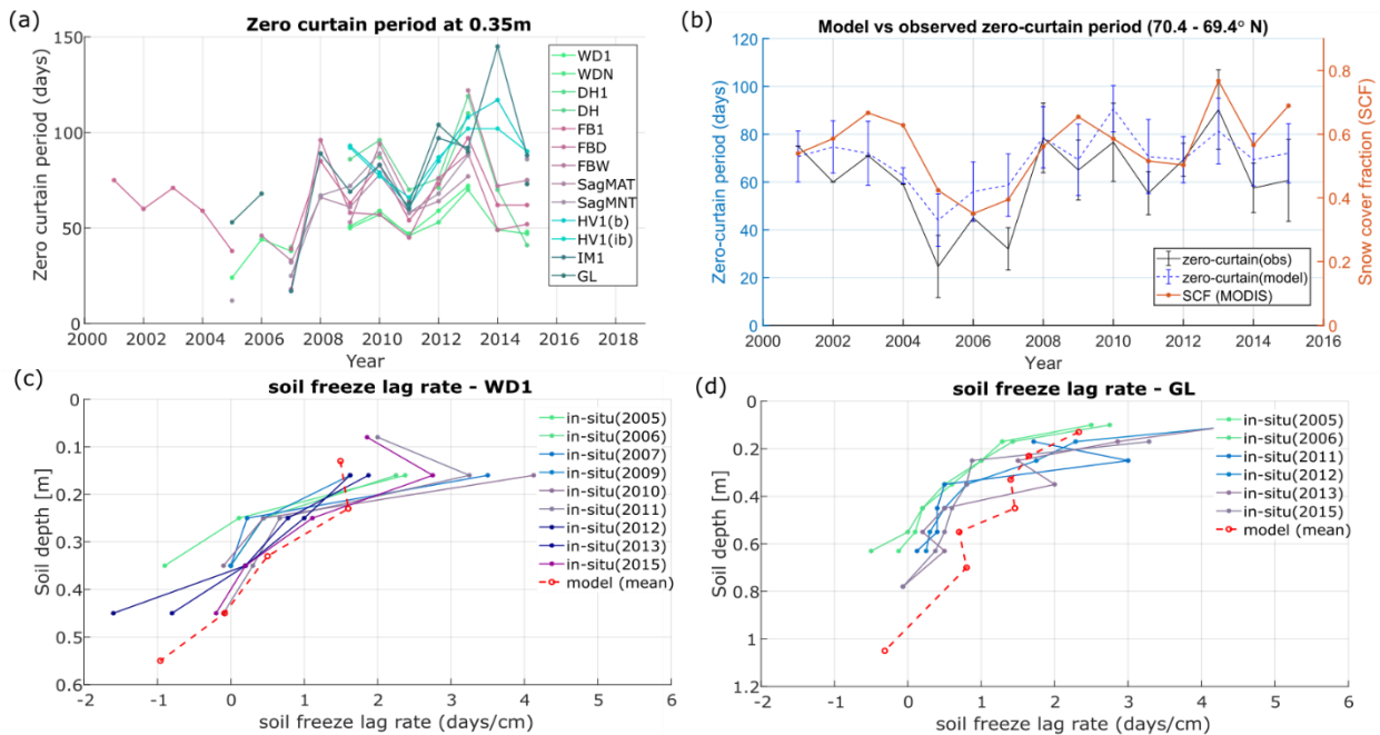
Figure 6: Comparisons of soil freezing characteristics derived from GTN-P soil temperature measurements and model simulations along the DHN transect in northern Alaska: a) inter-annual variations in zero-curtain period derived from in-situ measurements; b) variations of model versus in-situ zero-curtain period at 0.35 m soil depth relative to MODIS SCF averaged for the northern part of the DHN transect; c-d) changes in the soil freeze lag rate with depth at two DHN sites. Both sites have lower ALT in the earlier years shown here, ranging from 0.37 m in the earlier period to 0.43 m during later period of record for the WD1 site, and from 0.47 m to 0.57 m for the GL site.
