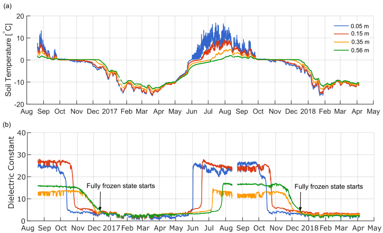
Figure 3: In-situ measurements of soil temperature (a) and dielectric constant (b) for a single SoilSCAPE sensor node (S6) at the Prudhoe Meadow site in northern Alaska ( http://soilscape.usc.edu ).
