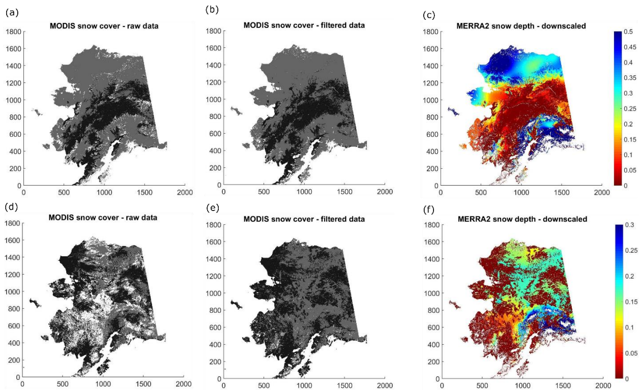
5 Figure 5: Illustration of the snow data processing: the raw (a&d) and cloud filtered (b&e) MODIS SCE images using an elevation-based spatial filter and downscaled MERRA-2 snow depth (m) data (c&f) using the filtered MODIS SCE and DEM data during spring snow melt (top: 04/23-04/30) and early snow accumulation (bottom: 09/30-10/07) period in 2007. In the MODIS images, snow covered areas are shown as gray, while land and cloud covered areas are shown as black and white, respectively.
