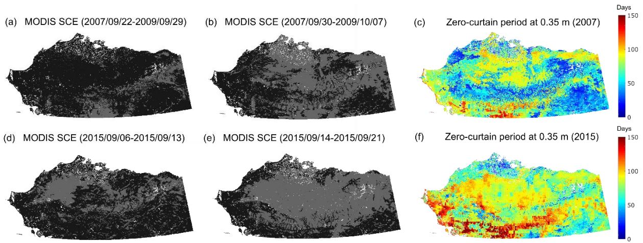
Figure 8: Model simulated zero-curtain period at 0.35 m in relation to snow accumulation during early snow season indicated by filtered MODIS SCE images for two selected years with later (2007: a-c) and earlier (2015: d-f) snowfall. In the MODIS images, snow was shown as dark gray, while land was shown as black and the areas masked out were shown as white.
