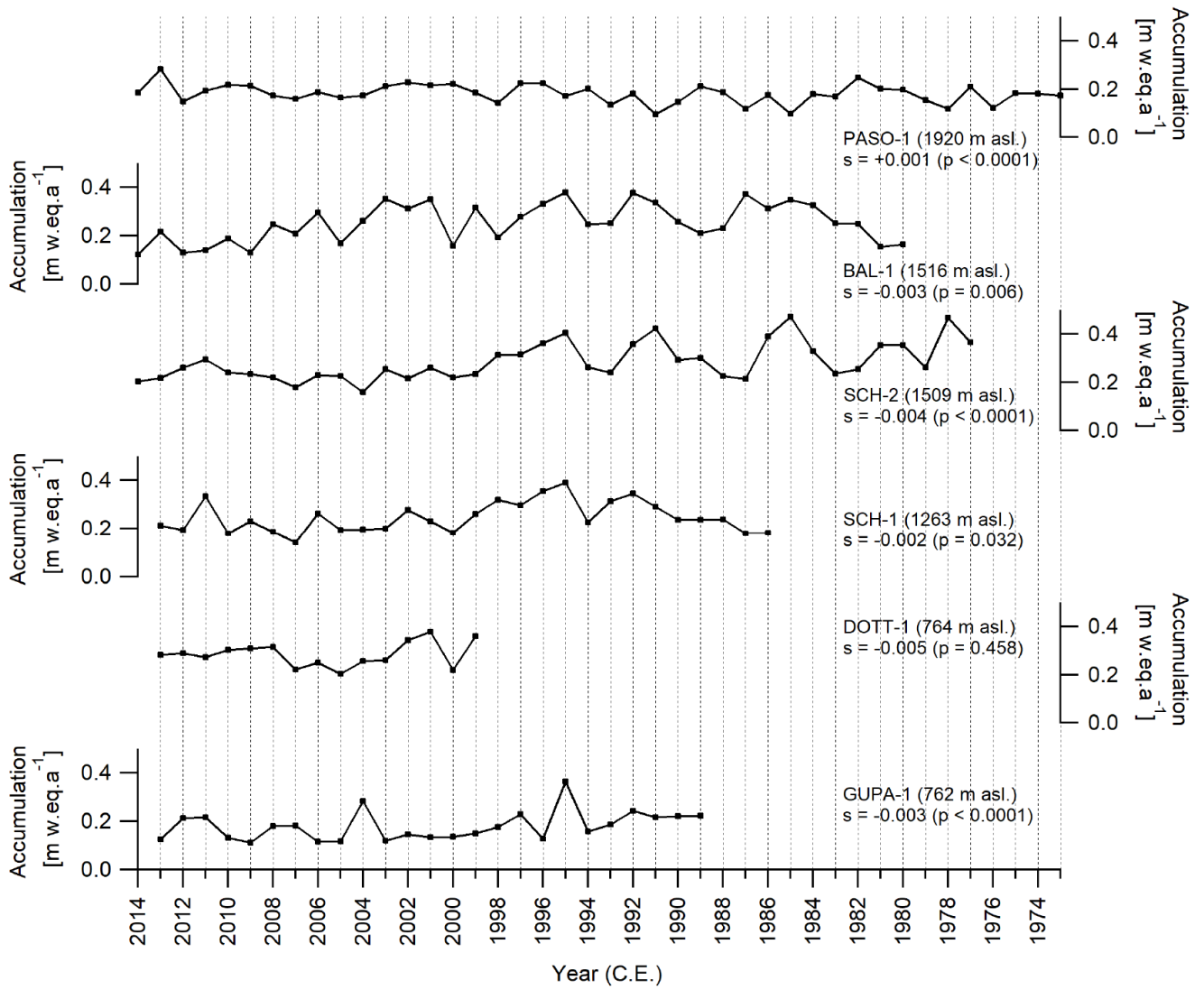
Figure 6: Annual accumulation rates at the drill sites of the six firn cores from Union Glacier for the period covered by the respective firn core. Sen slopes ( s in \text{m w.eq.a}^{-1} ) and p -values ( p ) are given for all firn cores indicating that snow accumulation has decreased at most sites since the beginning of the record period.
