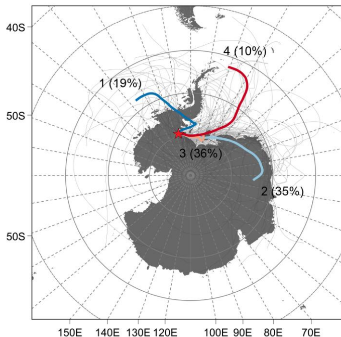
Figure 10: Cluster analysis of 5-day backward trajectories transporting air masses towards the UG region (red star) as calculated for all days with precipitation events (in total 121, represented by thin grey lines) for the period 2010-2015 using the model HYSPLIT. Bold lines represent main transport pathways calculated as percentage (%) of all trajectories associated with the respective cluster.
