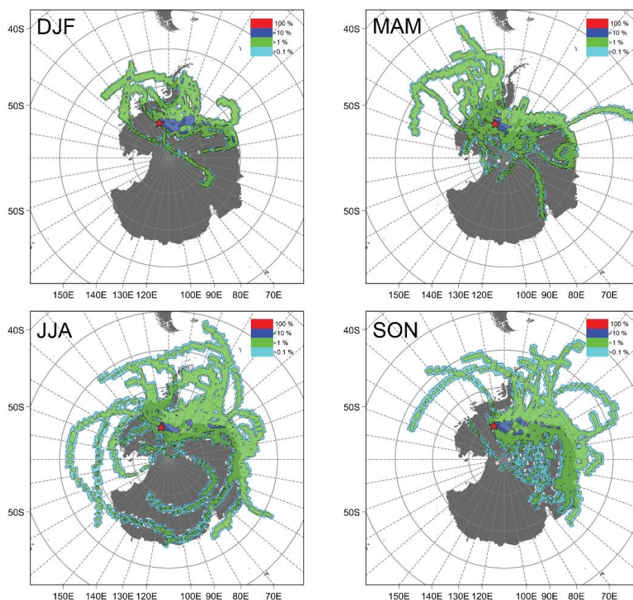
Figure 11: Seasonal frequency distribution of single 5-day backward trajectories during precipitation events extracted from ERA-Interim time series of daily precipitation for the UG region (red star) for the period 2010-2015. In total 121 precipitation events with \geq 1\% of the mean annual snow accumulation ( \sim 2.5 \text{ mm d}^{-1} ) were considered for this analysis performed with the
