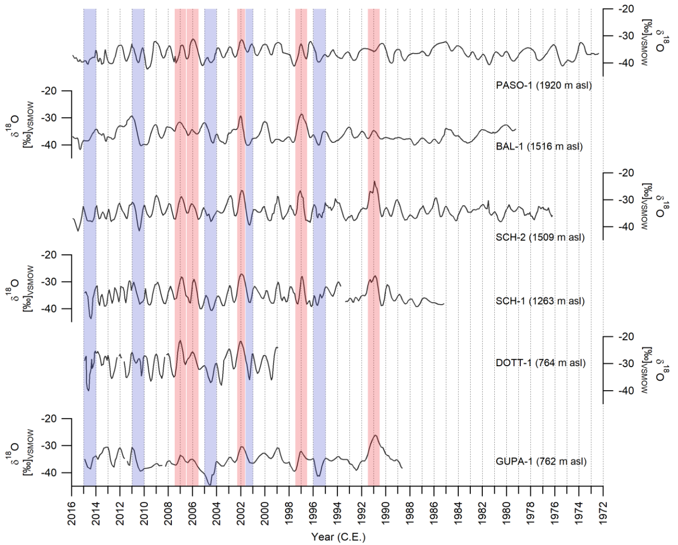
Figure 7: Profiles of the stable water isotope composition ( \delta^{18}\text{O} ) of the six firn cores from Union Glacier with respect to time. Years with prominent maxima and minima in \delta^{18}\text{O} -time series - although not visible in all cores - are highlighted by red and blue shading, respectively. The peak in summer 2002 is the only maximum found in all cores.
