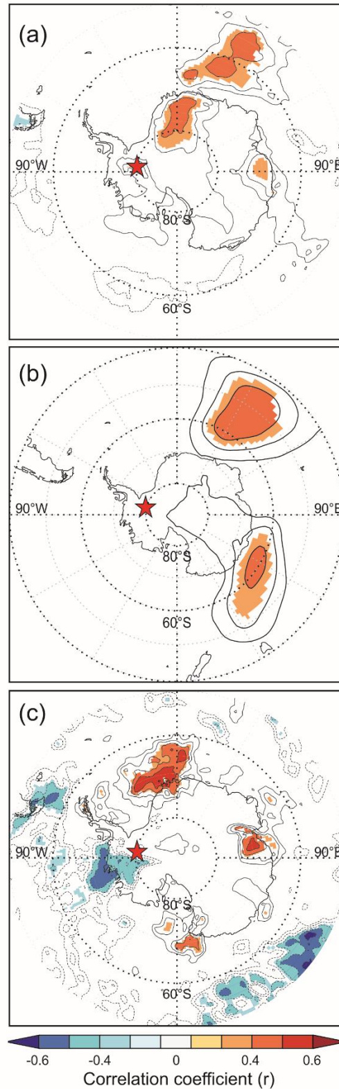
Figure 9a-c: Spatial correlation of annually averaged ERA-Interim (a) near-surface air temperatures (2 m), (b) geopotential heights (850 mbar) and (c) precipitation-evaporation with standardized mean annual (a) \delta^{18}\text{O} , (b) d excess and (c) snow accumulation in the UG region for the period 1980-2014 (excluding firn core GUPA-1). All time series were detrended before calculating spatial correlations. The red star denotes the location of the UG region. Only statistically significant correlations ( p -value < 0.05 ) are displayed. For (a) and (c) December-November annual averages (calendar year) were used, whereas for (b) August-July annual averages (winter-winter) were considered as spatial correlations appear more significant than for December-November annual averages.
