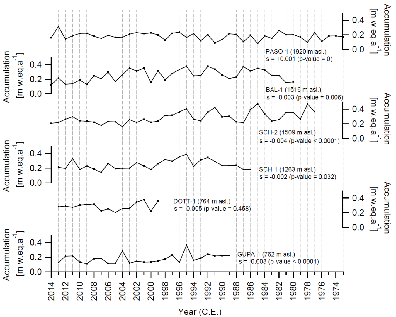
Figure 6: Annual accumulation rates at the drill sites of the six firn cores from Union Glacier for the period covered by the respective firn core. Sen slopes ( s in \text{m w.eq.a}^{-1} ) and p-values are given for all firn cores indicating that accumulation has decreased at most sites since the beginning of the record period.
