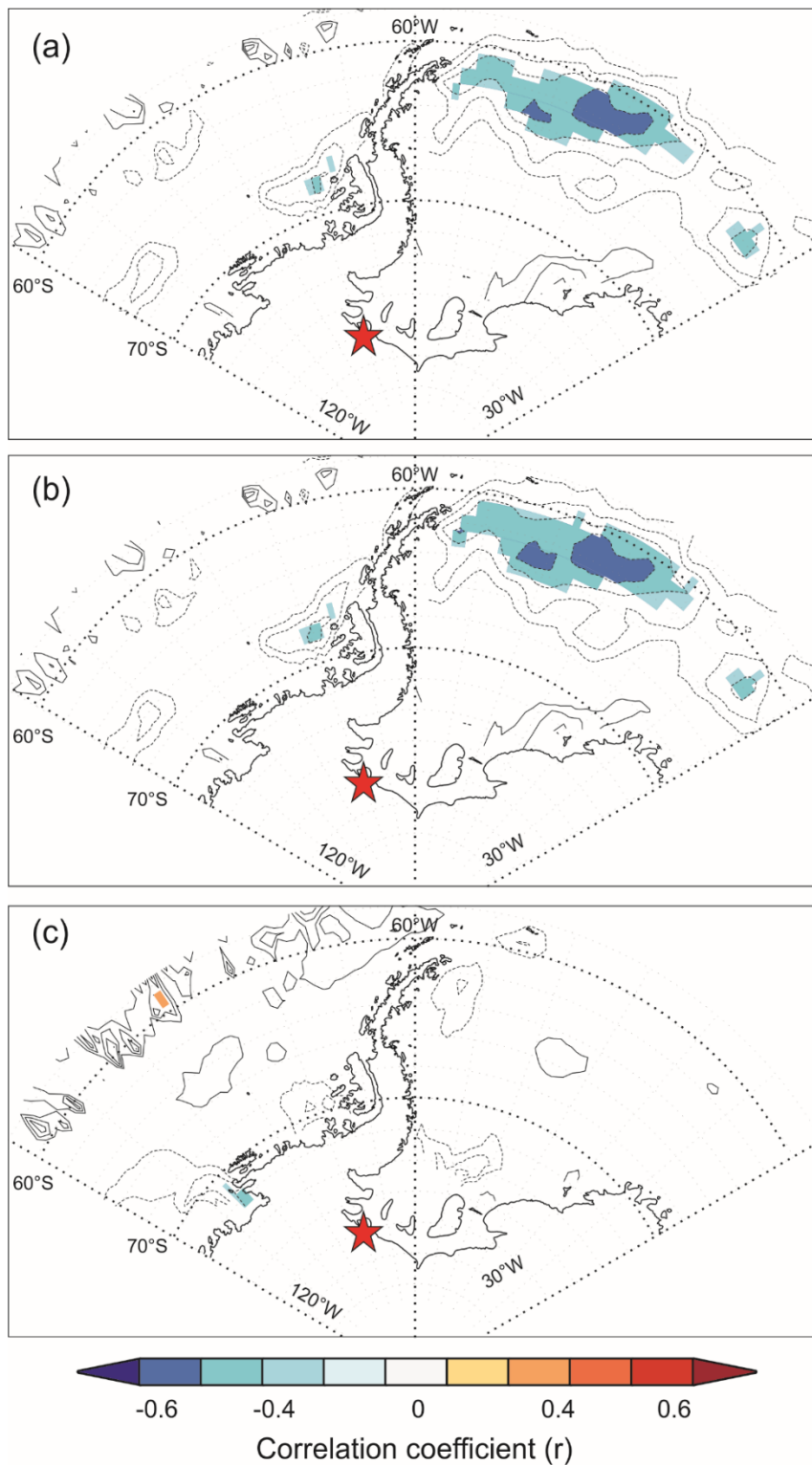
Figure 12a-c: Spatial correlations of standardized mean annual (a) \delta^{18}\text{O} , (b) d excess and (c) snow accumulation in the UG region with mean annual sea ice concentrations in the Weddell and Bellingshausen Sea sectors for the period 1980-2014 (excluding firn core GUPA-1). For the calculations all time series were detrended and December-November annual averages (calendar year) were considered. The red star denotes the location of the UG region. Only statistically significant correlations ( p -value < 0.05) are shown.
