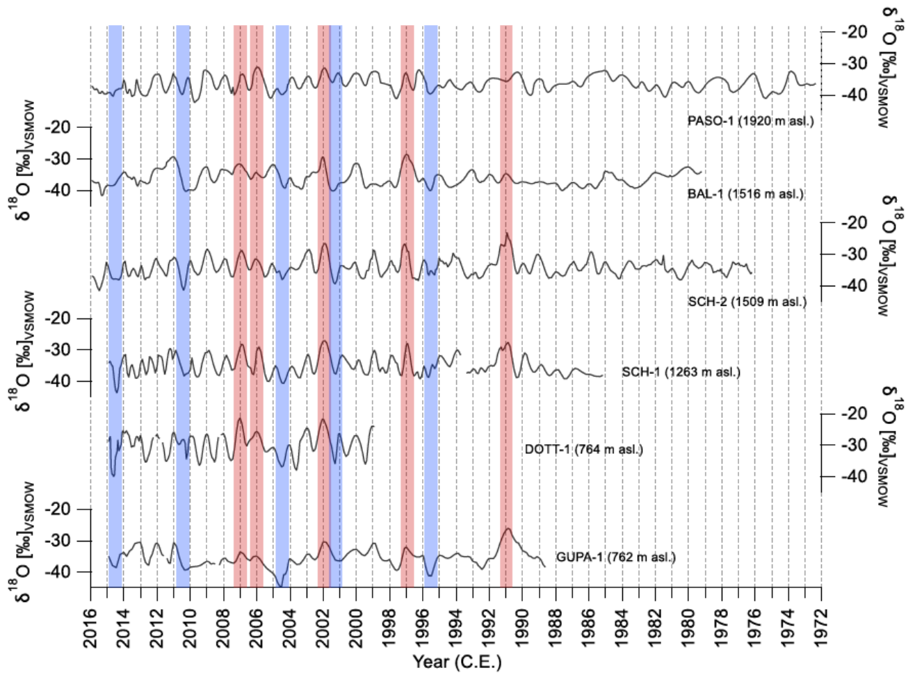
Figure 7: Profiles of the stable water isotope composition ( \delta^{18}\text{O} ) of the six firn cores from Union Glacier with respect to time. Years with prominent maxima and minima in \delta^{18}\text{O} -time series - although not visible in all cores - are highlighted by red and blue shading, respectively. The peak in summer 2002 is the only maximum found in all cores.
