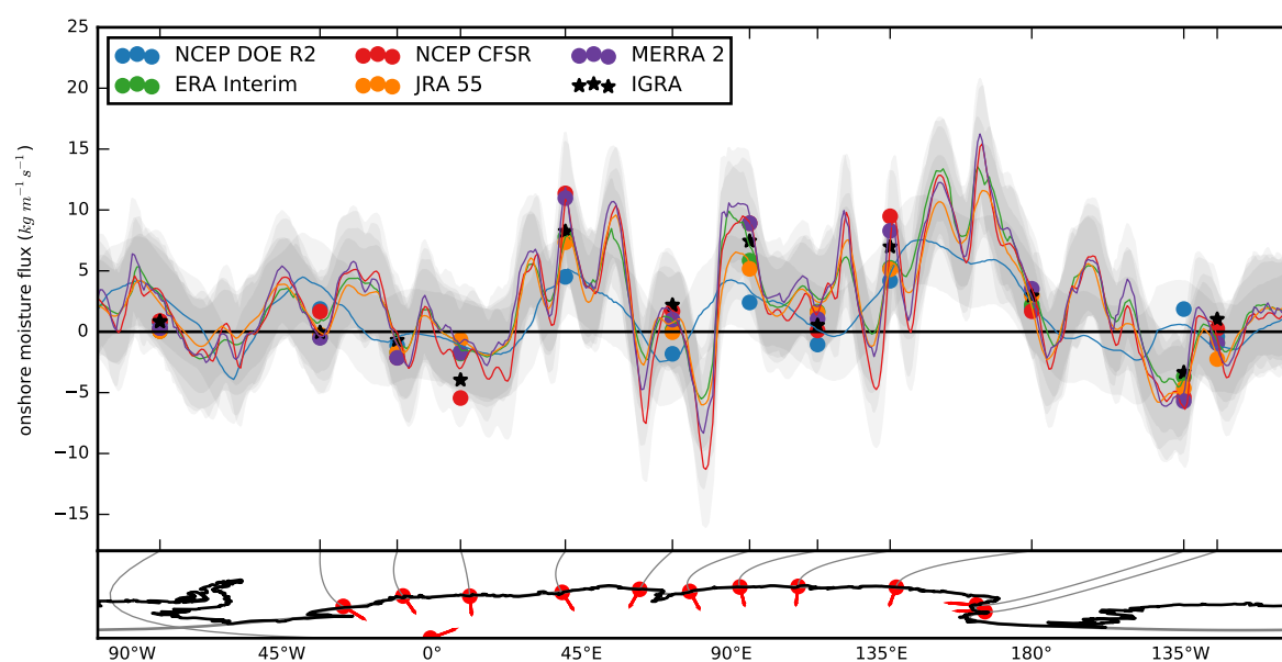
Figure 5. Distribution of the mean incoming vertically integrated moisture flux on the boundary of the Antarctic ice sheet in different reanalyses. The grey shaded bands indicate the ranges corresponding to plus or minus one interannual standard deviation from the mean. Stars represent the radiosonde and dots the reanalyses interpolated over the launch sites and with the same temporal sampling as the observations. The red dots in the lower panel indicate the location of the sites and the arrows the direction normal to the boundary.
