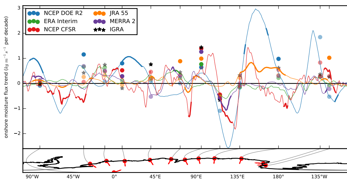
Figure 10. Linear trends of vertically integrated moisture transport into East Antarctica. The profiles are built from reanalyses over the 1980-2016 period interpolated along the domain boundary whereas the dots are computed from reanalyses with the same temporal sampling as the observations. The stars correspond to trends computed from observations. The bold sections of the profiles and the solid dots and stars indicate statistically significant changes.
