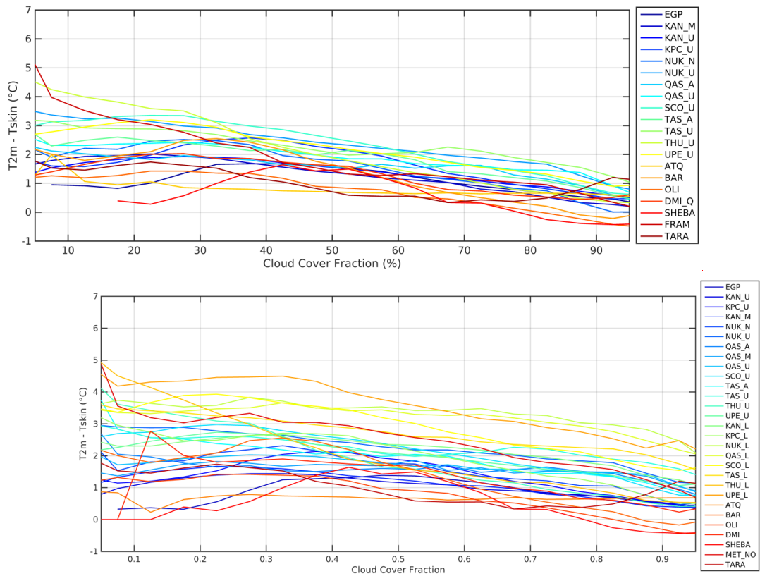
Figure 103: 2 m air temperature and skin temperature differences for all sites as a function of binned cloud cover fraction (CCF). The CCF bin size is 0.05, the T2m-Tskin bin size is 1°C, and only bins with more than 50 members are considered.
