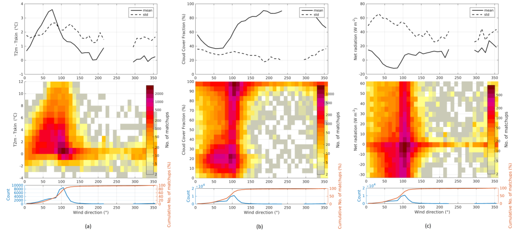
Figure 10: 2 m air temperature and T_{skin} difference (a), the cloud cover fraction (b), and the net radiation (c) as a function of binned wind direction for THU-U. The upper figures show the standard deviation (dashed lines) and mean difference (solid lines). The surface plots in the middle show the number of matchups in each bin, while the bottom plots show the number of matchups (blue lines) and the cumulative percentage of matchups (red lines) in each wind direction bin.
