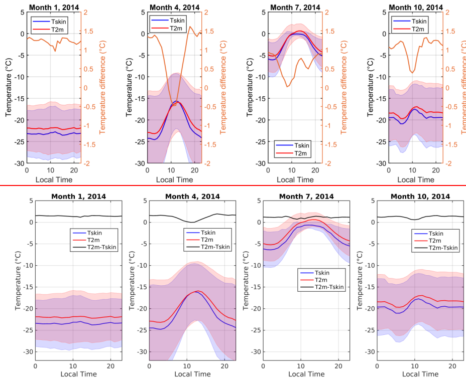
Figure 43: Monthly diurnal variability of 2 m air temperature (red) and skin temperature (blue) at KAN_U during the months: January, April, July and October. The black-orange curves are the difference between the red and blue curves. The shadings indicate the standard deviations.
