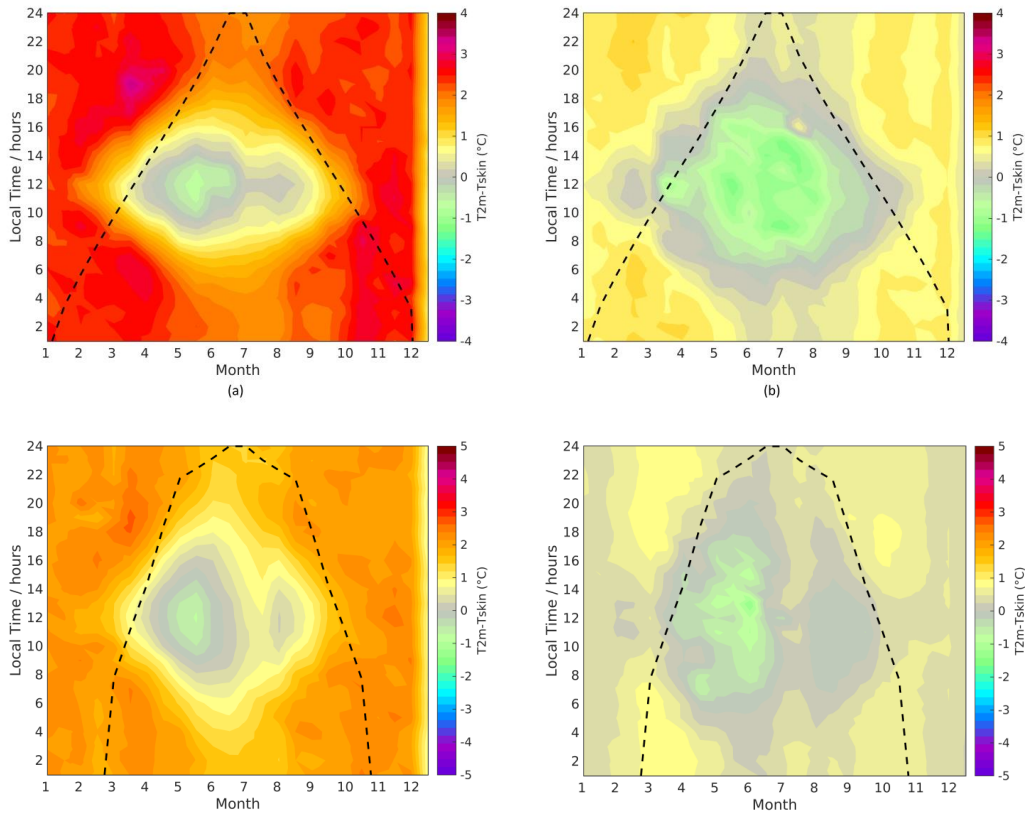
Figure 141: Similar to Fig. 7a but with 2 m air temperature and skin temperature differences for ACC sites at KAN-U in cases of clear-sky (a), and overcast conditions (b). The dotted black lines indicate the total hours of sunlight each month.
