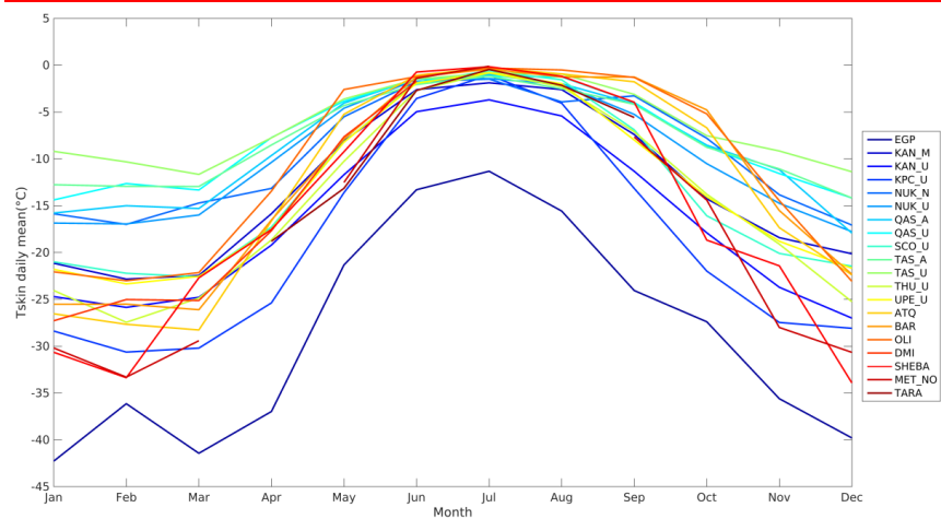
Figure 54: Monthly mean of T_{skin} (a), skin temperature daily range in T_{skin} (b) and T2m - T_{skin} difference (c), for all sites. See Table 1 for station locations and types.
