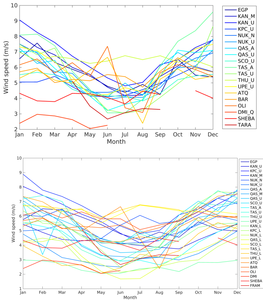
Figure 78: The average annual cycle in wind speed for all sites.
