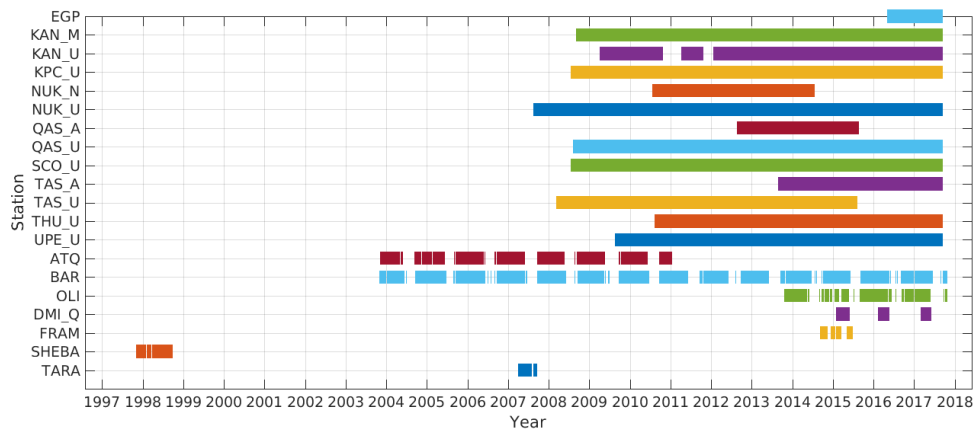
Figure 24: Temporal coverage for each data observation site included in this study.
