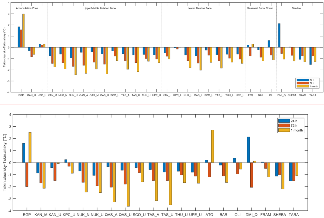
Figure 152: Observed clear-sky biases ( T_{\text{skin\_clearsky}} - T_{\text{skin\_allsky}} ) averaged for different time intervals, for all sites ( ^{\circ}\text{C} ).
