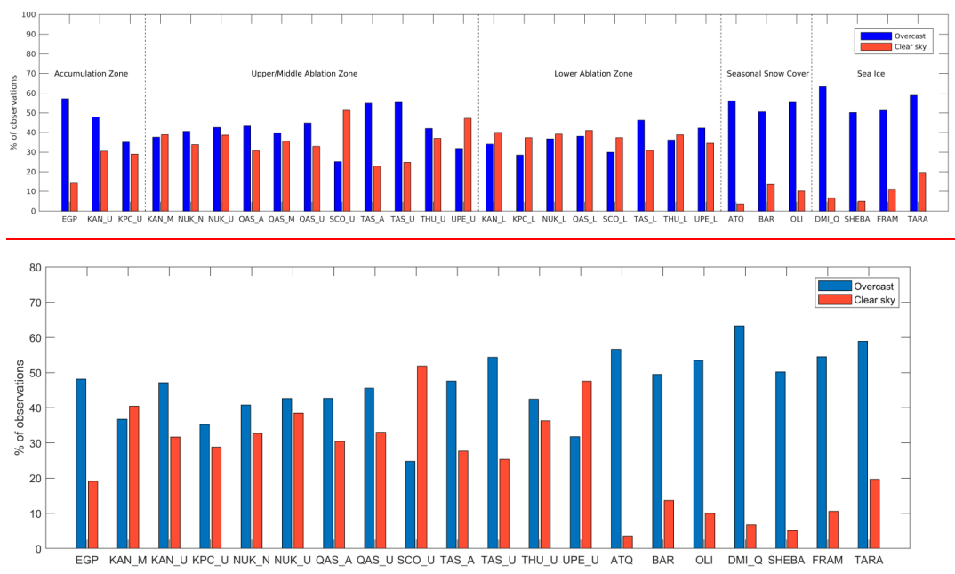
Figure 944: Frequency of clear-sky and overcast observations in percent of all observations for each site.
