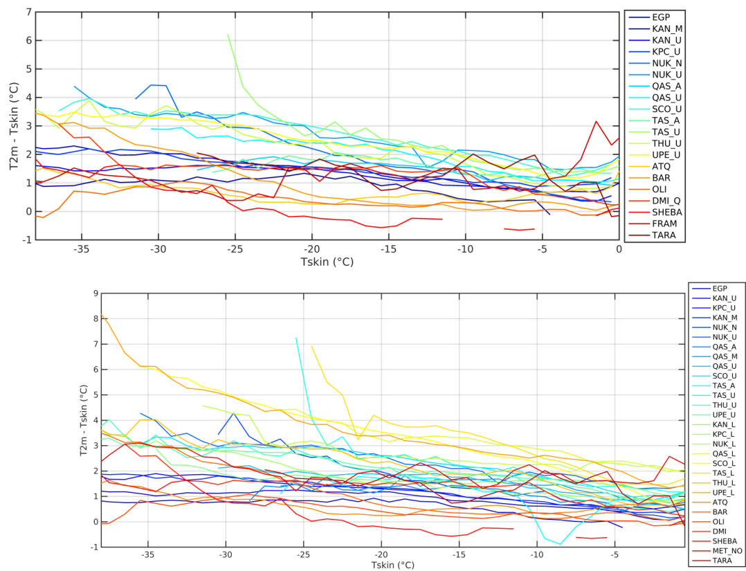
Figure 147: Mean 2 m air temperature and skin temperature differences for all sites as a function of binned skin temperature. The T_{skin} bin size is 1°C, the T_{2m}-T_{skin} bin size is 1°C, and only bins with more than 50 members are considered.
