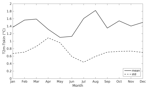
Figure 6: Monthly mean difference in 2-m air temperature and skin temperature ( T_{2m}-T_{skin} ) for all data-sites with time coverage as listed in Table 1 (solid line). The dashed line shows the mean of the standard deviations from the different observation sites.
