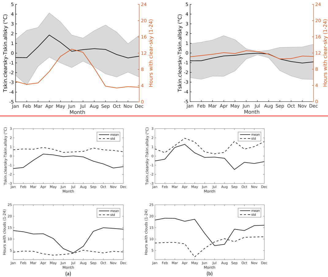
Figure 136: The top panels show the differences between 24 h averaged clear-sky and all-sky skin temperatures for PROMICE ACC stations (a) and SEAICE+LAB stations (b) for each month. The solid lines are the mean clear-sky bias while the dashed lines are standard deviations. The red lines show the 24 h averaged number of hours with CCF > 0.770% per day for each month.
