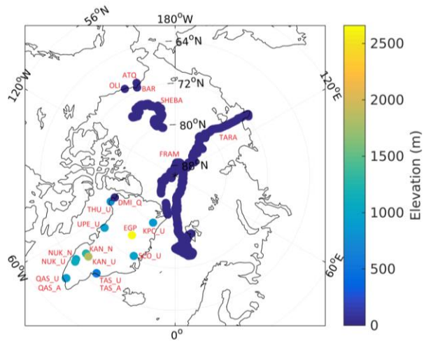
Figure 12: Spatial coverage and elevation for each site included in this study. The colour bar is elevation in meters.
