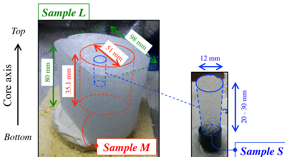
Figure 2. Schematic of the different sample sizes used in this work. Sample characteristics are listed in Table 2. In green, large samples L of the firm core were characterized by X-ray tomography using a voxel side length of 60\ \mu\text{m} . Zooming inside the L samples enables to obtain medium sized samples (typical of the size used in pycnometry measurements) named M and shown in red. These were scanned at 30\ \mu\text{m} (DC-M30). More than 40 samples (shown in blue) of size S were machined separately and scanned at 12\ \mu\text{m} for both sites (samples DC-S12 and LI-S12).
