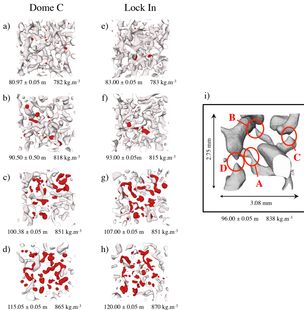
Figure 4. Evolution of closed pores (red) within the firm porosity network (grey) for different depths at Dome C and Lock In sites for DC-C12 and LI-C12 volumes (cross-section dimension is 6.72 \times 6.72 \text{ mm}^2 ). Note that (a-e), (b-f), (c-g) and (d-h) have approximately the same density. (i) Close-up view from a DC-C12 volume of a few channels between pores at different stages of the pinching process illustrated by areas A-B-C-D.
