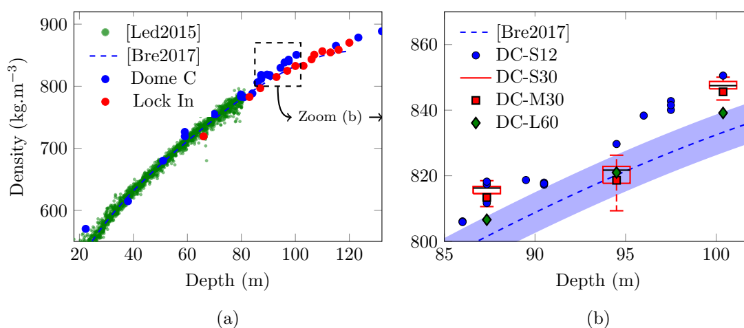
Figure 3. (a) Evolution of density with depth for Dome C and Lock In. (b) Zoom-in from (a) focused on Dome C for various ROI sizes (S, M, L) and voxel sizes (12, 30 and 60 \mu\text{m} ). Boxplots contain data from DC-S30 volumes. Hereafter, boxes represent lower and upper quartiles, the black lines inside being the median values. The confidence interval is set to account for all the data (no outliers). Green dots [Led2015] on (a) are data obtained by Leduc-Leballeur et al. (2015) from volume and mass measurements of 5 cm thick samples from a Dome C ice core down to 80 m. The blue dashed line [Bre2017] corresponds to a mean density profile of Dome C averaged on a 25 cm scale from Bréant et al. (2017). The blue shaded area on (b) represents a standard deviation of 6.2 \text{ kg.m}^{-3} between the fit and density data as given by Bréant et al. (2017).
