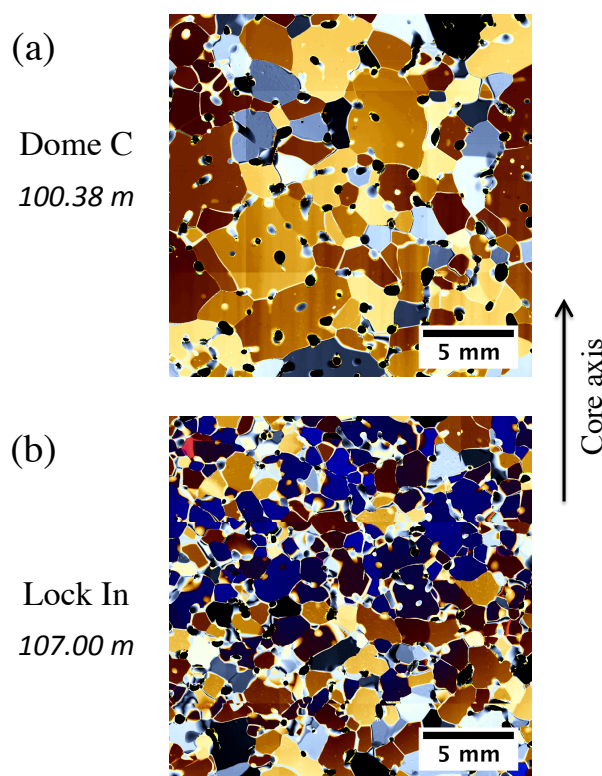
Figure 11. Comparison for the same density ( \rho = 851 \text{ kg}\cdot\text{m}^{-3} ) of (a) Dome C and (b) Lock In microstructures as observed by polarized light. Both thin sections are taken parallel to the core axis.
