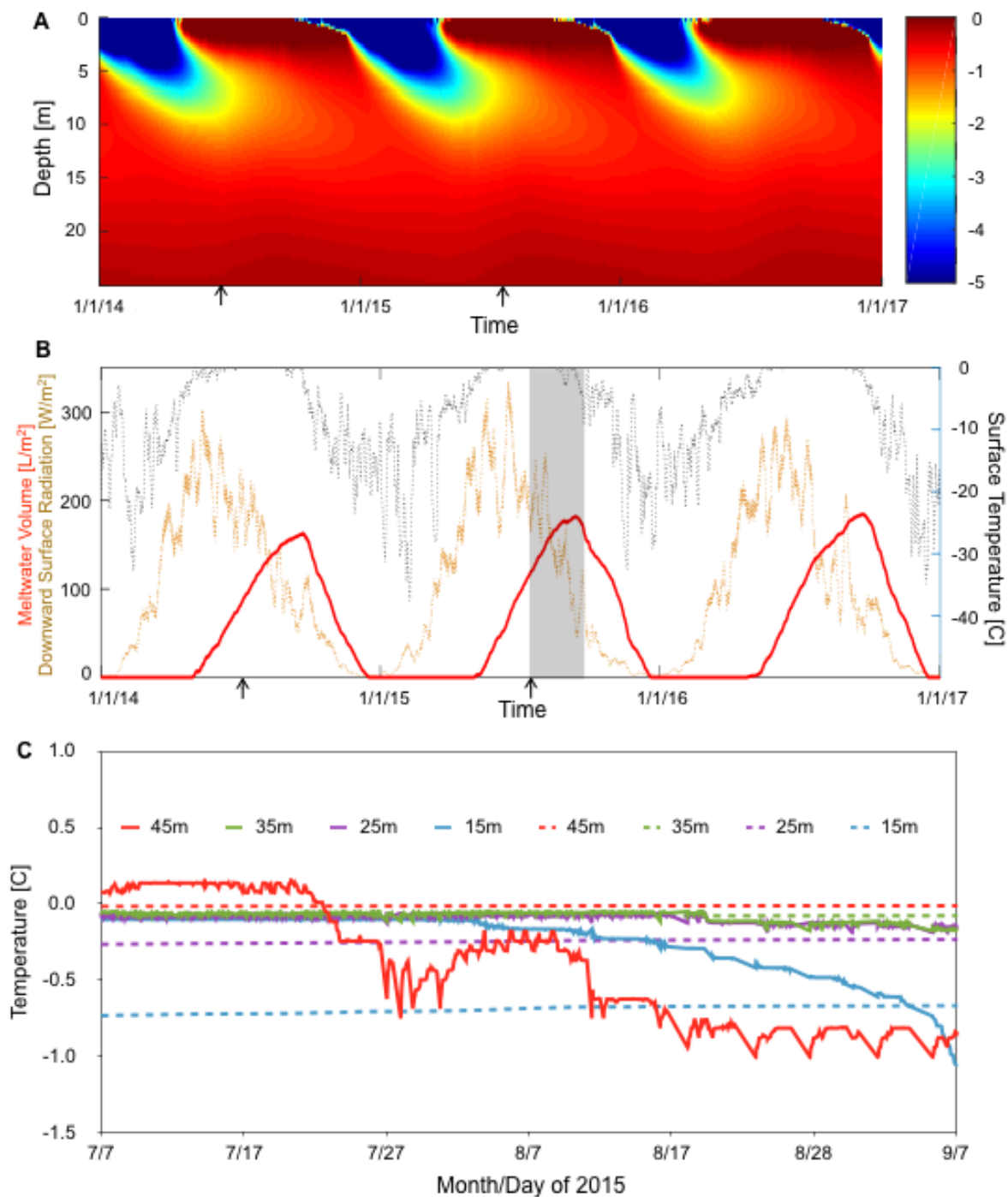
Figure 1. Temperature and ice water content during 2014 to 2016 (A) Modeled ice temperature was calculated using a finite
