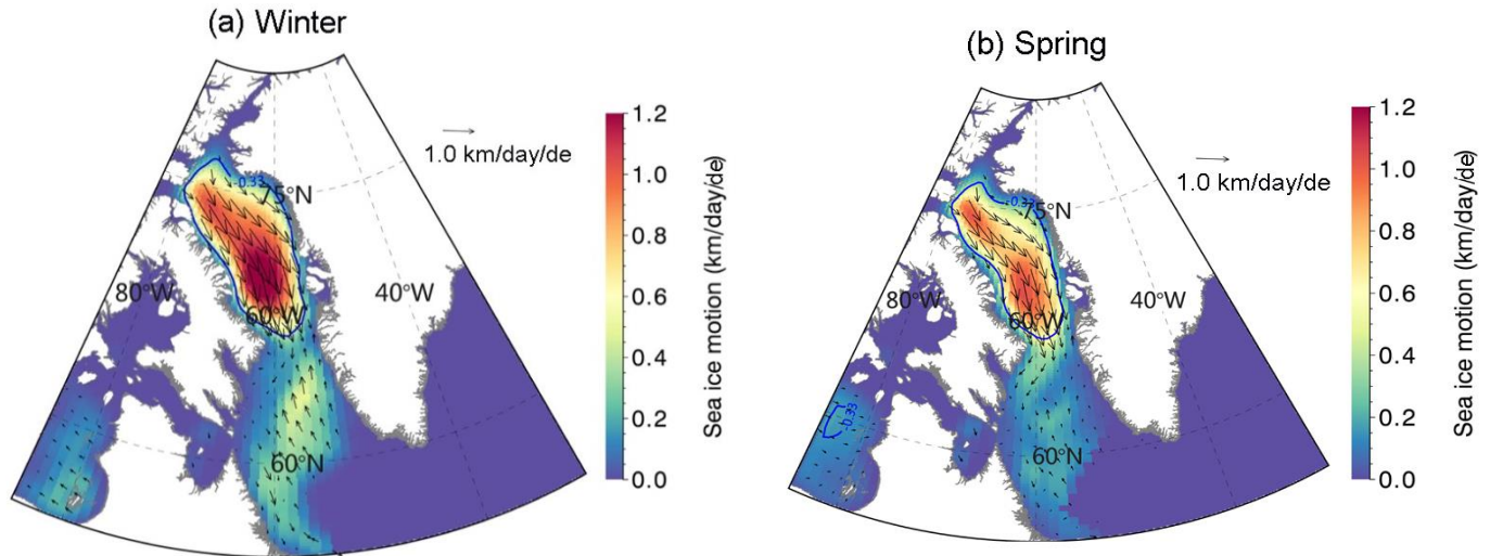
Figure 10. As Figure 8 but for sea ice motion fields.
