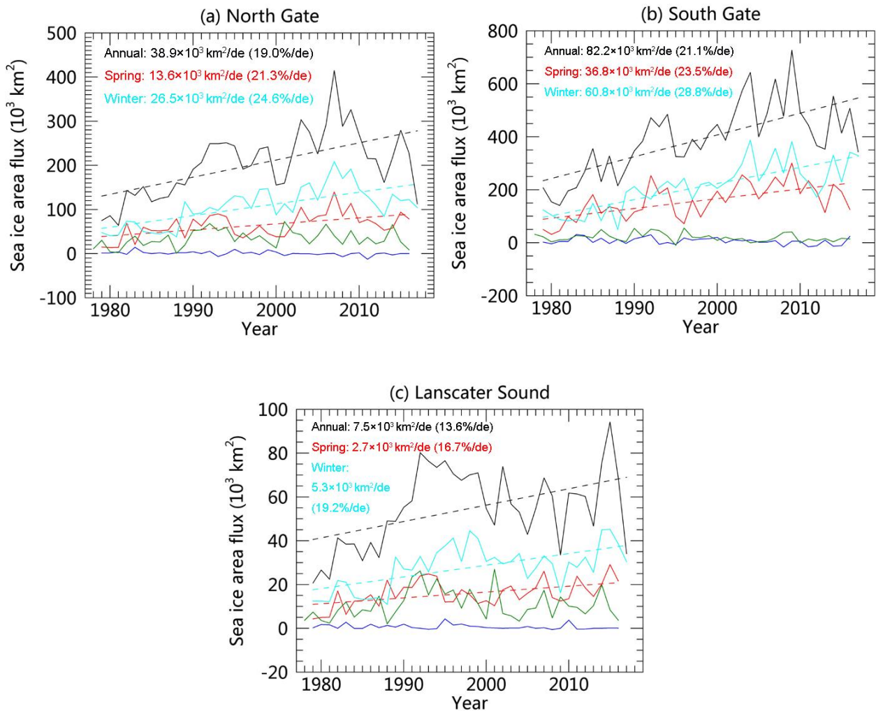
Figure 12. Time series of annual (September-August) sea ice area flux (black bold line) across (a) the North Gate, (b) the South Gate, and (c) Lancaster Sound. Seasonal flux is estimated for winter (December – February, cyan line), spring (March-May, red line), summer (June-August, green line), and autumn (September-November, blue line). The dashed lines represent the linearly fitted trends. The annual and cold-season (winter and spring) trends are all significant at the 99% level. However, for the warm seasons (summer and autumn), the trends are not statistically significant and are not shown in the panels.
