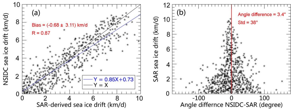
Figure 4. Comparison between NSIDC ice motion and Envisat SAR estimates in terms of (a) drifting speed and (b) angular direction.
