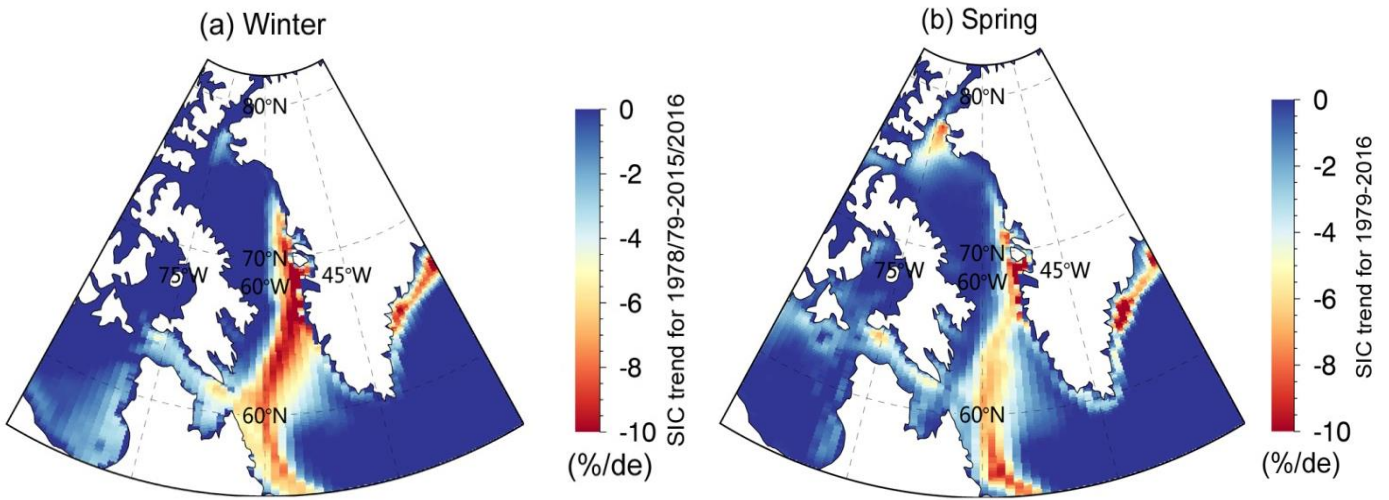
Figure 9. Sea ice concentration trends during (a) winter and (b) spring over the period 1978/1979-2016/2017.
