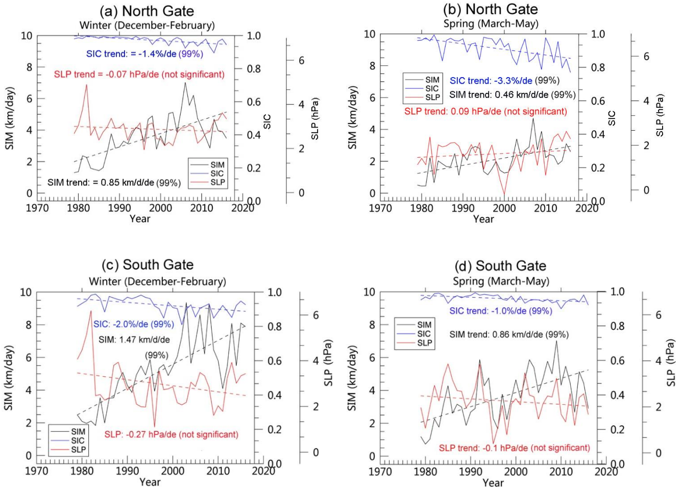
Figure 15. Trends and variability of cross-gate mean sea ice motion (black bold line) and concentration (blue bold line) for the (a-b) North Gate and (c-d) South Gate. The linear fit line for each parameter is shown as a dashed line. Cross-gate sea level pressure (SLP) difference (red) is shown to facilitate the analysis of causes of the significant trends in sea ice motion.
