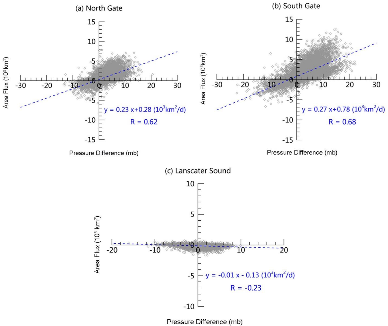
Figure 14. Scatterplot of daily sea ice area flux and cross-gate pressure differences for (a) the North Gate, (b) the South Gate, and (c) Lancaster Sound.
