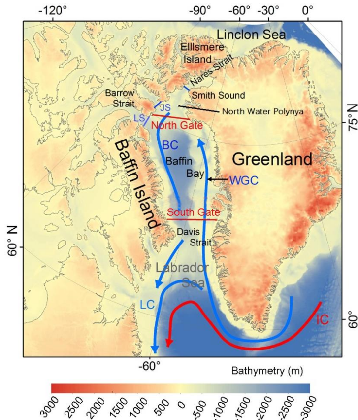
15 Figure 1. The mean circulation pattern in Baffin Bay (blue and red arrows) and the locations of the key fluxgates to assess sea ice area flux through the bay. The west Greenland current (WGC), Baffin Current (BC), and Labrador Current (LC) are marked with blue arrows. The Irminger Current (IC) is represented by the red arrow. The key fluxgates through which sea ice floats into the bay includes Nares Strait, Jones Sound (JS), and Lancaster Sound (LS). Area flux through a defined North
