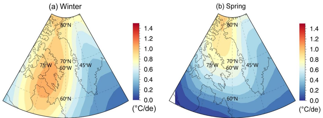
Figure 17. Surface air temperature trends for the period 1978/1979-2016/2017 during (a) winter and (b) spring periods
