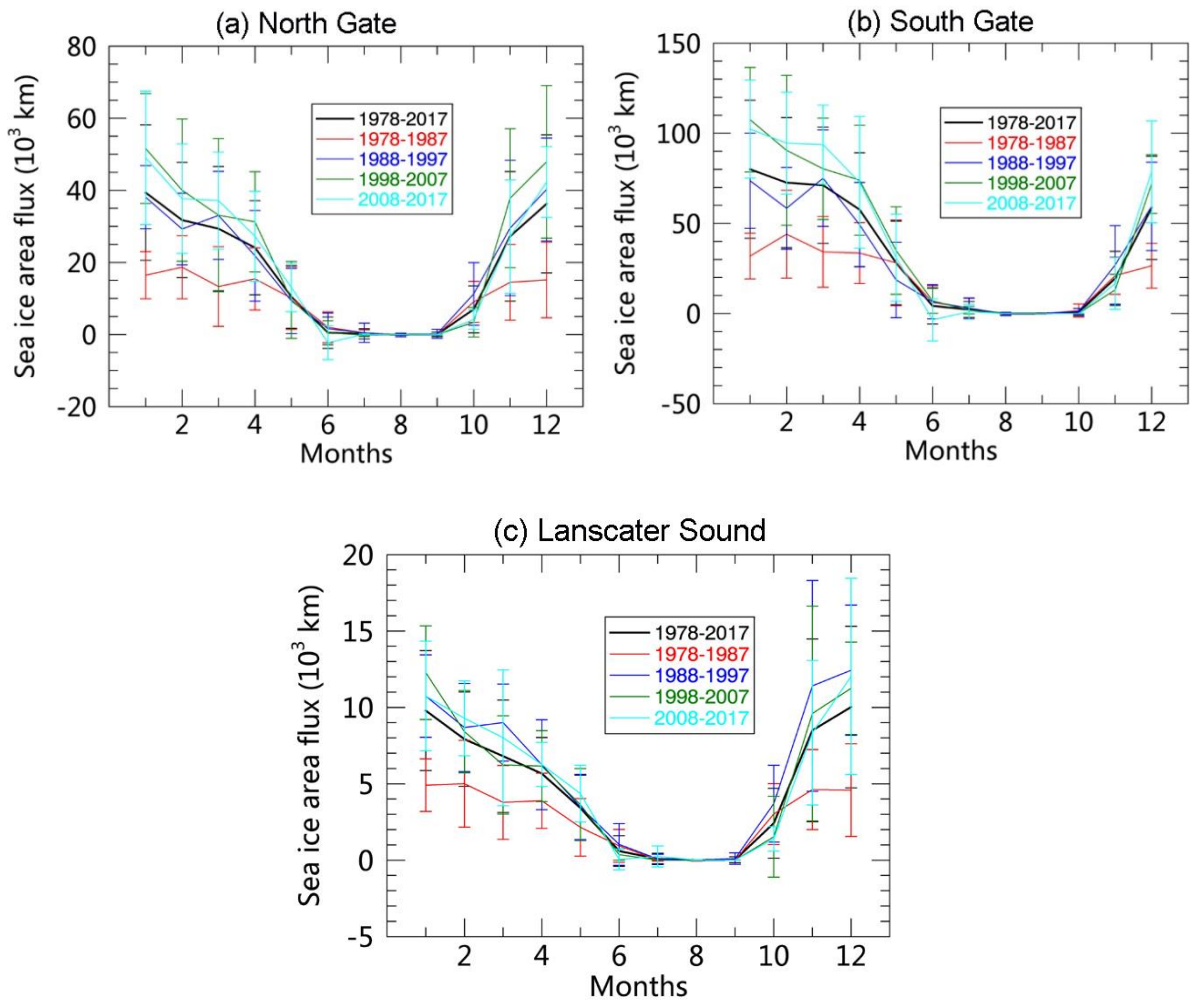
Figure 11. Monthly mean sea ice area export in (a) the North Gate, (b) the South Gate, and (c) Lancaster Sound. Both the climatology (1978/1979-2016/2017) and decadal mean fields are given in the panels.
