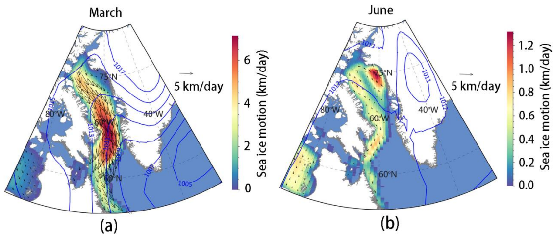
Figure 8. Sea ice drift patterns (arrows) in (a) March and (b) June 2016. Background color denotes the magnitudes of sea ice speeds. Superimposed bold curves represent the SLP distribution patterns of the corresponding month.
