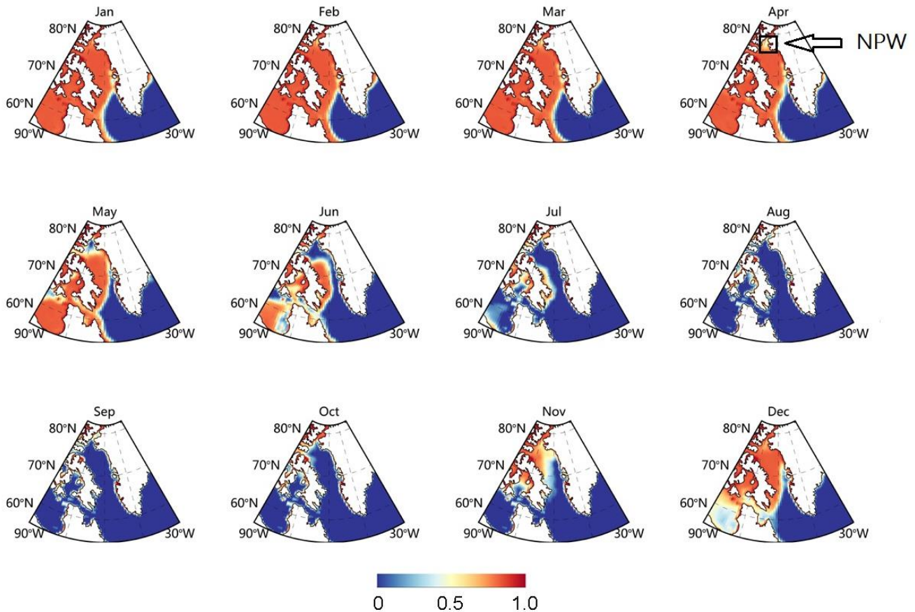
Figure 7. Spatial variations of mean sea ice concentration fields for the calendar months in 2016. In the panel for April, NPW is outlined.
