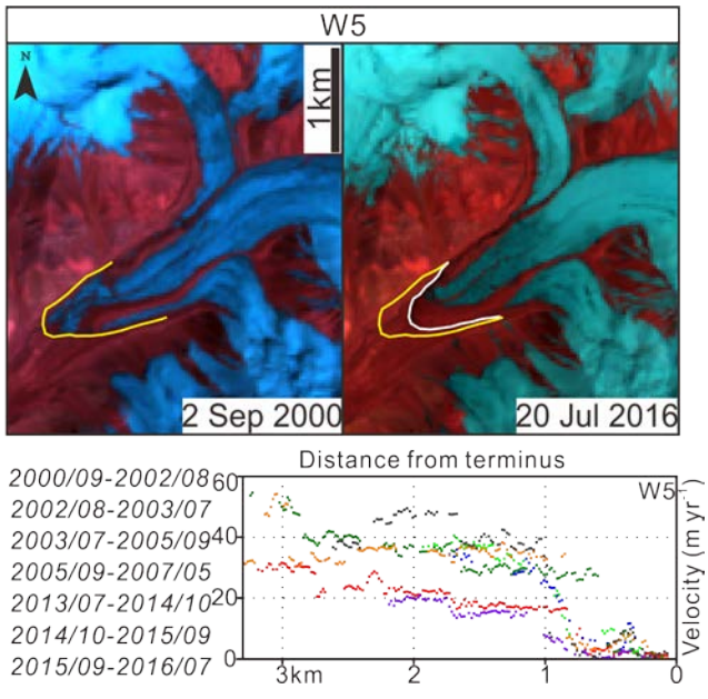
Figure 9: Comparison of W5 between 2000 and 2016 and its centreline annual-velocity profiles. The yellow line indicates its terminus position in 2000 and the white line indicates its terminus position in 2016.
