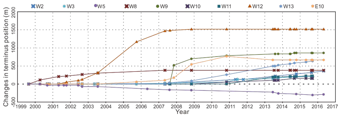
5 Figure 3: Changes in glacier terminus positions from 1999 to 2016 for 10 glaciers with detectable change.
