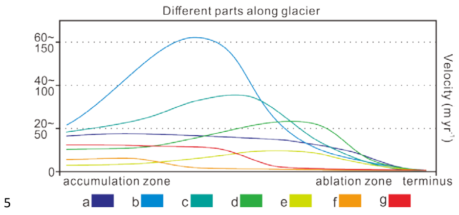
Figure 10: Conceptual characterisation of the glacial motion pattern of surge-type glaciers in the Kingata Mountains. Profile-a to Profile-g indicate different stages during the active and quiescent phases of a surge-type glacier.
