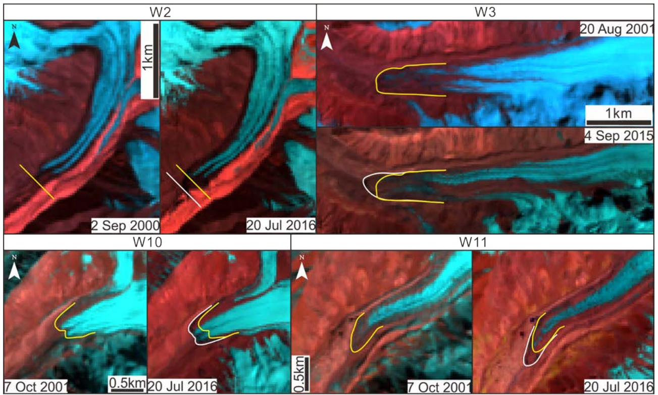
Figure 4: Comparison of the advancing glaciers before and after an advance. The yellow lines show the positions of glacier termini in early images and the white lines show the positions of the termini in recent images.
