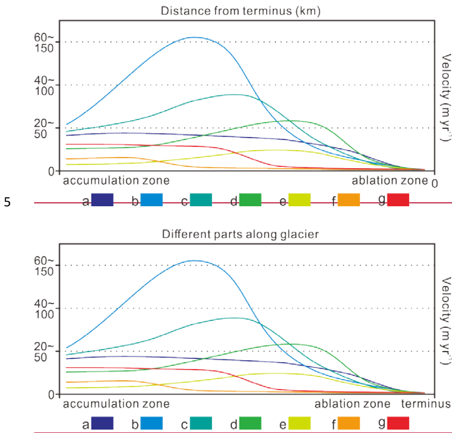
Figure 10: Conceptual characterisation of the glacial motion pattern of surge-type glaciers in the Kingata Mountains. Profile-a to Profile-g indicate different stages during the active and quiescent phases of a surge-type glacier.
