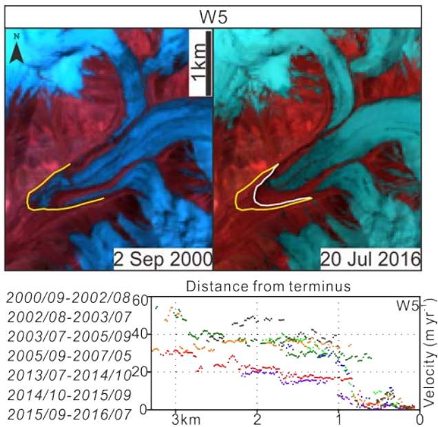
Figure 9: Comparison of W5 between 2000 and 2016 and its centreline annual-velocity profiles. The yellow line indicates its terminus position in 2000 and the white line indicates its terminus position in 2016.
