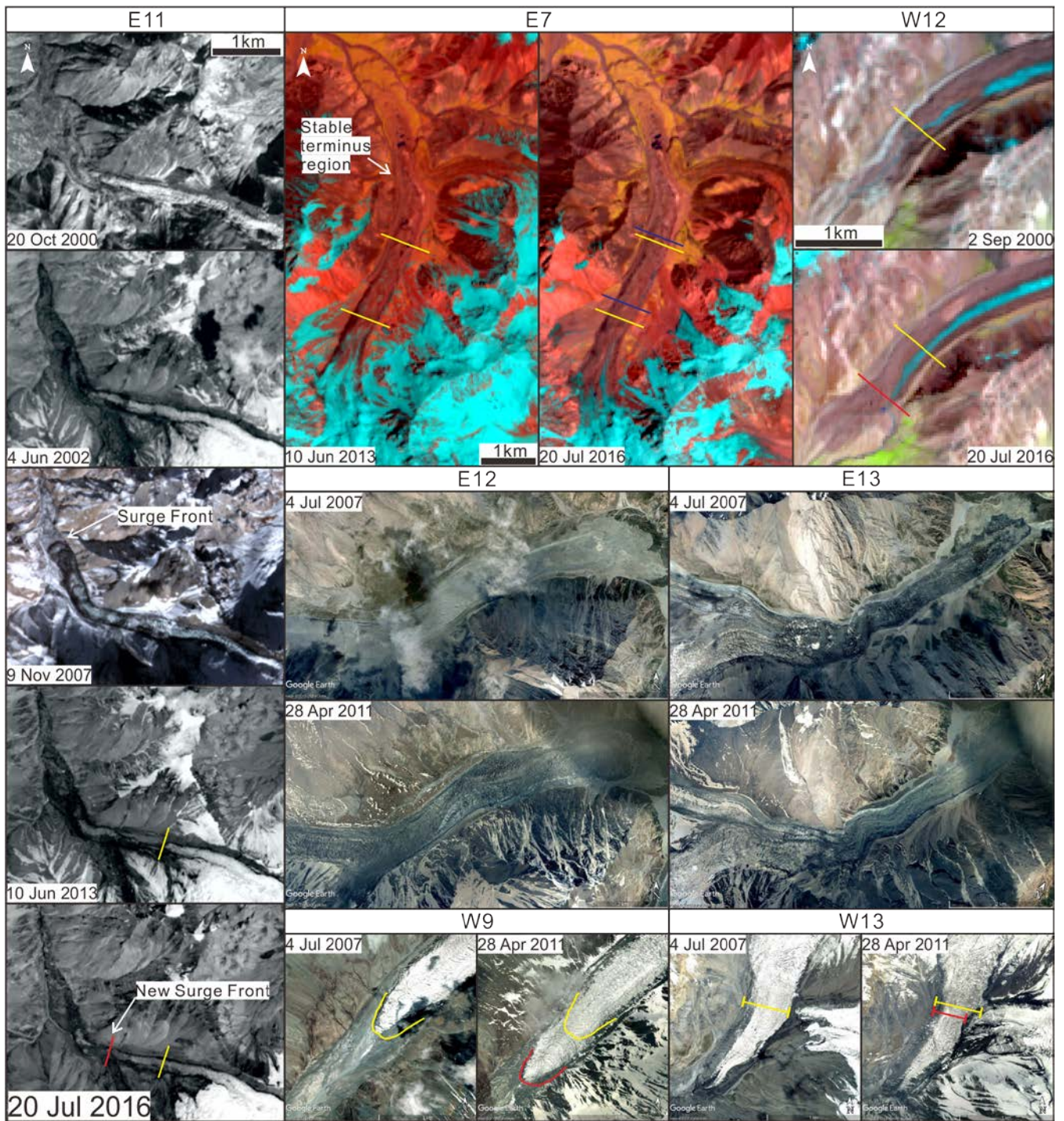
Figure 7: Comparison of the surge-type glaciers before and after surge events. The yellow lines show the positions of visible surface features in the earlier images and the red lines (blue lines for E7) show the positions of the same surface features in recent images. Note that the south branch of W13 surged into the trunk branch and narrowed the trunk branch to nearly two-thirds of its original width. E11 is given panels show the panchromatic band of Landsat, except for the middle panel which shows ASTER true colour combination in 2007.
