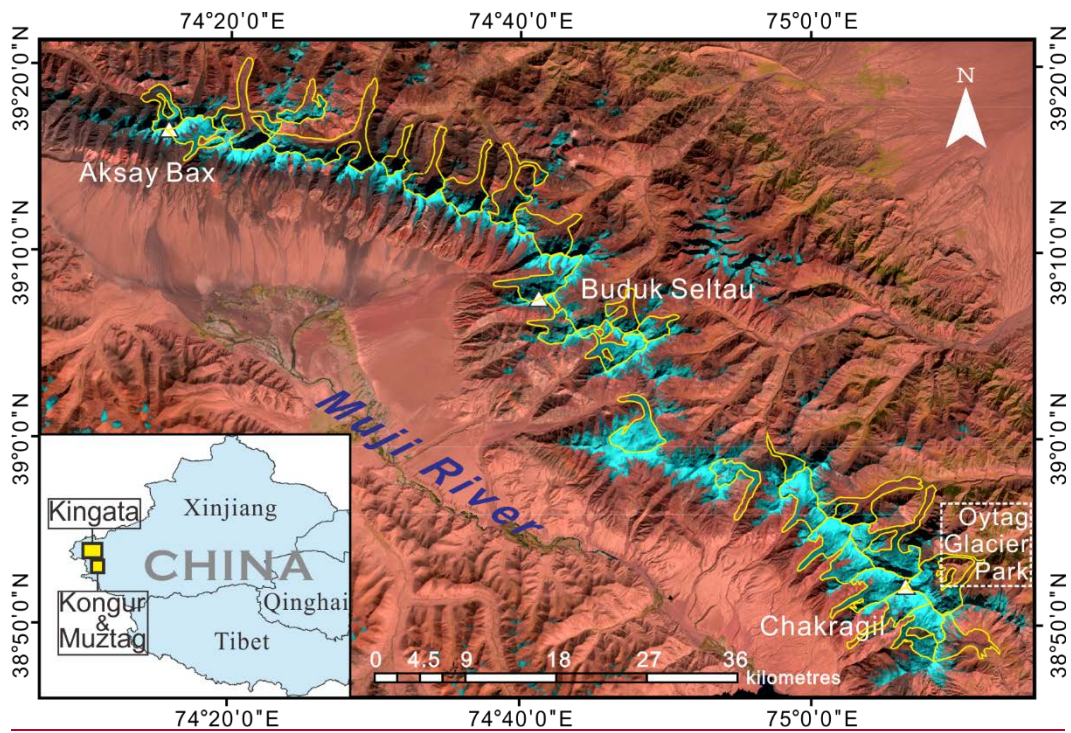
Figure 1: Landsat OLI image (bands 6-5-4) of the Kingata Mountains acquired on October 3rd, 2014. Light blue areas represent bare ice, red-brown areas represent bare soil and rocks, and green areas represent grass or other vegetation. Glaciers with area areas greater than 5 km 2 are highlighted by yellow lines.
