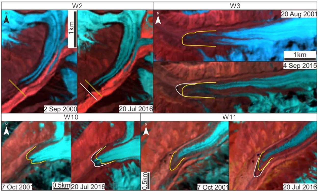
Figure 4: Comparison of the advancing glaciers before and after the sea level rise. The yellow lines show the positions of glacier termini in early images and the white lines show the positions of the termini in recent images.
