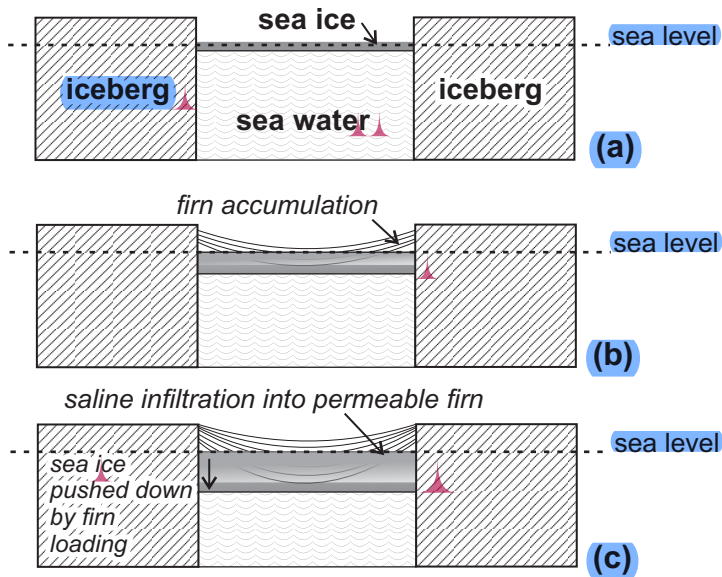
Figure 9: Cartoon to illustrate the process by which sea ice between icebergs becomes loaded by firn accumulation and driven below sea level by hydrostatic adjustment, allowing sea water to soak into the porous and permeable firn from below.
