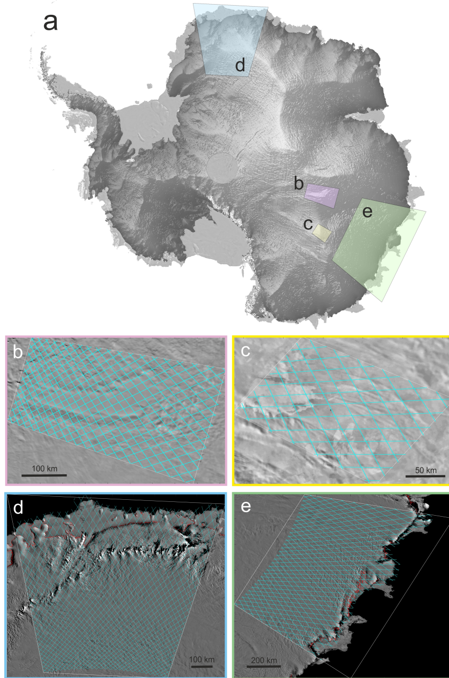
Figure 1. a. Overview of the Lake Vostok (b), Dome C (c), Dronning Maud Land (d) and Wilkes Land (e) study sites. The background image in panel a is a surface DEM from CryoSat-2 ( Slater et al., 2018 ) overlaid upon the MODIS Mosaic of Antarctica (MOA) ( Haran et al., 2006 ). Panels b-e show the Sentinel-3 ground tracks (cyan) at each study site, overlaid upon MOA.
