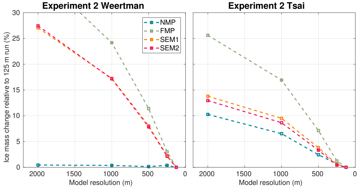
Figure 8. Convergence of ice volume above flotation at the end of Experiment 2 as a function of mesh resolution and Absolute error relative to the corresponding 125 mesh resolution results (same friction law and melt parameterization scheme) for the Weertman (a) and Tsai (b) friction laws for the NMP (blue), FMP (redgreen), SEM1 (yelloworange), and SEM2 (purplered) sub-element melt parameterizations.
