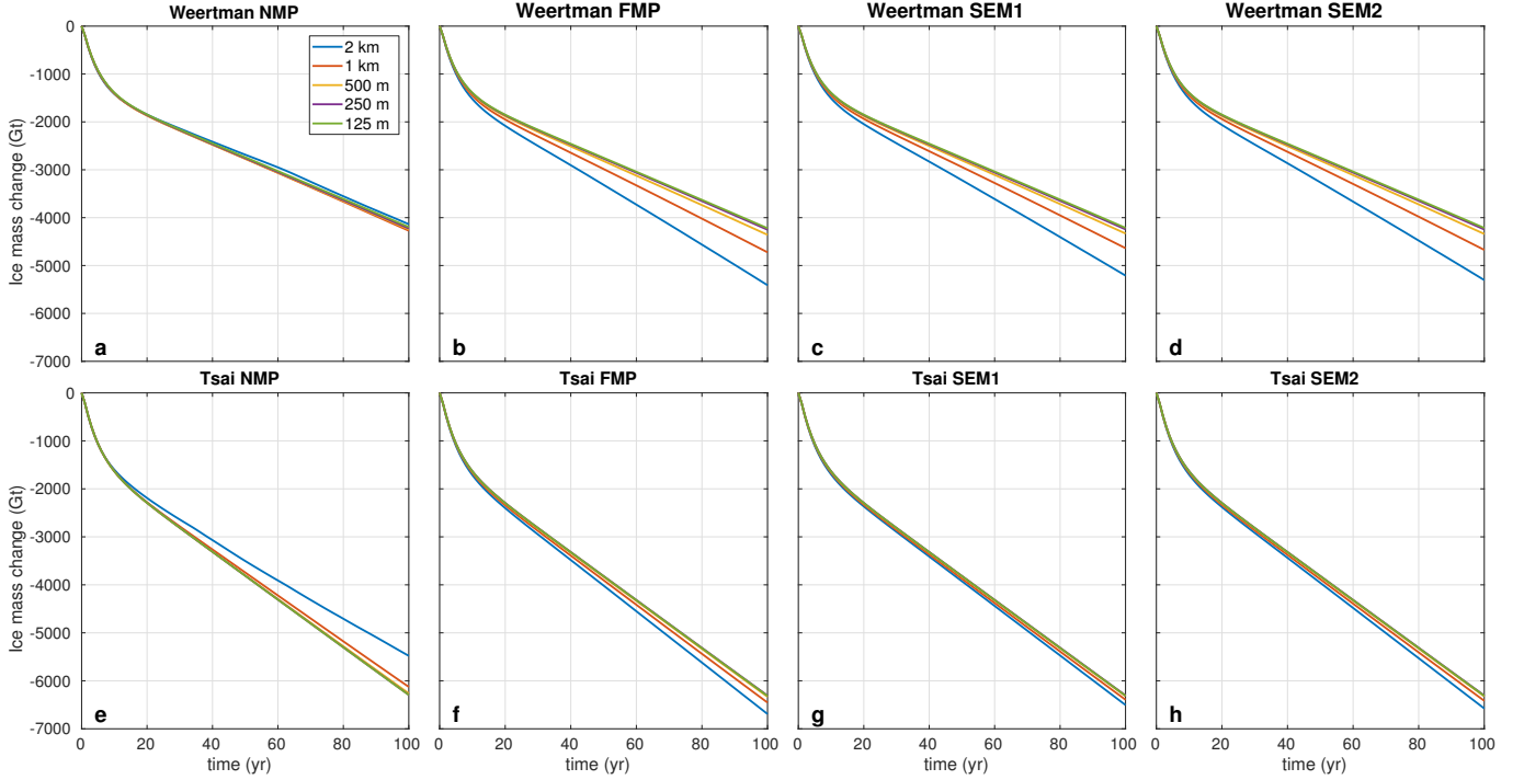
Figure 5. Evolution of ice volume above flotation in Experiment 1 for the NMP (a and e), FMP (b and f), SEM1 (c and g), and SEM2 (d and h), for the Weertman (a-d) and Tsai (f-h) friction laws. Each plot represents the evolution for the 5 mesh resolutions: 2 km (blue), 1 km (red), 500 m (yellow), 250 m (purple), and 125 m (green).
