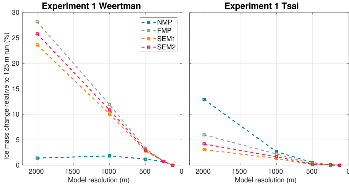
Figure 7. Convergence of ice volume above floatation at the end of Experiment 1 as a function of mesh resolution and Absolute error relative to the corresponding 125 mesh resolution results (same friction law and melt parameterization scheme) for the Weertman (a) and Tsai (b) friction laws for the NMP (blue), FMP (redgreen), SEM1 (yelloworange), and SEM2 (purplered) sub-element melt parameterizations.
