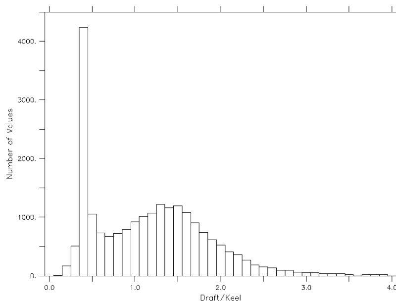
Figure 1. The histogram of the ULS measurement for the analysis of draft and keel (meters).
