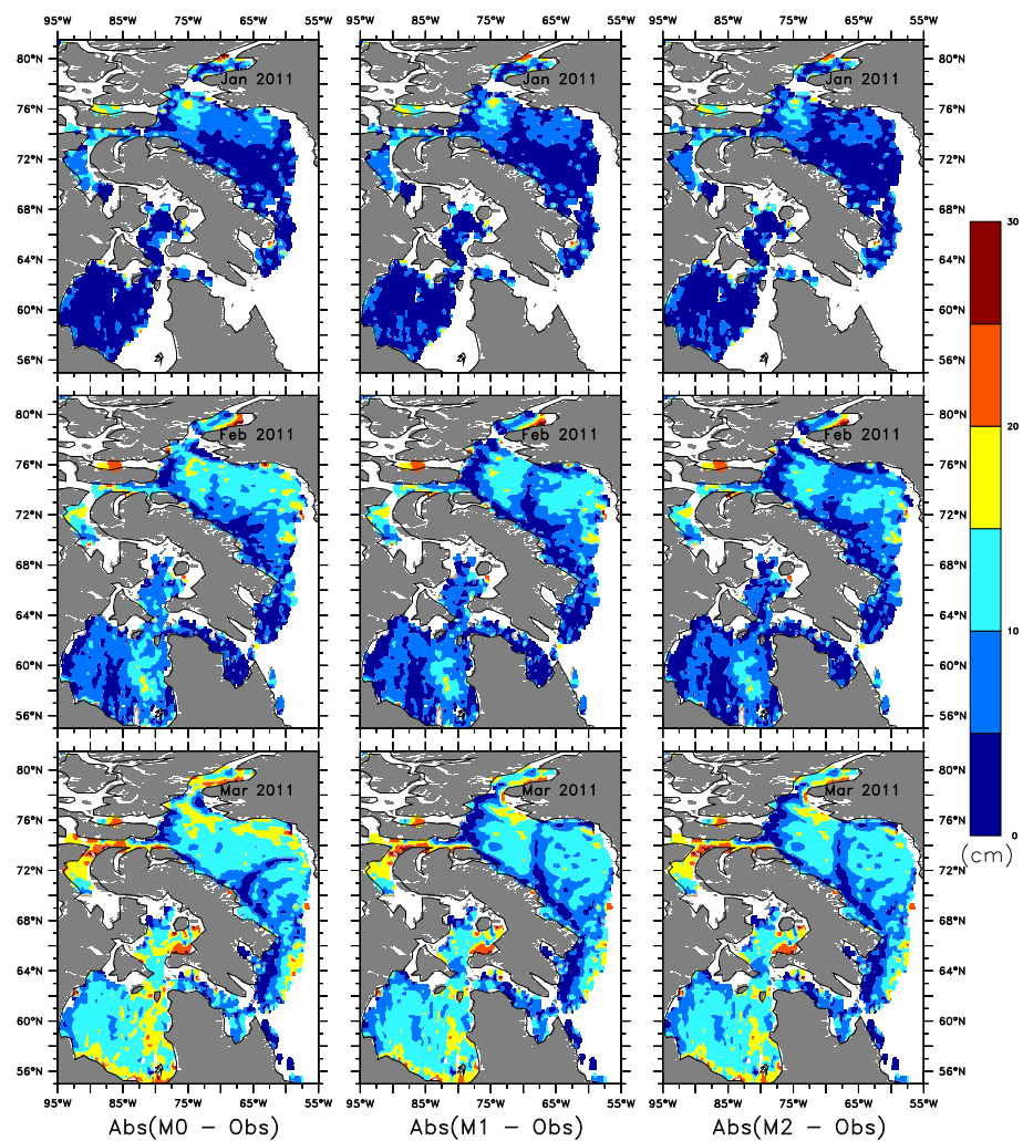
Figure 15. The absolute error between the model freeboard for M0, M1 and M2 and CryoSat-2 for January, February and March 2011.
