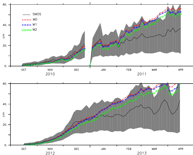
Figure 5. The ice thickness from the models M0, M1, M2, and observation (SMOS ice thickness) from October 2010 to April 2011 and October 2012 to April 2013 . The uncertainty of observation (SMOS ice thickness) is shaded in gray.
