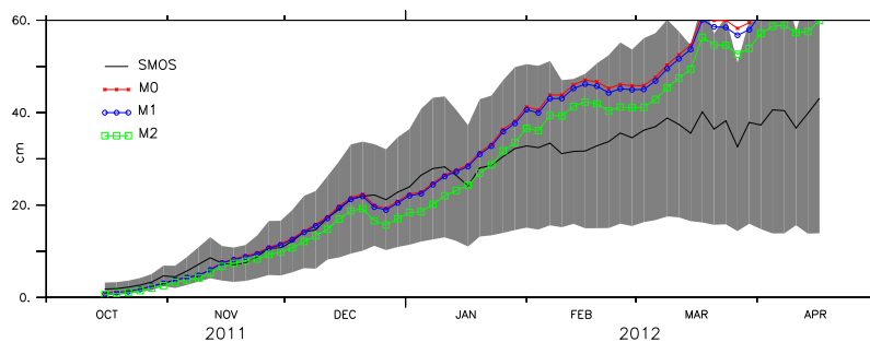
Figure 7. The ice thickness from models M0, M1(non assimilated but used the initial conditions from the model assimilated with ice concentration), M2 (assimilated only with SST and used model initial conditions derived from assimilating both ice concentration and SST) and observations (SMOS ice thickness) from October 2011 to April 2012. The uncertainty of observation (SMOS ice thickness) is shaded in gray.
