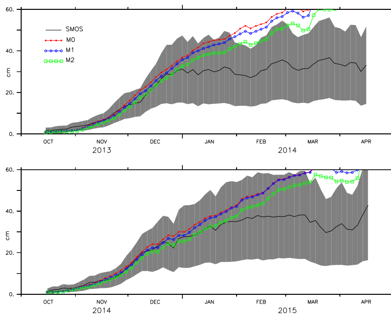
Figure 6. The ice thickness from the models M0, M1, M2, and observation (SMOS ice thickness) from October 2013 to April 2014 and October 2014 to April 2015. The uncertainty of observation (SMOS ice thickness) is shaded in gray.
