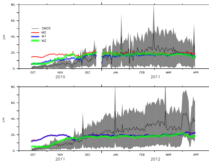
Figure 9. The model 'M2' estimated ice thickness, SMOS-MIRAS derived ice thickness, and the observation uncertainty for SMOS ice thickness less than 30 cm.
