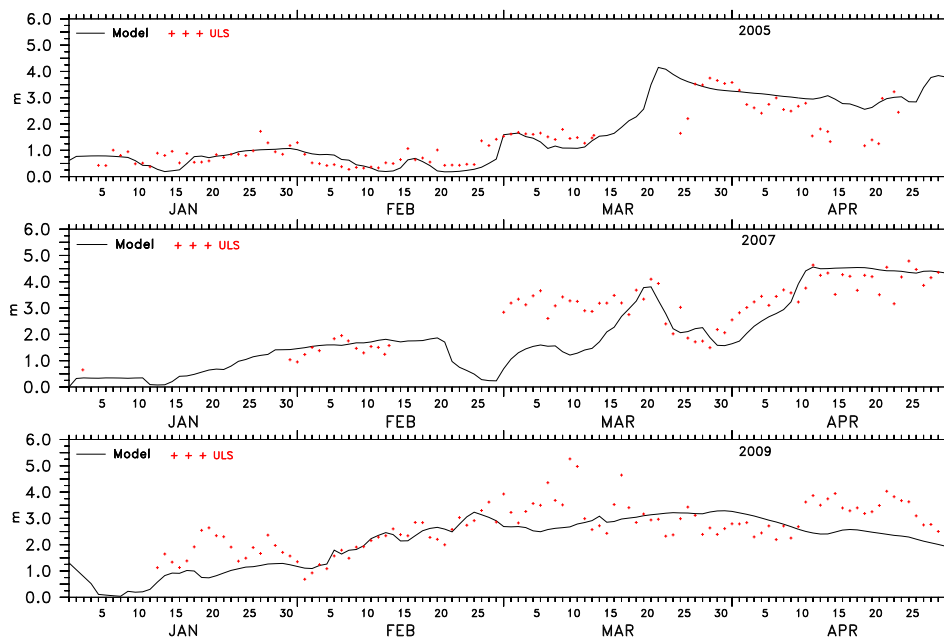
Figure 14. The keel depth computed from the ULS measurement and the model estimated values in cm for 2005, 2007 and 2009.
