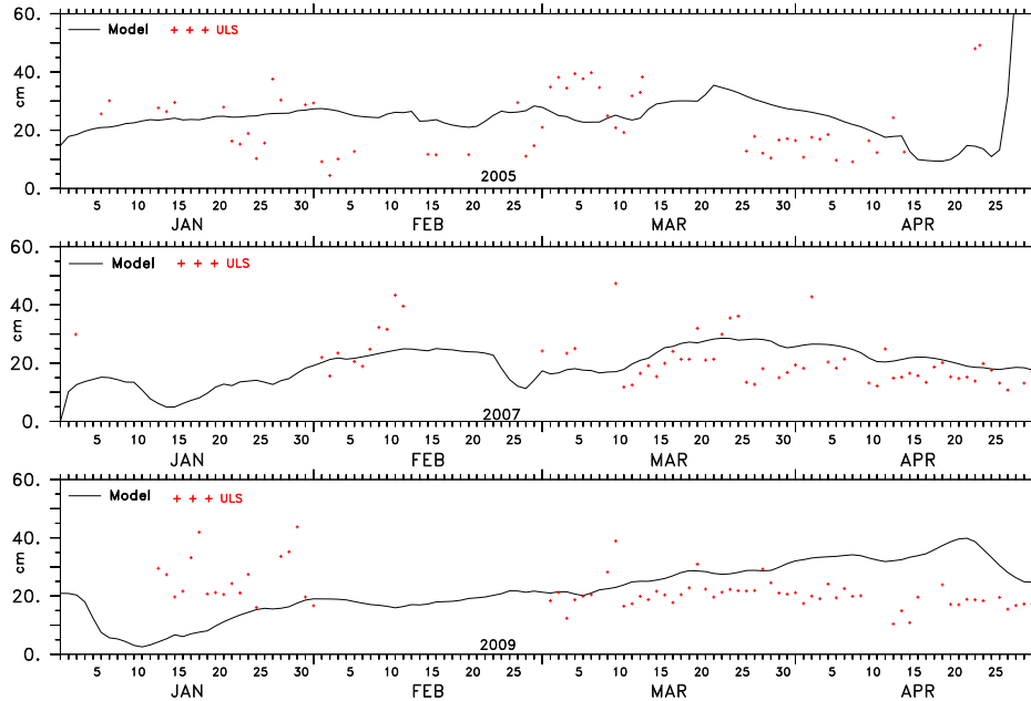
Figure 13. The level ice draft computed from the ULS measurement and the model estimated values in cm for 2005, 2007 and 2009.
