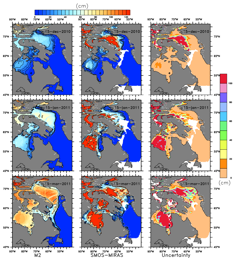
Figure 8. The model 'M2' estimated ice thickness, SMOS-MIRAS derived ice thickness, and the observation uncertainty for 2010-2011.
