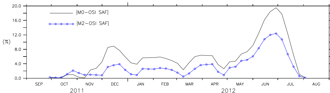
Figure 4. The absolute error from October 2011 to July 2012, ice concentration is not available for assimilation and hence model M2 will be only assimilated with SST during the period.
