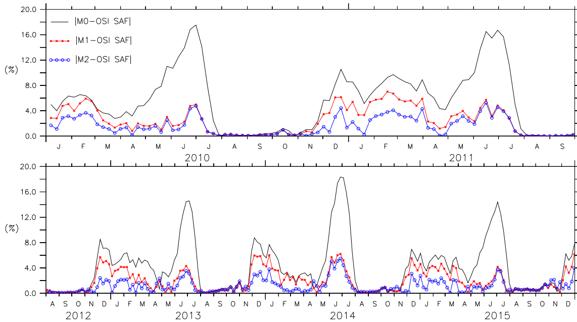
Figure 3. The absolute error for models M0, M1 and M2 from January 2010 to September 2011 is shown in row 1 and from August 2012 to December 2015 is shown in row 2.
