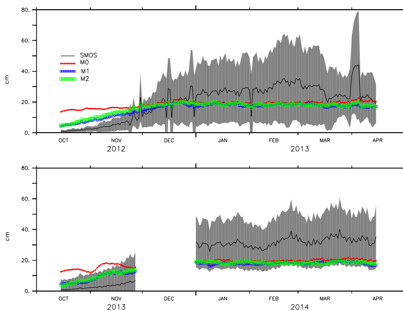
Figure 10. The model 'M2' estimated ice thickness, SMOS-MIRAS derived ice thickness, and the observation uncertainty for SMOS ice thickness less than 30 cm.
