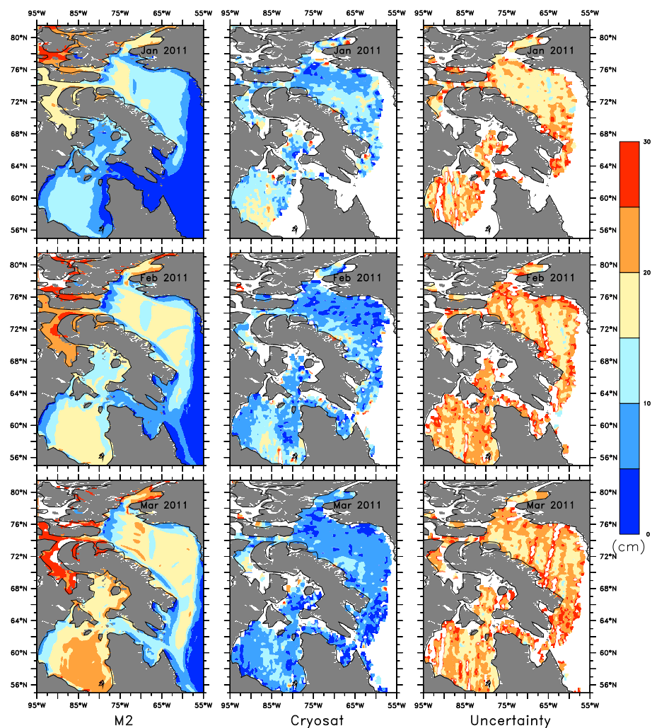
Figure 16. The Freeboard from model M2, CryoSat-2 and the uncertainty of the observations for 2011.
