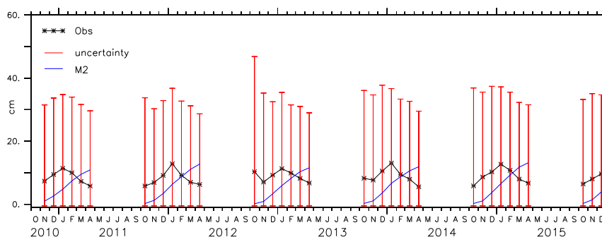
Figure 17. The freeboard from CryoSat-2, uncertainty of the observation and the model M2,
