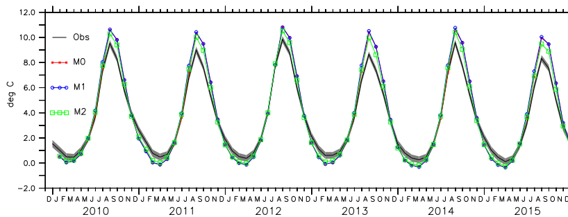
Figure 12. The SST from AVHRR with the shaded region represents the uncertainty of AVHRR SST, and SST from models M0, M1, M2.
