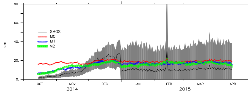
Figure 11. The model 'M2' estimated ice thickness, SMOS-MIRAS derived ice thickness, and the observation uncertainty for SMOS ice thickness less than 30 cm.
