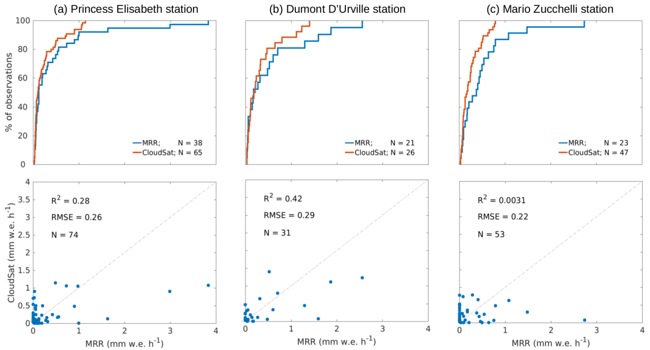
Figure 7. (first row) Empirical cumulative distribution of MRR and CloudSat snowfall events at a spatial resolution of 1^\circ latitude by 2^\circ longitude. (second row) Direct comparison between MRR and CloudSat individual snowfall events. R^2 denotes the adjusted coefficient of determination, RMSE is the root mean square error, N indicates the number of observations, while the thin line is the bisector.
