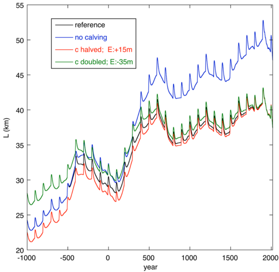
Figure 9. Sensitivity of glacier length to different values of the calving parameter c . For a halved (red curve) or doubled (green curve) value of c the model has been recalibrated by adjusting the ELA (values given in legend).
