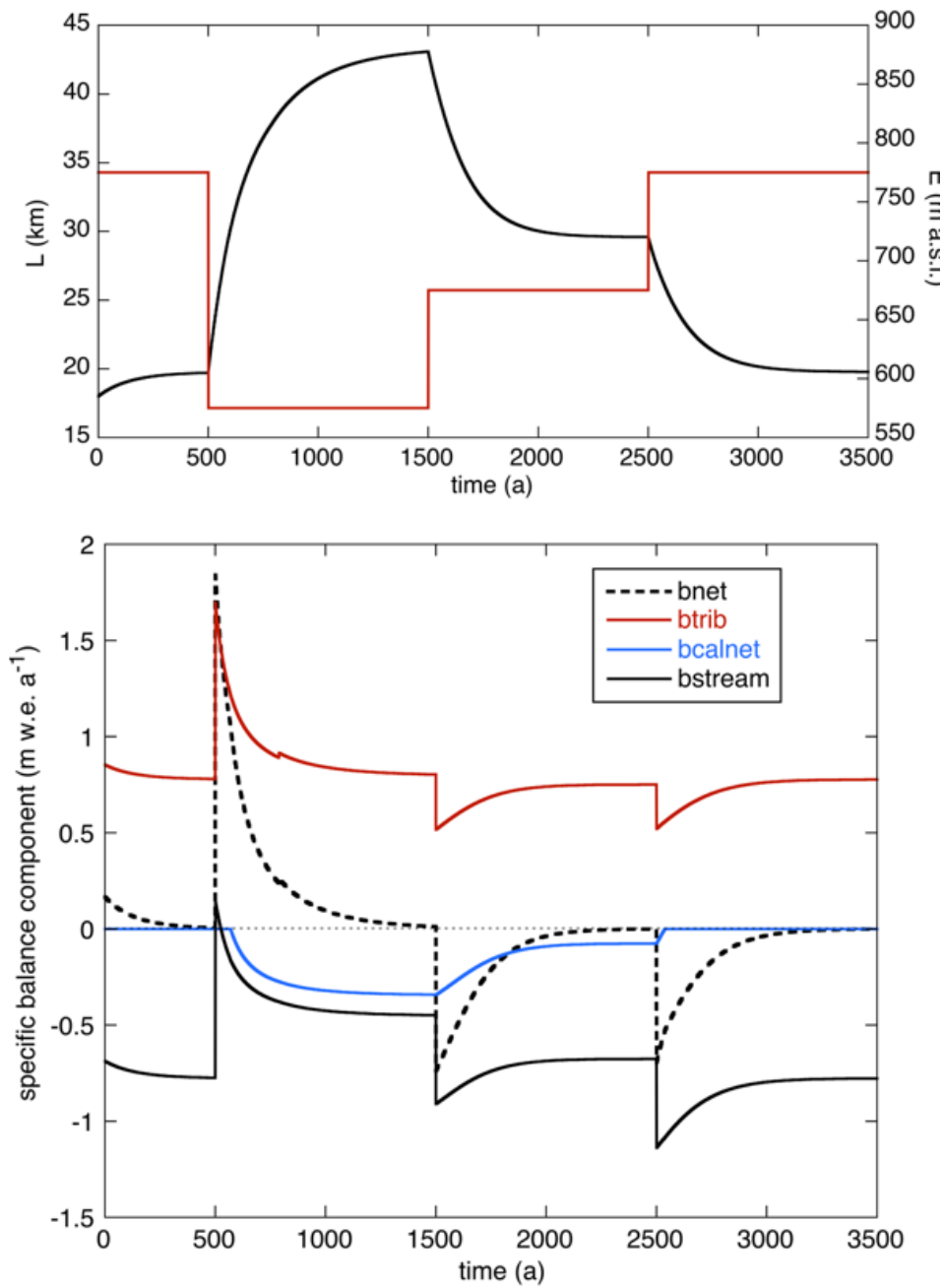
670 Figure 5. Upper panel: Evolution of glaciers length L (black) for stepwise changes in the equilibrium-line altitude E (in red). Lower panel: The corresponding components of the mass budget.
