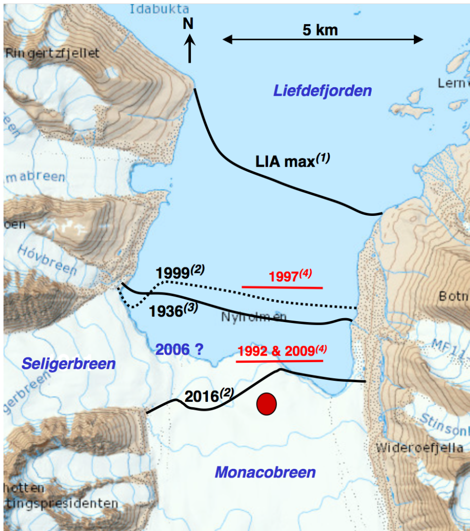
640 Figure 1. Front positions of Monacobreen in different years, drawn on a topographic map of the Norsk Polatinstiutt (http://toposvalbard.npolar.no) . The Little Ice Age maximum stand occurred around 1900 (Martin-Moreno et al., 2017), the 1999 and 2016 positions are from Landsat images (Pelto, 2017). The maximum front position related to the surge was in 1997 (Mansell et al., 2012). The 1992 position is just prior to the surge. In 2009 the glacier front had retreated back to this location. The red dot serves as a reference point for glacier length ( L = 37.8 km).
