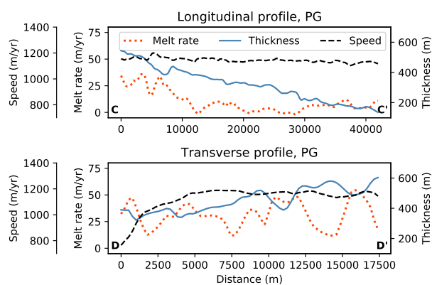
Figure 3. Velocity, melt rate, and ice thickness profiles for PG. Longitudinal profile is outside of a long sub-shelf channel. Transverse profile is taken approximately 1 km downstream of the upstream flux gate.
