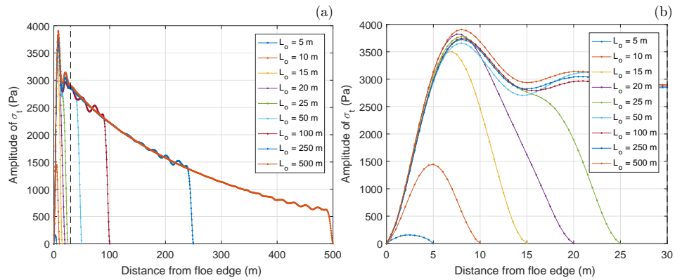
Figure 7. Amplitude of the tensile stress \sigma_t in function of the distance from the upwave ice edge for different floe length L_o ; open-water wavelength L_{w,0} = 42 m, ice thickness h_i = 0.5 m. The plot in (b) is a close-up of the region to the left of the dashed line in (a).
