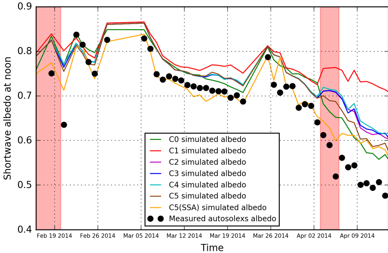
Figure 5. Shortwave broadband albedo at noon. The colored lines correspond to simulated albedo while the black dots correspond to Autosolexs measured albedo (Dumont et al., 2017). The two major Saharan dust events are represented by the red shading.
