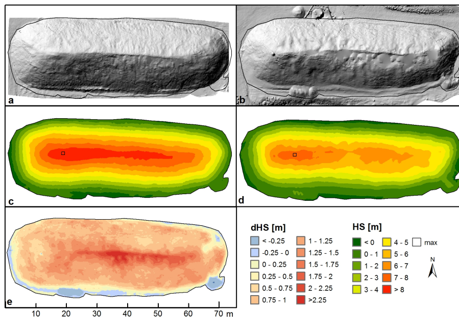
Figure 5. Flüela snow heap: Hillshade images (a: 29 Apr, b: 8 Oct), snow heights HS (c, d) and snow height change dHS (e). The area of the maximum HS at 29 Apr is indicated in c and d.
