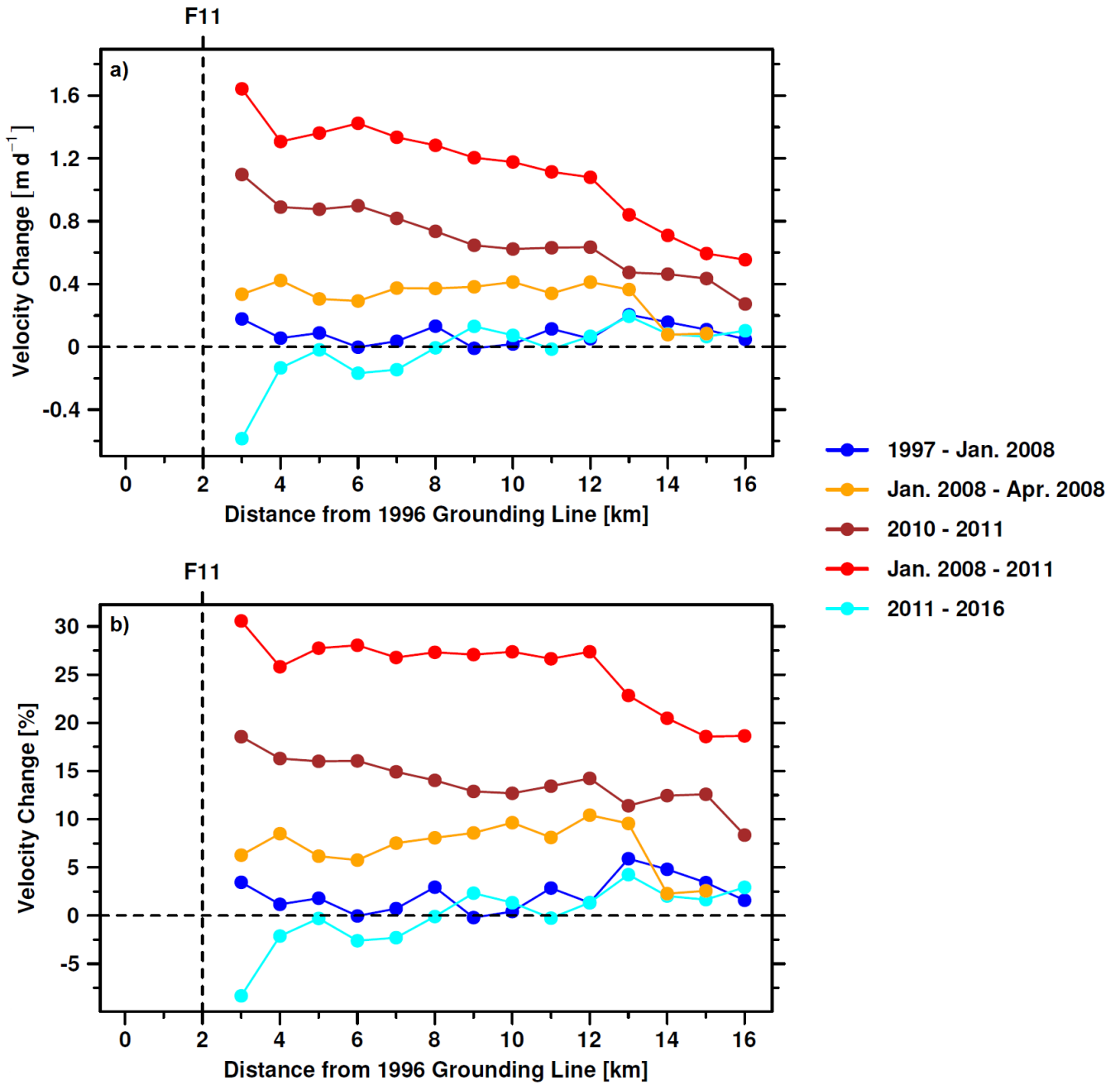
Figure 3: Absolute (a) and relative (b) velocity change along the centreline profile on Fleming Glacier (Fig. 1) for 1997-02-27 to 2008-01-05, 2008-01-05 to 2008-04-30, 2010-02-08 to 2011-10-02, 2008-01-05 to 2011-10-02 and 2011-10-02 to 2016-03-13. F11: front position in 2011. See Tab. S1 for data used for front mapping.
