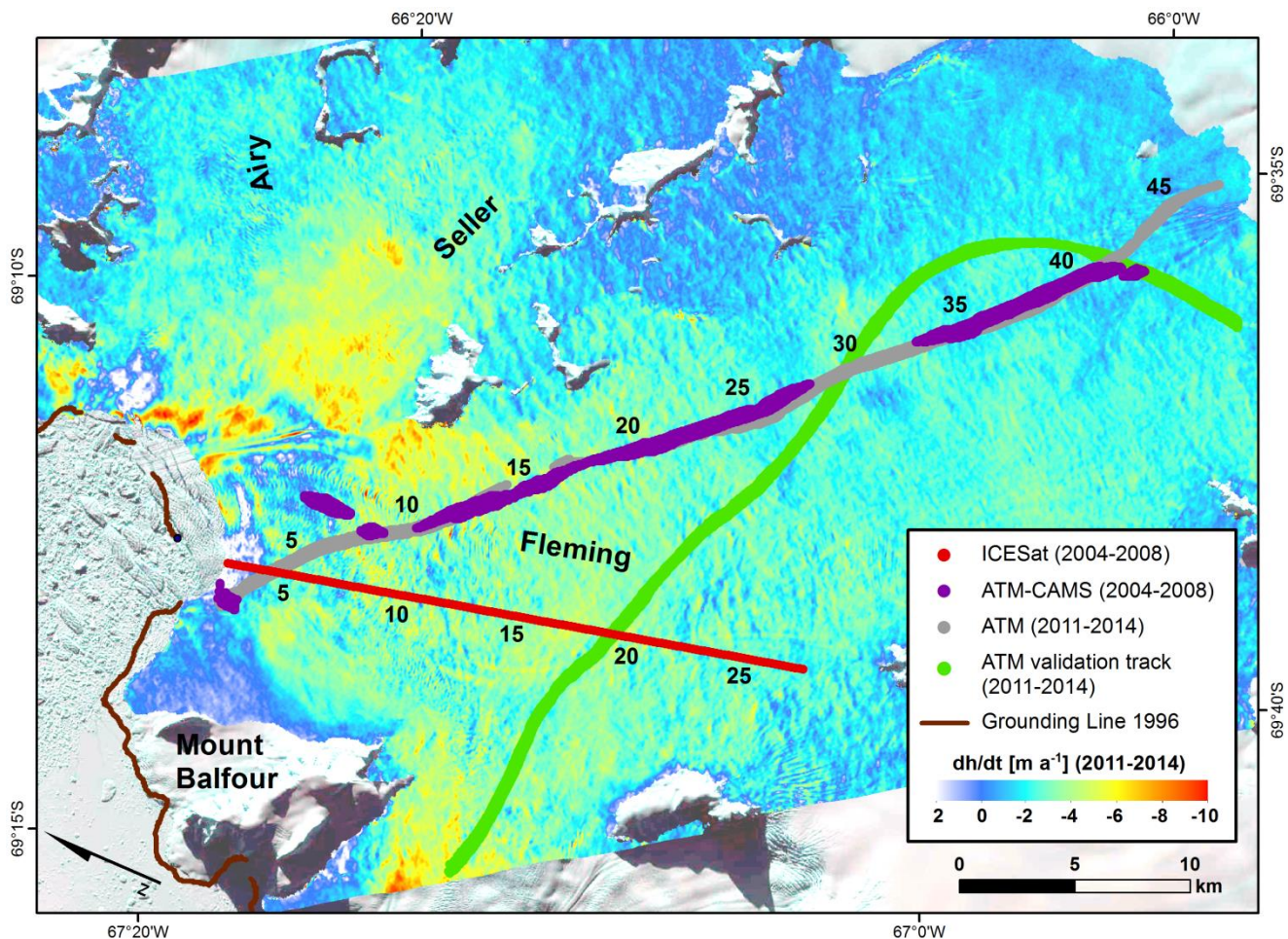
5 Figure 4: Glacier surface elevation change on Fleming Glacier between 2011 and 2014 derived from TSX/TDX bistatic and monostatic acquisitions. Red dots: ICESat track on 2008-10-04 taken as reference for ICESat 2004–2008 dh/dt calculations. Purple dots: common locations of PIB ATM and CAMS LiDAR measurements in 2004 and 2008. Grey dots: common locations of OIB ATM LiDAR measurements in 2011 and 2014. Green dots: common locations of OIB ATM LiDAR measurements in 2011 and 2014 taken for validation of the 2011–2014 TSX/TDX dh/dt measurements. Brown line: grounding line in 1996 from Rignot et al. (2005) and Rignot et al. (2011a). Numbers indicate distances to the 1996 grounding line. Background: Mosaic of two Landsat-8 “Natural Color” images, acquired on 2015-09-16 ©USGS.
