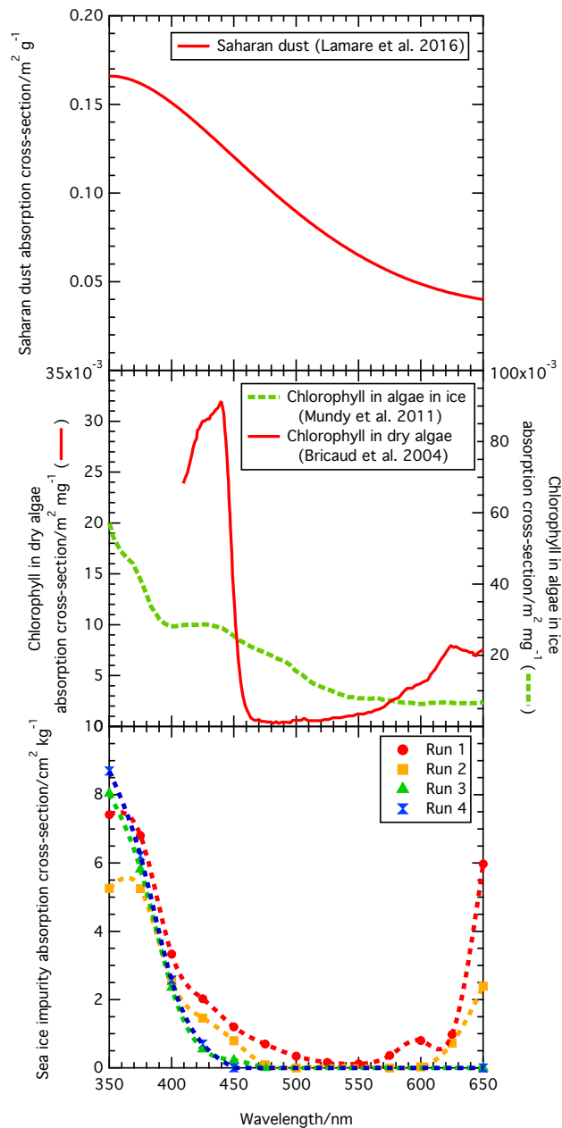
Figure 9. a-A (top)) Absorption cross-section of Saharan dust taken from Lamare et al. (2016) . B (middle)) Absorption cross-sections of chlorophyll. Chlorophyll in ice (dashed line) taken from Mundy et al. (2011) is per mg of algae determined by fluorescence. Chlorophyll (solid line) is taken from Bricaud et al. (2004) is per mg of dry weight cells. b-C (bottom)) Wavelength dependent absorption cross-section derived from reflectance and e -folding depth data from runs 1 to 4 for the undoped ice. A smooth line is added to guide the eye. Values for run 4 are too small to plot clearly at longer wavelengths. Error bars show the possible variation in absorption cross-section obtained from different fits of the original reflectance and e -folding depth data.
