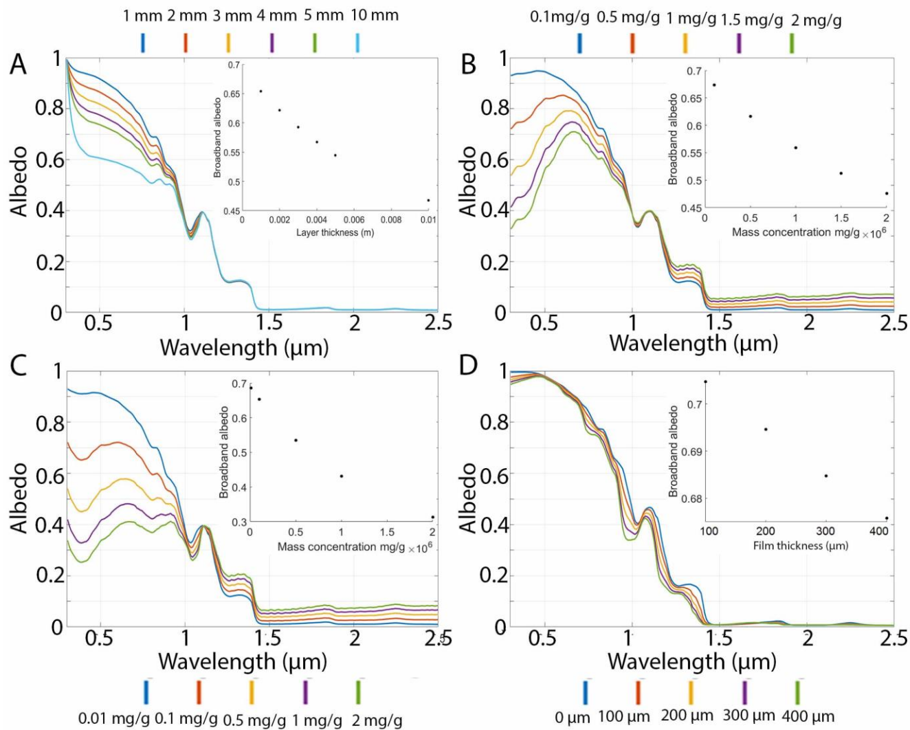
Figure 4: A constant biomass ( 0.5 \text{ mg}_{\text{algae}} / \text{g}_{\text{ice}} , pigment mass fractions (% total cell dry mass) = 1.5% chlorophyll a, 5% primary and secondary carotenoids, 15 \mu\text{m} cell radius) distributed vertically in layers of ice ( 1500 \mu\text{m} grain radius) of varying thickness (1, 2, 3, 4, 5, 10 mm). B) Varying concentrations of mineral dust in a 3 mm surface layer ( 0.1, 0.5, 1, 1.5, 2 \text{ mg}_{\text{dust}} / \text{g}_{\text{ice}} ) on otherwise clean ice (grain radius 1500 \mu\text{m} ). The dust used was SNICAR's 'dust 4' which has grain radii 2.5 - 5 \mu\text{m} ; C) Equal mass concentrations ( 0.01, 0.1, 0.5, 1, 2 \text{ mg}_{\text{impurity}} / \text{g}_{\text{ice}} ) of algal cells (pigment mass fractions (% total cell dry mass) = 1.5% chlorophyll a, 5% primary and secondary carotenoids, 15 \mu\text{m} cell radius) and mineral dust (SNICAR's 'dust 4' which has grain radii 2.5 - 5 \mu\text{m} ) in a 3 mm surface layer in otherwise clean ice ( 1500 \mu\text{m} grain radius); D) Albedo of a dry snowpack (grain radii = 1000 \mu\text{m} ) and snowpacks with liquid water as a coating around the ice grains. The legend indicates the thickness of water layer around a 1000 \mu\text{m} ice grain. Insets show broadband albedo plotted against the relevant model variable.
