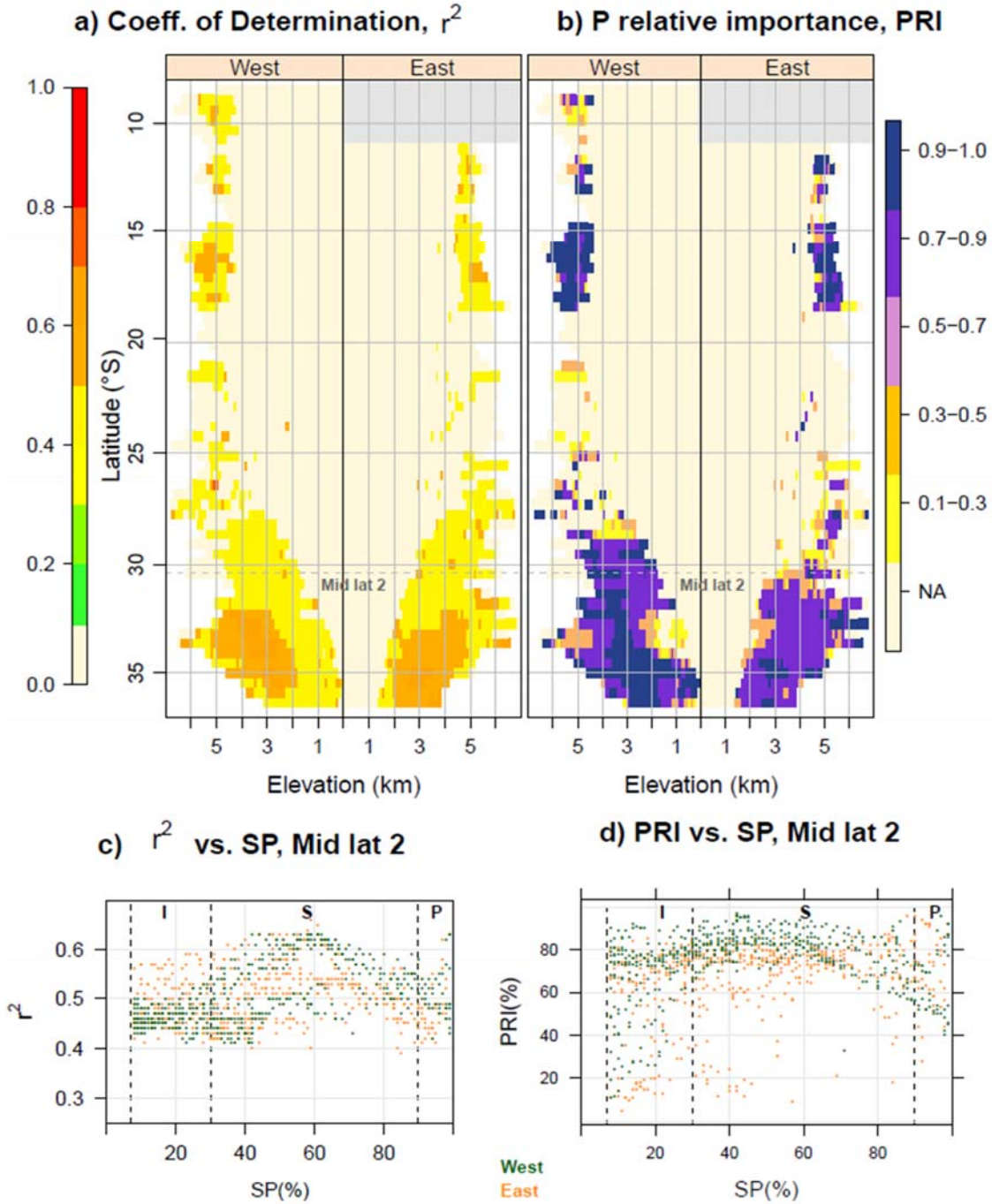
5 Figure 11. Latitude-elevation band analysis of a) coefficient of determination ( r^2 ) for multiple linear regression using annual precipitation and mean air temperature to predict SP, 2000-2014, b) relative importance of precipitation. Grey areas represent latitudes masked due to high frequency of cloud cover in snow covered area analysis (>30% period). c) r^2 vs. SP and d) precipitation relative importance (PRI) in Mid Latitude 2 snow region for West (green) and East (orange) vs SP values. Vertical dashed grey lines inside inset boxes represent thresholds for intermittent (I), seasonal (S), and persistent (P) snow zones.
