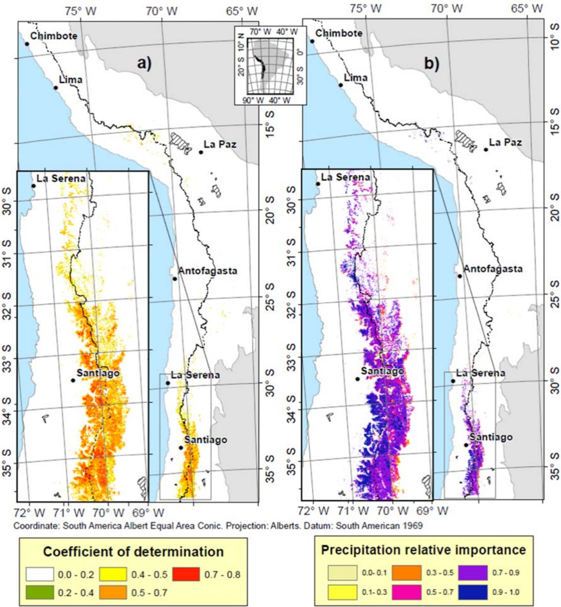
5 Figure 10. Multiple linear regression analysis by pixel showing a) the coefficient of determination ( r^2 ) for SP predictions using annual precipitation and mean annual air temperature) and b) Precipitation relative importance (PRI), indicating the individual contribution of precipitation to the full r^2 of the model.
