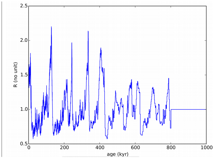
Figure 2: R(t) proportionality factor (see Eq. 3) applied to accumulation and melting rates. The plot is cut at 1 Myr for better readability. R(t) is based on the accumulation record at EDC for the last 800 kyr (Bazin et al., 2013; Veres et al., 2013).
