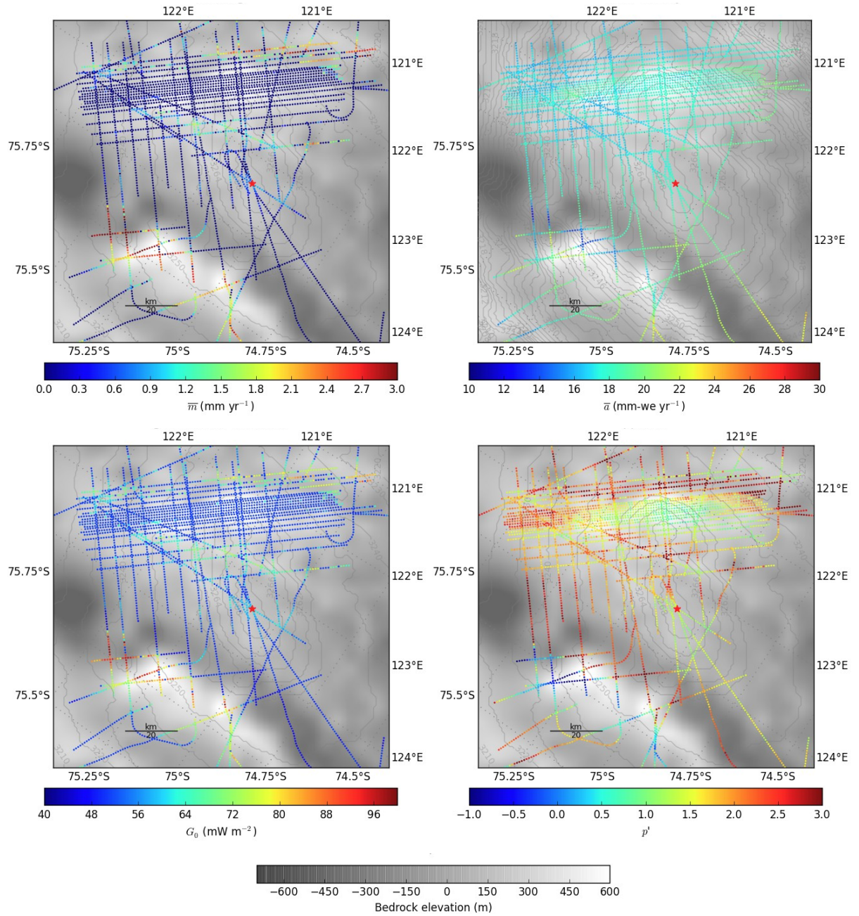
Figure 5: Various variables reconstructed by the inverse method along the radar transects, in vivid colour scale. The bedrock and surface elevations (greyscale light colors and isolines, respectively) are shown as in Figure 1. (Top-Left) Modeled temporally averaged basal melting. (Top-Right) Inferred temporally averaged vertical steady surface accumulation rate. (Left-Bottom) Inferred vertical geothermal flux. (Right-Bottom) Inferred vertical p' vertical velocity parameter.
