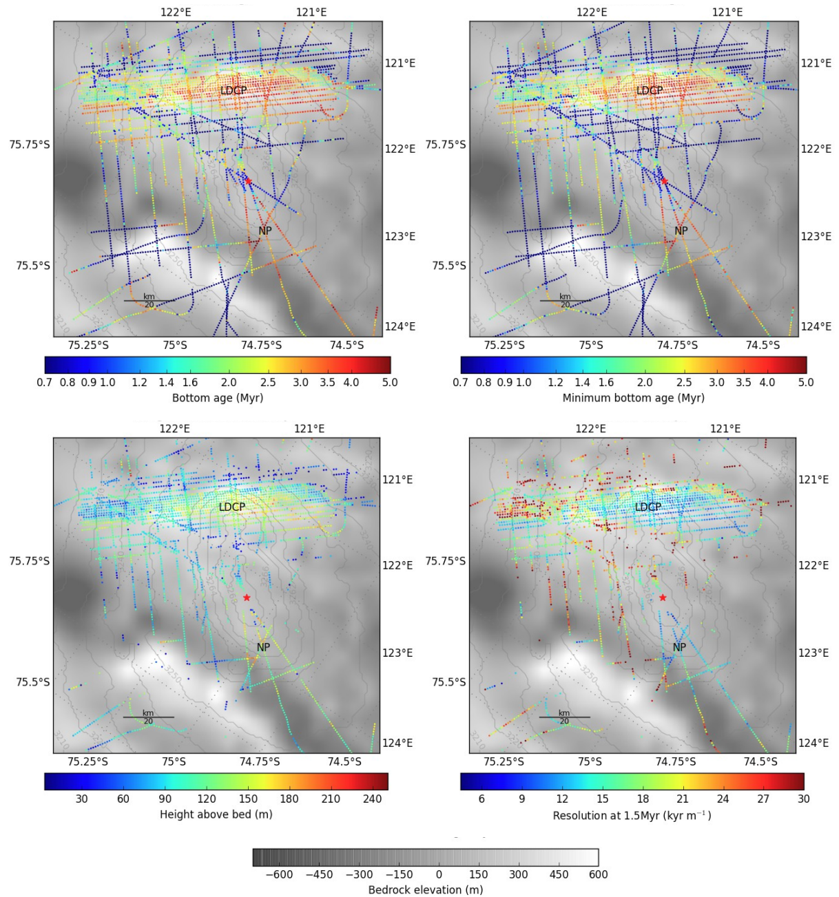
Figure 4: Various bottom age-related variables along the radar transects, in vivid colors. The bedrock and surface elevations (greyscale light colors and isolines, respectively) are shown as in Fig. 1. LDCP and NP are the two old ice patches that we discuss in this study. (Top-Left) Modeled bottom age at 60 m above bedrock. (Top-Right) Minimum bottom age at 60 m above bedrock with 85% confidence. (Bottom-Left) Height modeled age at 150 m above bed of the 1.5 Myr isochrone. (Bottom-Right) Temporal resolution for the 1.5 Myr modeled isochrone.
