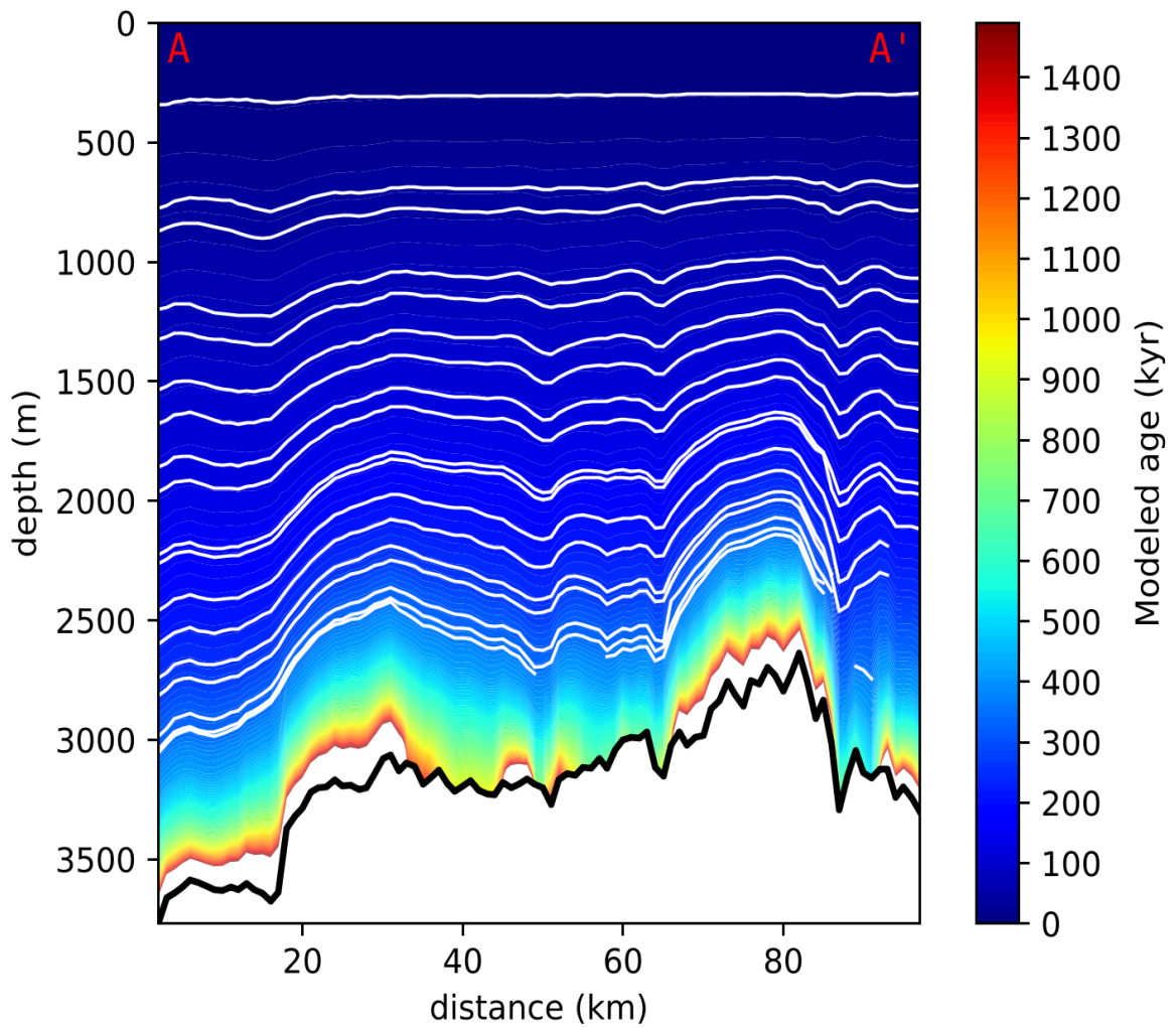
Figure 3: Modeled age (in colour scale, white is for ages older than 1.5 Myr ) along the OIA/JKB2n/X45 radar transect (see red dotted line in Figure 1 for location), together with observed isochrones (in white). Left is north-east and right is south-west. Note the two main Oldest Ice candidates at distance 25 km (NP) and at distance 75 km (LDCP).
