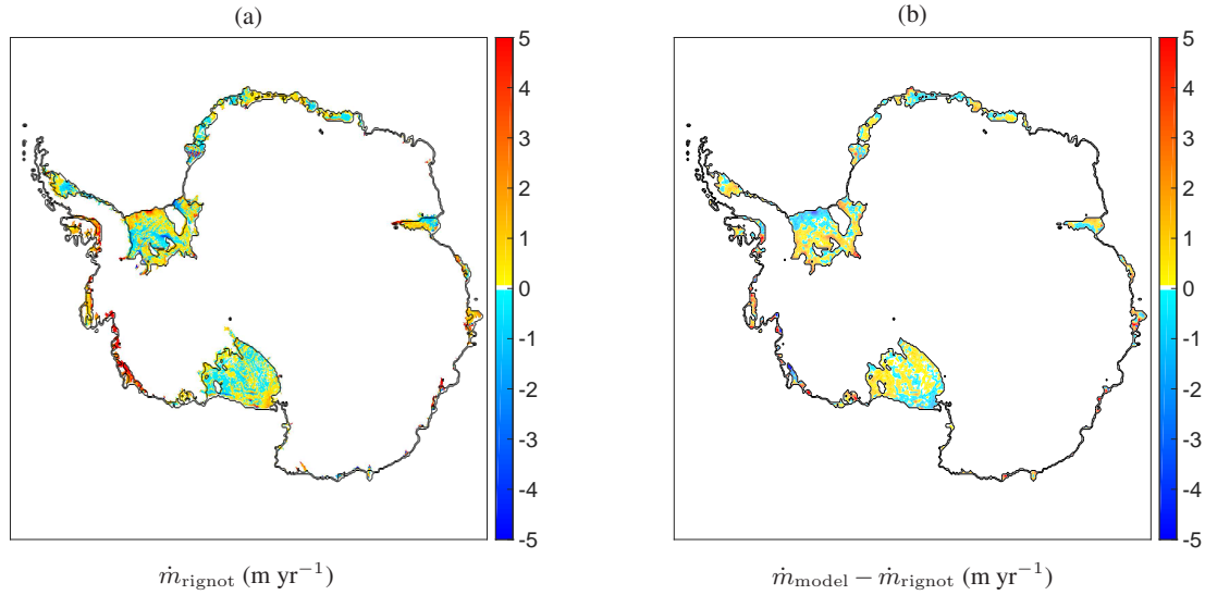
Figure 11. Basal melt rates in meter per year extracted from the Rignot et al. (2013) observational dataset (courtesy of Dr Jeremie Mouginot): (a) raw data plotted together with the currently used mask; (b) difference between the plume parametrization (Fig. 9a) and the observations interpolated on the 20-km grid.
