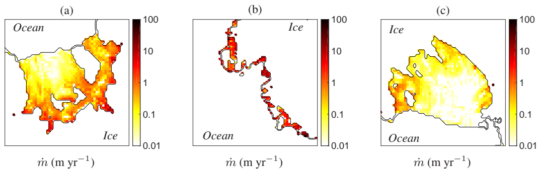
Figure 10. As Fig. 9a, but with a logarithmic color scale (negative and zero values shown white) and zoomed in on (a) Filcher-Ronne ice shelf (group 1), (b) West Antarctica including Pine Island and Thwaites (group 11), (c) Ross ice shelf (group 9).
