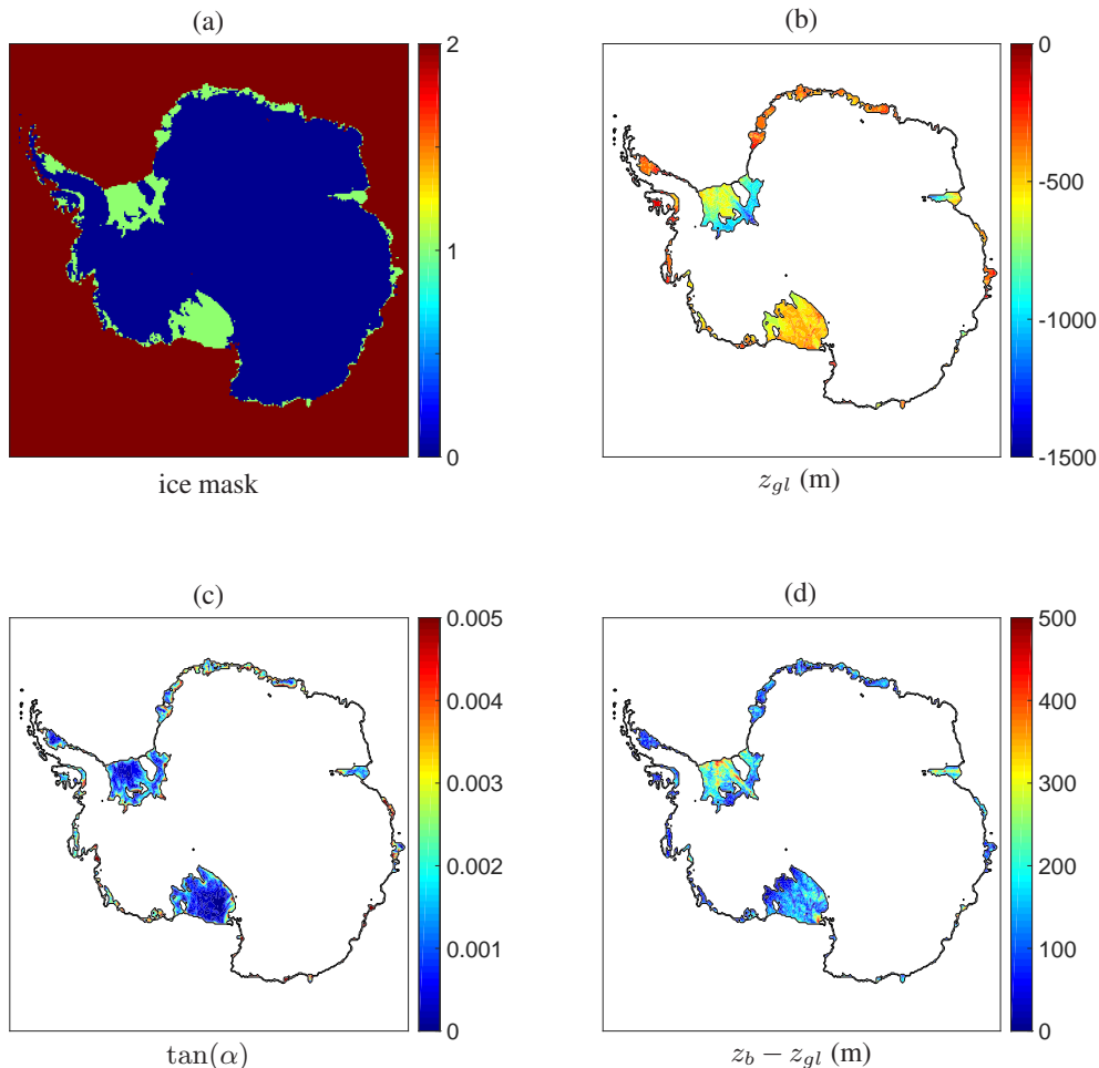
Figure 4. Effective plume paths under the Antarctic ice shelves as calculated by the algorithm of Section 2.3 using the Bedmap2 topographic data remapped on a 20 km by 20 km grid. (a) Ice mask according to Table 2. (b) The effective grounding-line depth z_{gl} . (c) The effective slope \tan(\alpha) . (d) The difference between local ice-base depth and associated grounding-line depth, z_b - z_{gl} .
