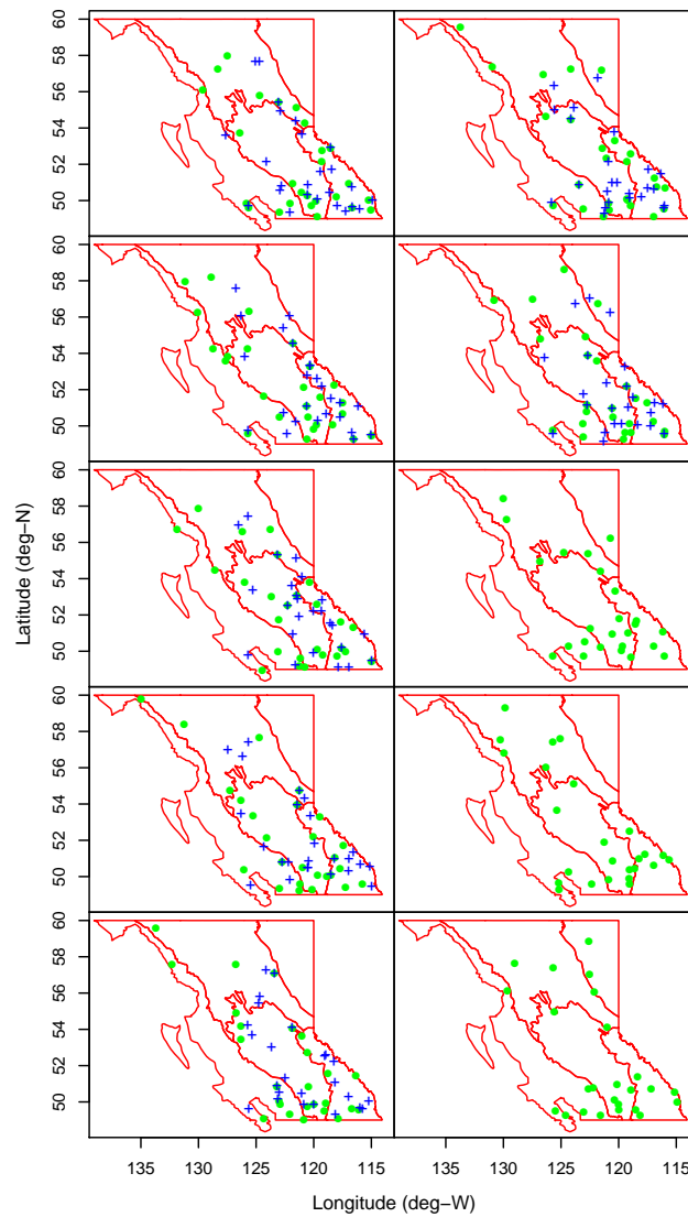
Figure 2. MSS station locations used in evaluating combination products. Green dots show the distribution of ten test splits for comparing means, MLRs, and ANNs to gridded SWE products throughout BC by cross-validation. Blue crosses show the distribution of seven test splits for comparing ANNs to VIC runs in four BC watersheds. Physiographic regions are outlined in red.
