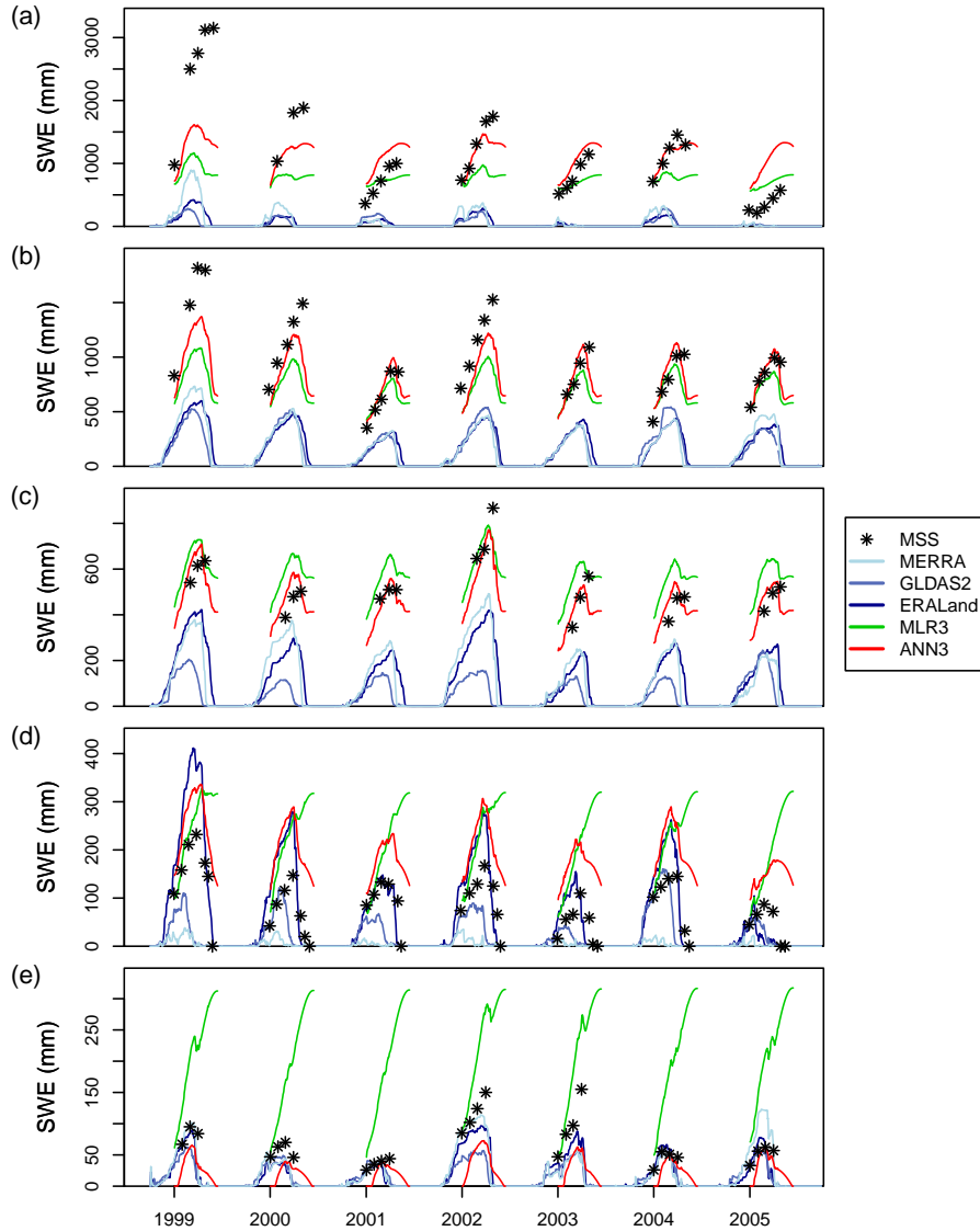
Figure 3. SWE time series for manual snow survey stations, the best three gridded SWE products, MLR3, and ANN3. Gridded products are ordered by increasing overall performance, with darker blues for better performing products. MLR3 and ANN3 estimates are masked outside the mean first and final survey dates (January 2 and June 15 respectively). A representative station is shown for each of the five physiographic regions of BC: (a) station 1D08 Stave Lake in the Coast Mountains and Islands, (b) station 2A25 Kirbyville Lake in the Columbia Mountains and Southern Rockies, (c) station 4B08 Mount Cronin in the Northern and Central Plateaus and Mountains, (d) station 2F11 Isintok Lake in the Interior Plateau, and (e) station 4C05 Fort Nelson Airport in the BC Plains.
