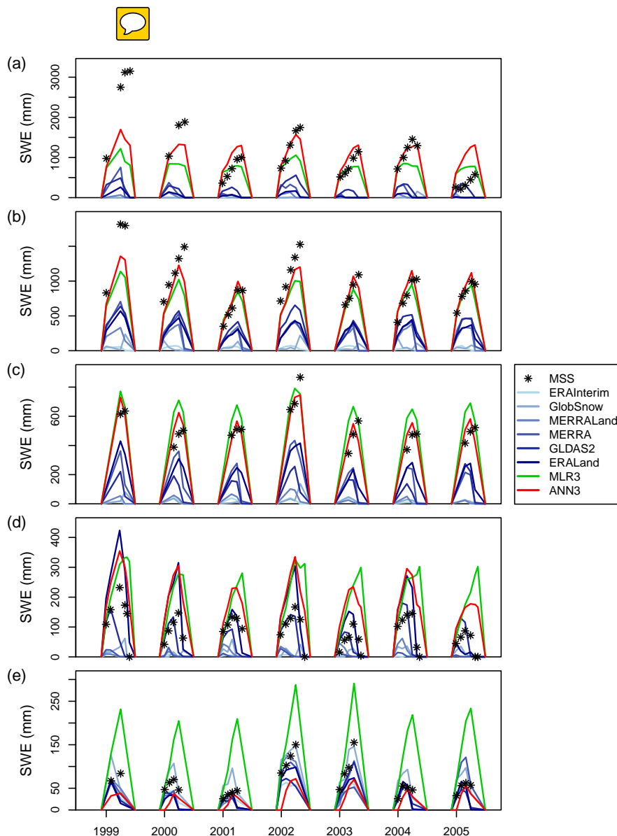
Figure 3. SWE time series for manual snow survey stations, gridded SWE products, MLR3 and ANN3. Gridded products are ordered by increasing overall performance, with the darkest blues for the best performing products. A representative station is shown for each of the 5 physiographic regions of BC: (a) station 1D08 Stave Lake in the Coast Mountains and Islands, (b) station 2A25 Kirbyville Lake in the Columbia Mountains and Southern Rockies, (c) station 4B08 Mount Cronin in the Northern and Central Plateaus and Mountains, (d) station 2F11 Isintok Lake in the Interior Plateau, and (e) station 4C05 Fort Nelson Airport in the BC Plains.
