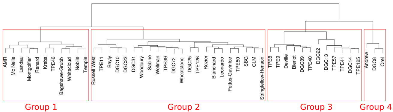
Figure 6. Dendrogram of hierarchical cluster analysis of glaciers in sector "West". The glaciers are assorted in four groups (red rectangles). See also Section 5.3.
