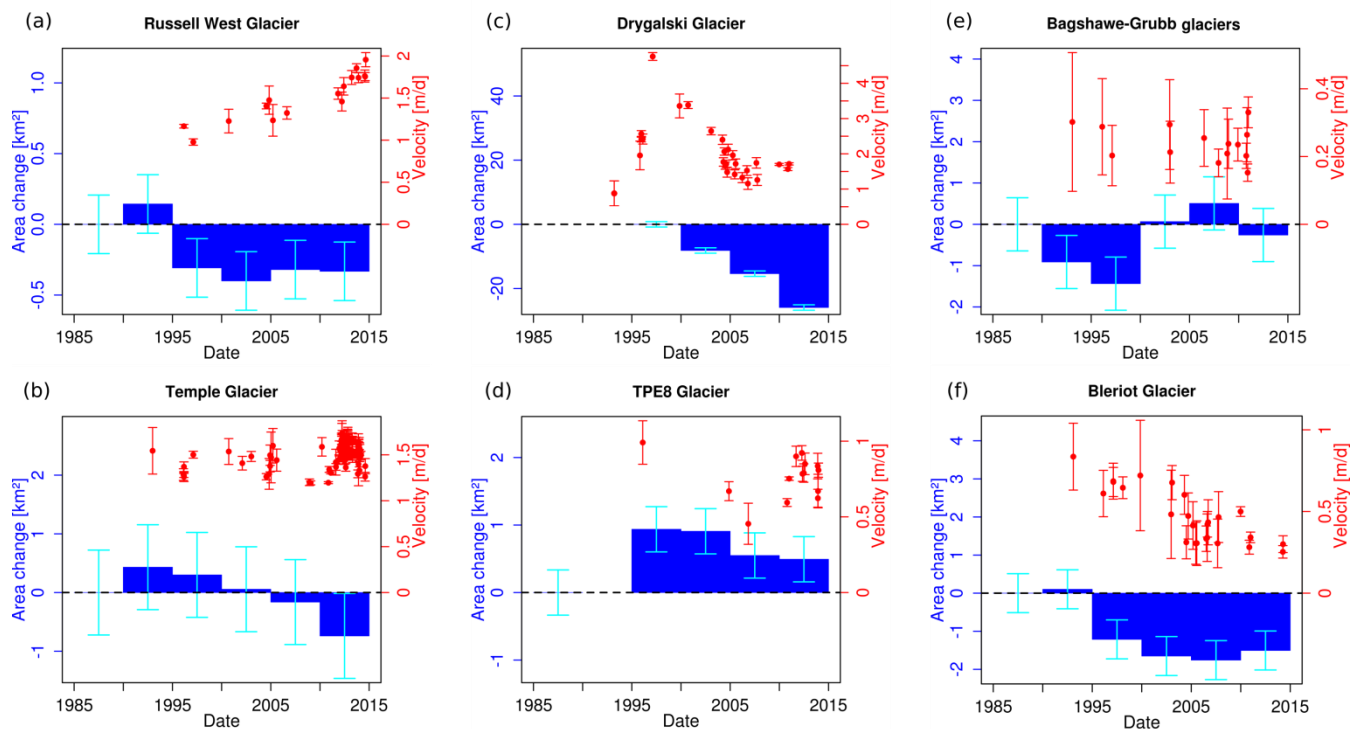
Figure 2. Temporal evolution of surface velocity (red) and area (blue) changes of selected glaciers in the study area for each velocity change category (see Table 3).
