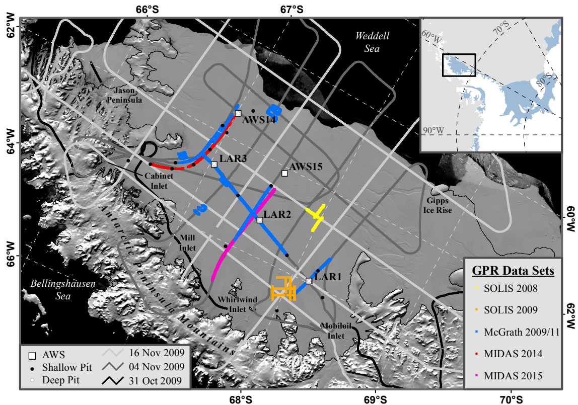
Figure 1. Map showing fieldwork locations, Operation Ice Bridge flight lines, GPR tracks, and relevant geographical names. The MODIS mosaic of Antarctica is shown in the background (Scambos et al., 2007; Haran et al., 2014).
