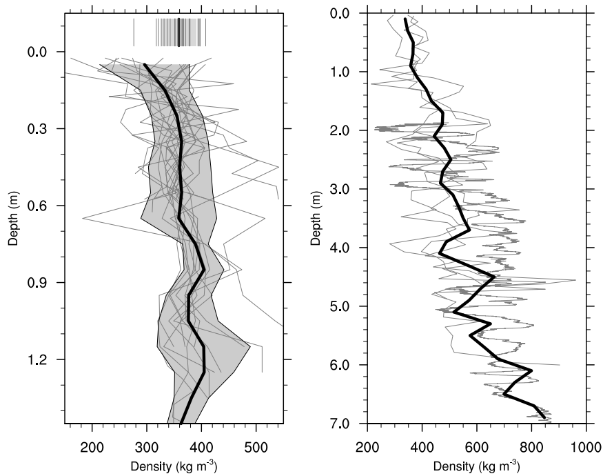
Figure 4. Vertical profiles of snow and firn density used to convert the observed surface height changes to mass fluxes. Thick lines indicate mean density profiles, with shading denoting one standard deviation. (a) Snow pit observations between 0 and 1.50 m. Vertical bars in the top of the figure are vertically integrated densities, including the mean vertically-integrated density as a thick bar; (b) firn core observations (gravity coring and OPTV logging) up to 7 m below the surface. Note different depth and density scales between the panels.
