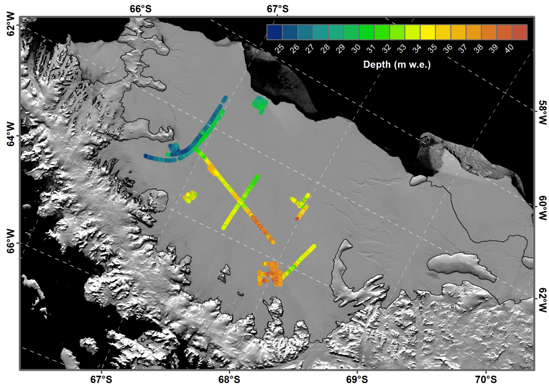
Figure 7. Map of LCIS showing estimated total mass (m w.e.) above the strong, undated reflection horizon along the GPR tracks.
