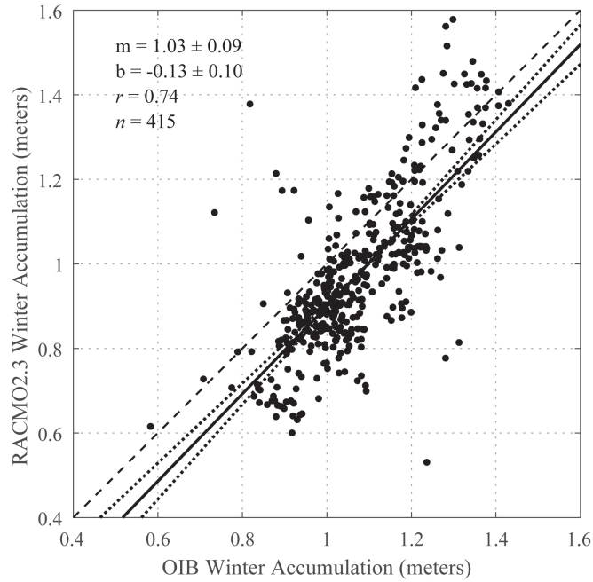
Figure 9. Comparison between Operation Ice Bridge-derived and RACMO2-simulated winter accumulation (m) between February and November 2009, based on 415 equally-spaced observations along the OIB flight lines. The 1:1-line is dashed; the linear fit is represented by a solid line, with associated uncertainty of the fit in dashed lines. Slope of the fit line is m and intercept with the vertical axis is b .
