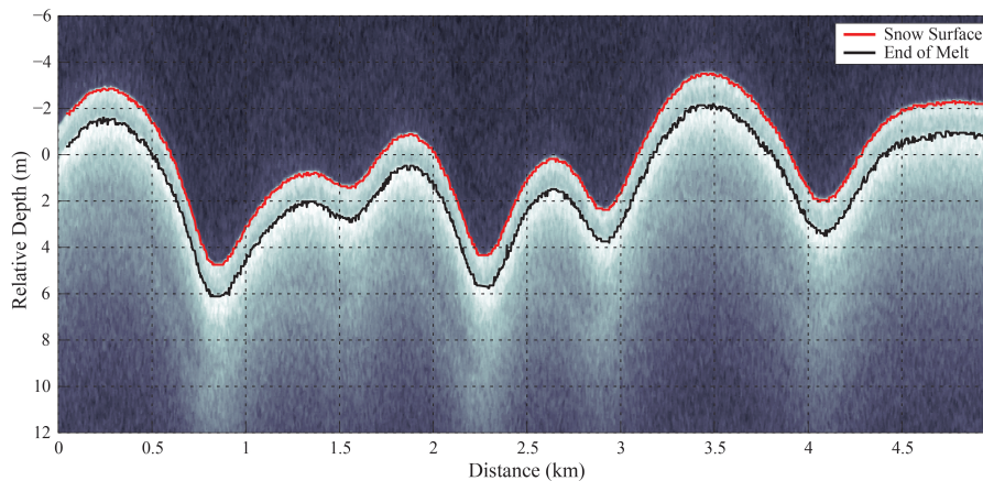
Figure 2. Sample radar echogram obtained from CReSIS Ku-band radar (14–16 GHz) onboard the 16 November 2009 Operation Ice Bridge flight. Automated surface and subsurface picks are overlaid. Nearly all echograms look similar with very strong surface and a strong to very strong subsurface reflection horizon. The subsurface horizon is interpreted as the end of the melt season, and it physically represents the transition from dry snow (above) and snow that has strong melt features (ice lenses).
