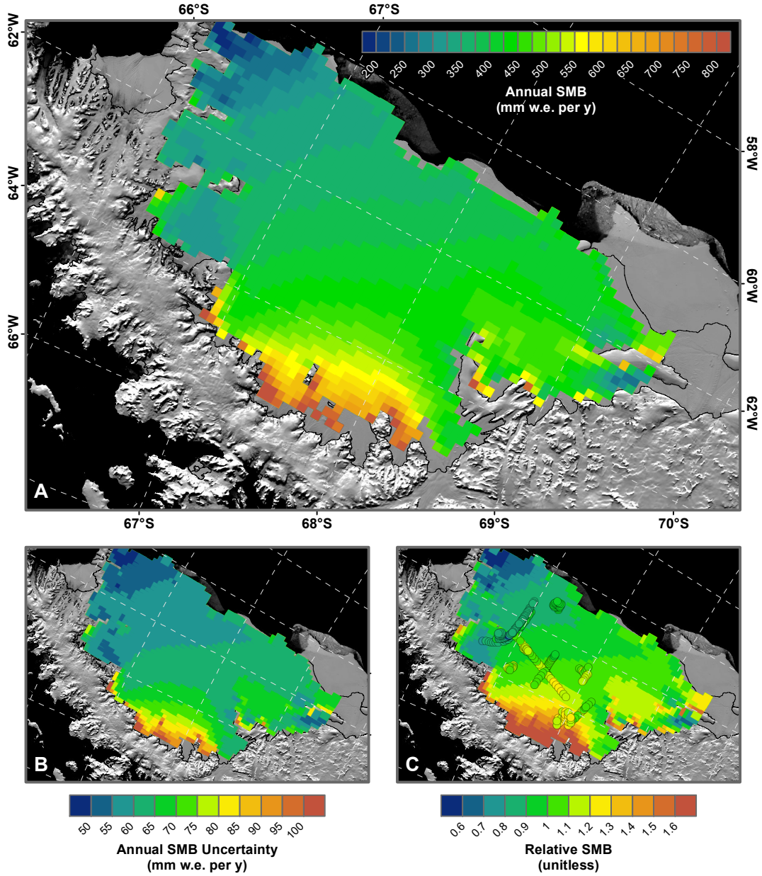
Figure 10. (a) Map of Larsen C Ice Shelf showing a reconstruction of annual SMB (in \text{mm w.e. y}^{-1} ), obtained by adjusting 1979–2014 RACMO2 SMB to the spatial pattern of ground-penetrating radar, and to observations of SMB from sonic height rangiers; (b) Estimated uncertainty of the SMB values in panel a (in \text{mm w.e. y}^{-1} ); (c) Coloured dots indicate depth of the reflection horizon, detected by GPR, normalized with respect to the mean depth (unitless). The background shows a map of relative SMB (unitless) from RACMO2.
