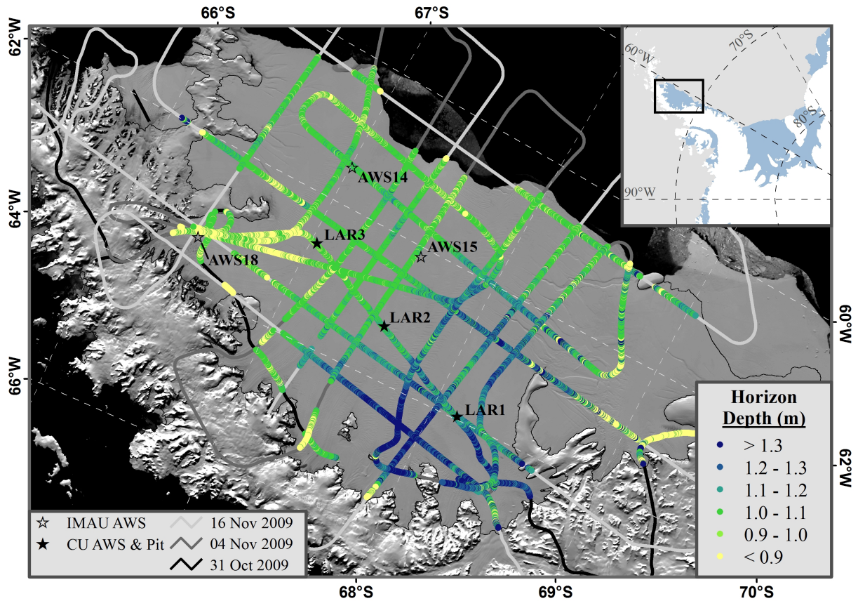
Figure 8. Map of LCIS showing Operation Ice Bridge reflector depths (in m) for the 2009 flight lines. Stars indicate the locations of automatic weather stations, with solid stars at locations where snow pit observations were made concurrent with the OIB overpasses.
