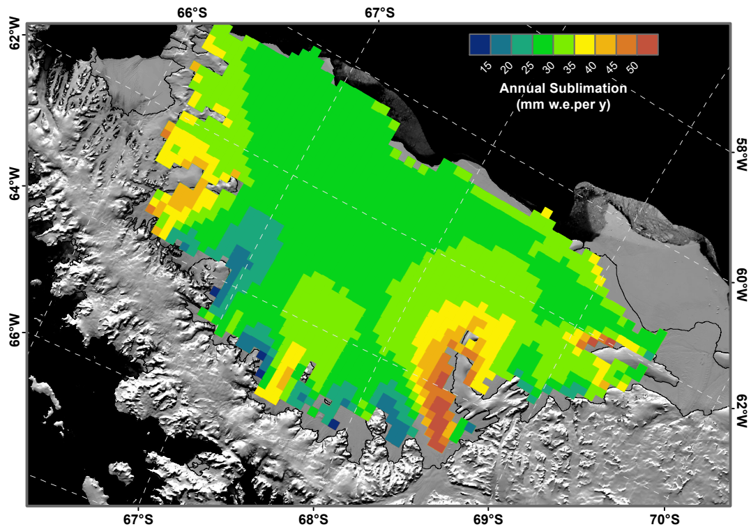
Figure 12. Annual mean sublimation (mm w.e. y^{-1} ) simulated by RACMO2 over LCIS, averaged over 1979–2014.
