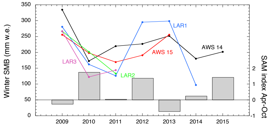
Figure 5. Time series of winter (Apr–Oct) surface mass balance (mm w.e.) derived from sonic height rangiers, with left vertical axis. Magnitude of the southern annular mode (SAM) is shown as gray bars, with the right vertical axis.
