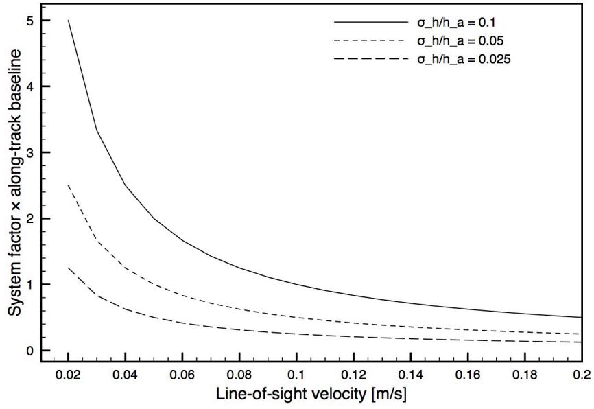
Figure 5: Along-track baseline B_{al} multiplied with the system factor C_{sys} versus the sea ice line-of-sight velocity for different ratios between relative height error and ambiguity height. See text for further explanations.
