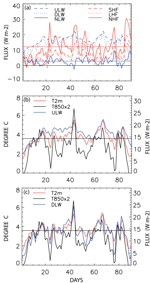
Fig. 3. The daily patterns of variability over the region of sea ice loss (21°-79.5°E × 75°-79.5°N) (reproduced from Figure 6 in the manuscript).
