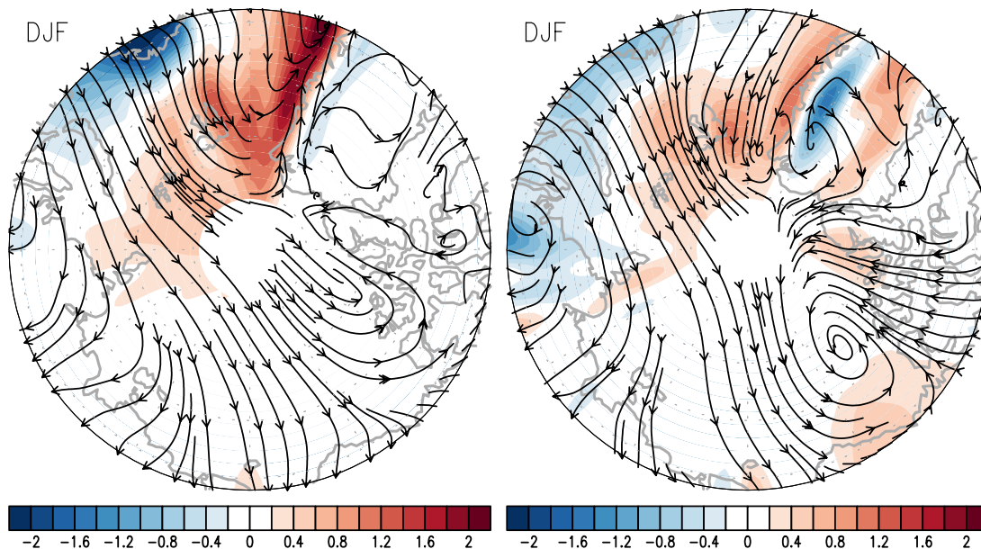
Fig. 4. Winter-averaged (left panel) moisture transport (streamline) and its convergence (shade) and (right panel) heat transport (streamline) and its convergence (shade) in the lower troposphere (1000-850 hP)
