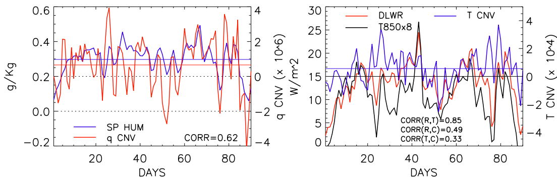
Fig. 5. The daily time series of anomalous specific humidity and anomalous moisture convergence averaged over the sea ice loss region ( 21^{\circ} - 79.5^{\circ} E \times 75^{\circ} - 79.5^{\circ} N) in the Barents-Kara Seas. This particular time
