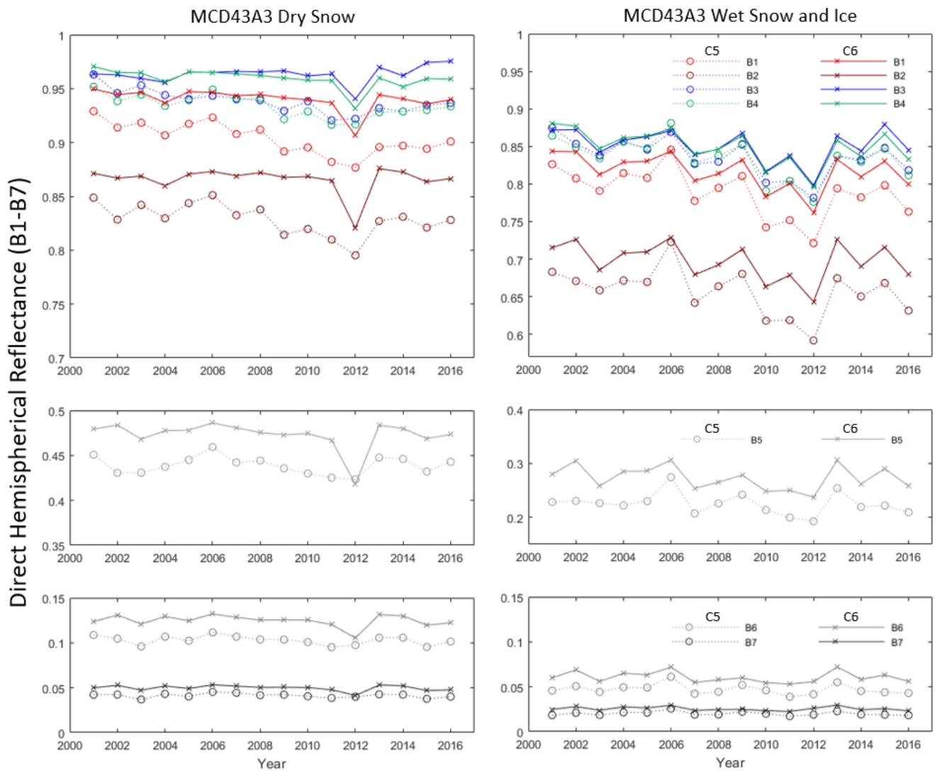
5 Figure 4: Greenland ice sheet average summer (Jun 1 - Aug 31) MCD43A3 BSA C5 and C6 Band 1-7 albedo for dry (left) and wet snow and ice (right). (Note the y-axis scale is different for dry vs. wet snow and ice for B1-4 and B5). Interestingly, there is a separation in C5 to C6 B1, B2, B4, B5, B6 albedo values throughout the MODIS record.
