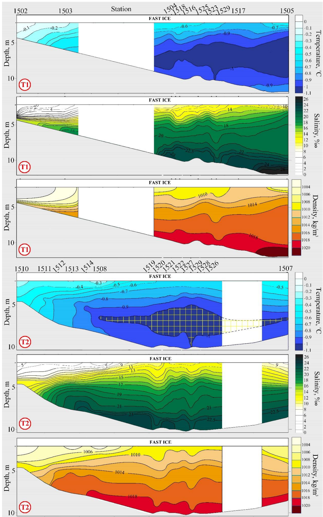
Figure 7: Vertical sections of winter salinity, temperature, and density distributions. The location of transects T1 and T2 is shown in Figure 2. A yellow cell shows a “mushroom-like structure”. In places where there are no data, white gap are shown.
