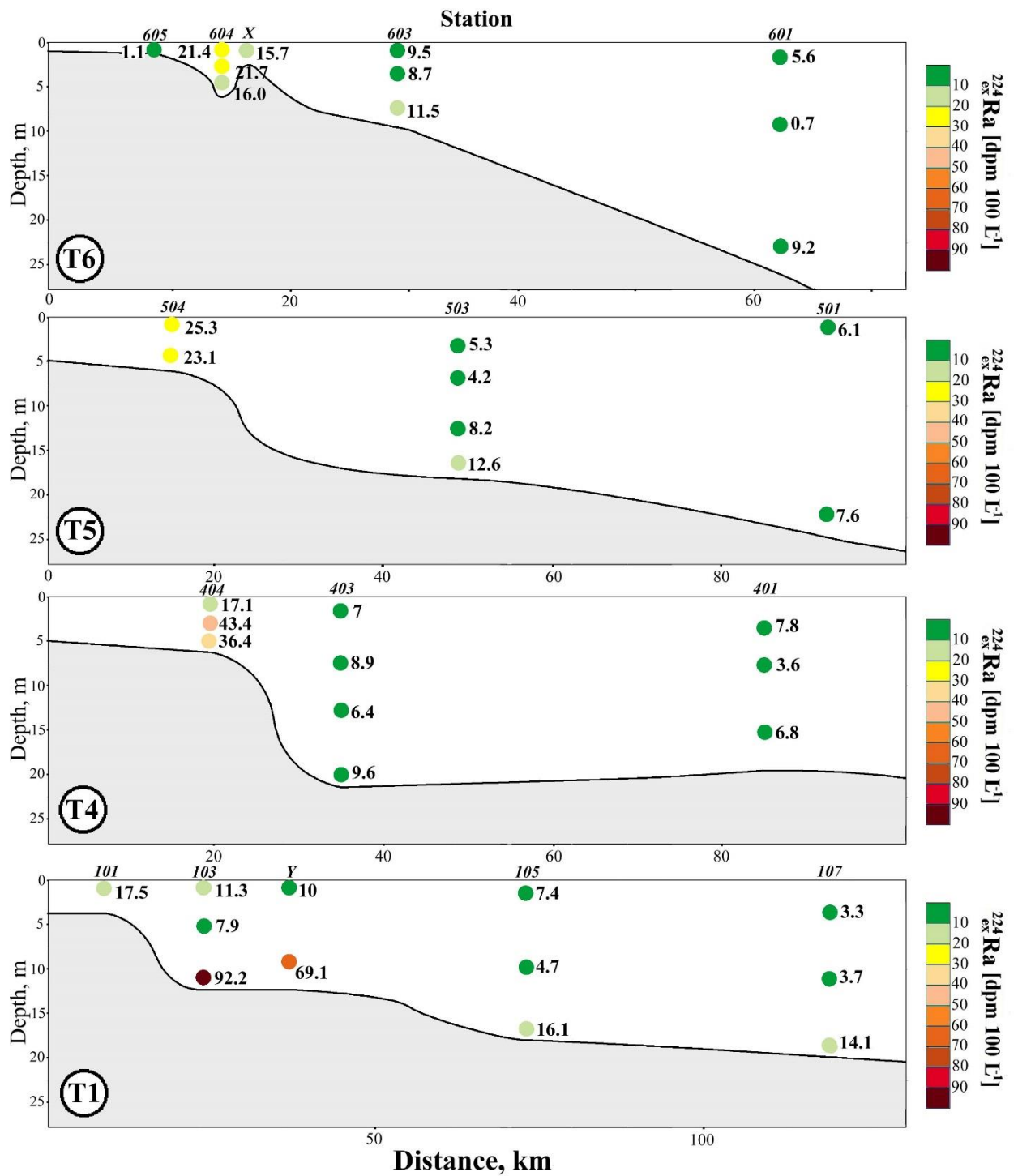
Figure 11: Summer (September 2013) vertical distribution of \text{ex}^{224}\text{Ra} in the Lena Delta. Sta Y (72°N, 130°E) is included in transect T1.
