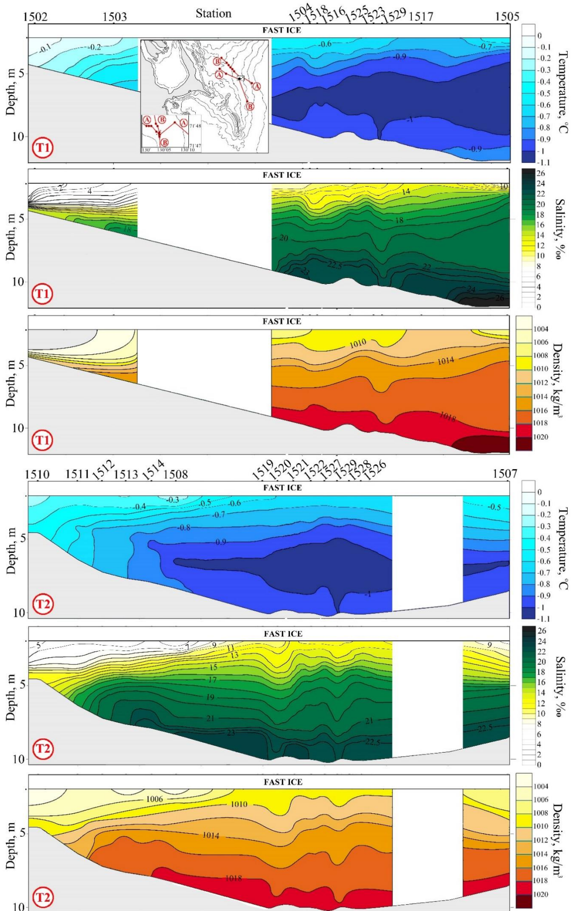
Figure 7: Vertical sections of winter salinity, temperature, and density distributions.
