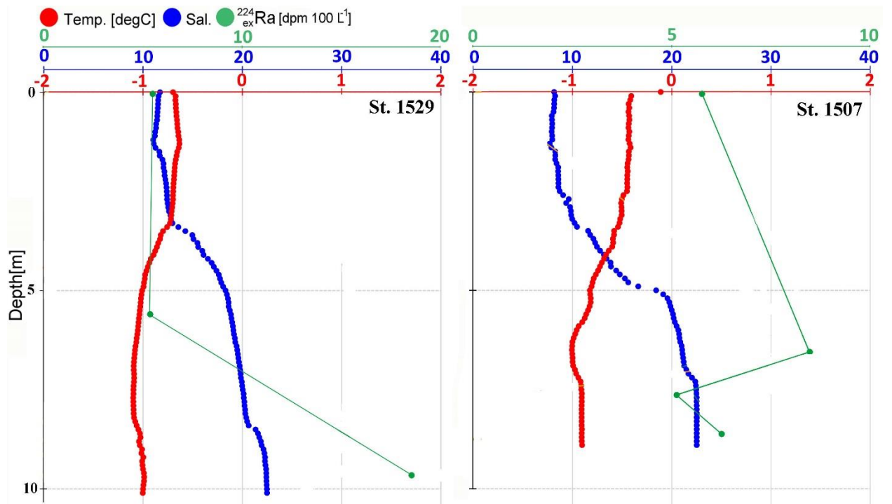
Figure 9: Vertical profiles of the winter water column.
