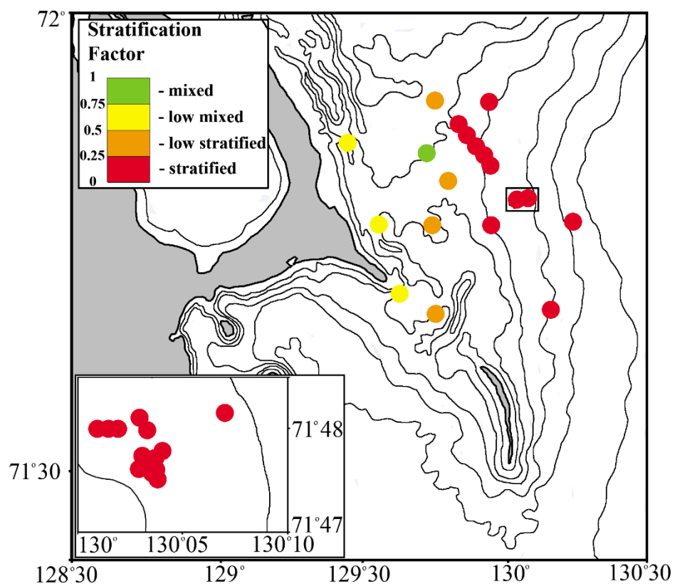
Figure 5: Winter stratification factor in the study areas.
