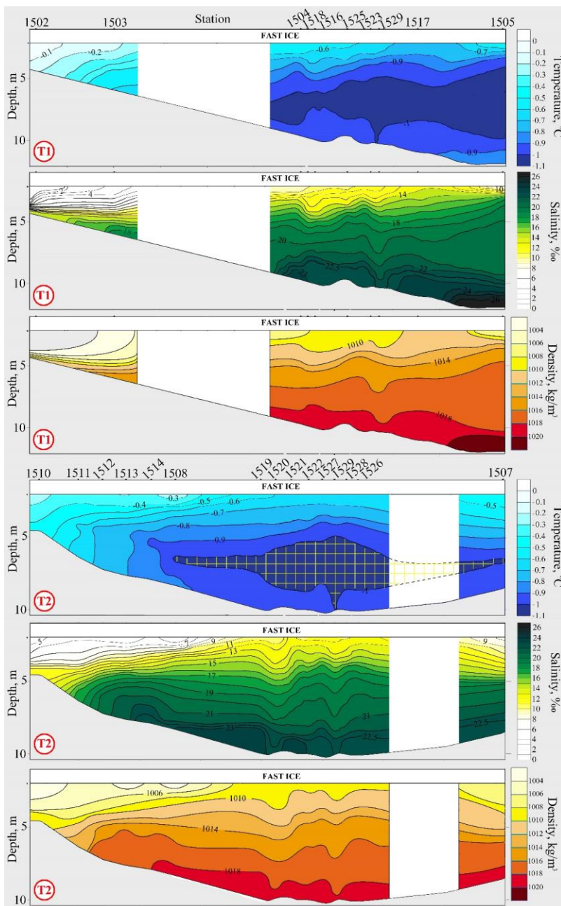
Figure 7: Vertical sections of winter salinity, temperature, and density distributions. The location of transects T1 and T2 is shown in Figure 2. A yellow cell shows a “mushroom-like structure”. In places where there are no data, white gap has shown.
