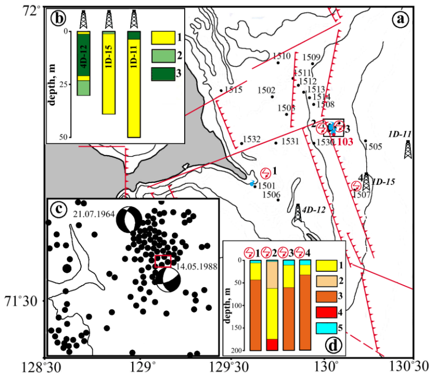
Figure 4: Location of drilling sites and oceanographic stations superimposed on a seismotectonic map modified from Imaev et al. (2004) and overview map of Fig. 2.
