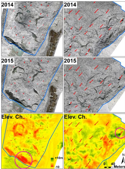
Figure 9: Locations of maximum and minimum change in ice elevation on Llaca glacier tongue. Upper row panels show 2014 orthomosaic; middle row panels show 2015 orthomosaic; lower row panels show elevation change where 2014 elevation is subtracted from 2015 elevation (i.e. negative value is ice loss). Maximum ice loss of 18m occurred at the calving face (pink circle lower left panel). Maximum gain of 11m is recorded in upper right section where a large boulder (roughly 10m tall) has moved through the scene (visible by comparison of 2014 and 2015 orthomosaics). Blue line is glacier tongue boundary, red arrows are velocity measurements. Note: elevation change values are truncated to +/-10m for display purposes. Location of panels is depicted in Figure 7 inset boxes: 3 – left panels; 1 – right panels.
