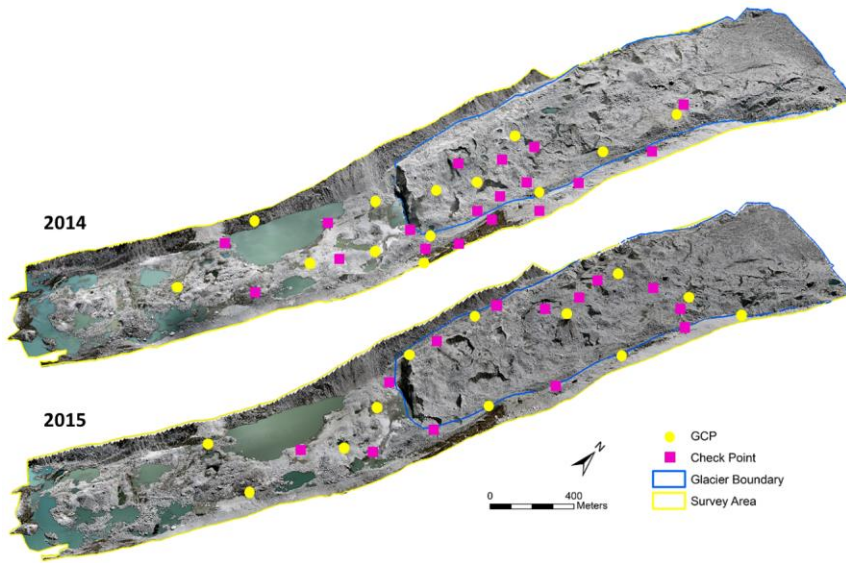
Figure 4: Photogrammetric DEM's and RGB orthomosaics of Llaca glacier tongue in 2014 (top) and 2015 (bottom), constructed through SfM workflow.
