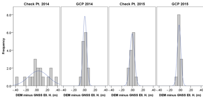
Figure 5: Histogram plot of elevation differences (errors) between check points and GCP surveyed elevations and DEM elevations for 2014 and 2015 respectively. Note: negative values indicate underestimation of DEM surface with respect to surveyed positions and thus imply flattening of the DEM surface. Most errors are less than +/-5cm and all within +/-10cm except for 2014 check points. Large 2014 check point errors are assumed to be the result of poor location selection.
