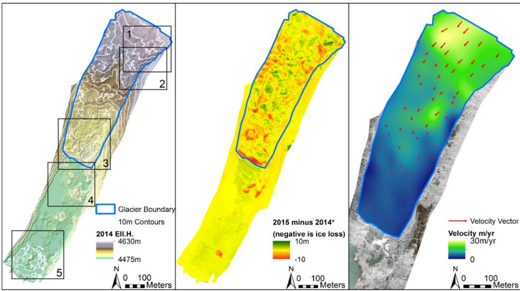
Figure 7: 2014 SfM DEM elevations (EIL.H.) (left); Vertical change in elevation from 23 July 2014 to 28 July 2015 (centre); Glacier surface velocity tracks and interpolated velocity surface (right). Numbered extent boxes depict locations of: 1 – Figure 9 right panels; 2 - Figure 11 top panels; 3 - Figure 9 left panels and Figure 11 lower panels; 4 - Figure 13 left panels; 5 - Figure 13 right panels. *Note: centre panel values are truncated to +/-10m for display purposes (see Figure 8).
