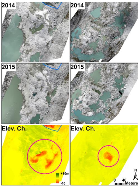
Figure 13: Locations of major elevation change (ice loss) within lake sediments (pink circles), indicate buried glacier ice is still present. Low surface velocities were also measured here (~2.5m/yr below calving face in left panels, and ~0.5m/yr at end of surveyed region in right panels, indicating these sediments are still connected to the main glacier tongue. Upper row panels show 2014 orthomosaic; middle row panels show 2015 orthomosaic; lower row panels show elevation change where 2014 elevation is subtracted from 2015 elevation (i.e. negative value is ice loss). Blue line is glacier tongue boundary. Note: elevation change values are truncated to +/-10m for display purposes. Location of panels is depicted in Figure 7 inset boxes: 4 – left panels; 5 – right panels.
