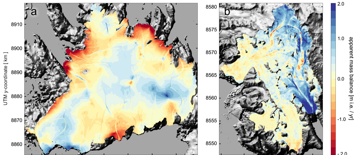
Figure A2. Apparent mass balance \dot{a} for VIC (a,c) and THPB/WSB (b,d). Panels (a,b) give the initial input as given by the SMB and the measured surface elevation changes. Panels (c,d) show the final field after adaptation of \dot{a} during the optimisation in accordance with the cost function. Background: grey-scale hill-shaded topography based on a NPI 50 m DEM.
