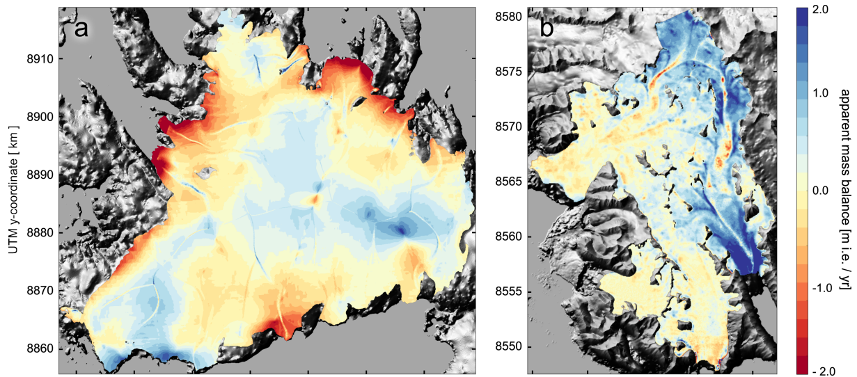
Figure A2. Apparent Final apparent mass balance \dot{a} for VIC (a,e) and THPB/WSB (b,d) . Panels (a,b) give after minimisation of the initial input as given by the SMB and the measured surface elevation changes cost function. Panels (e)During this minimisation, (d) show the final field after adaptation - \dot{a} is iteratively adjusted. The input values of \dot{a} during the optimisation are presented in accordance with the cost function Fig. 2e,f. Background: grey-scale hill-shaded topography based on a NPI 50 m DEM.
