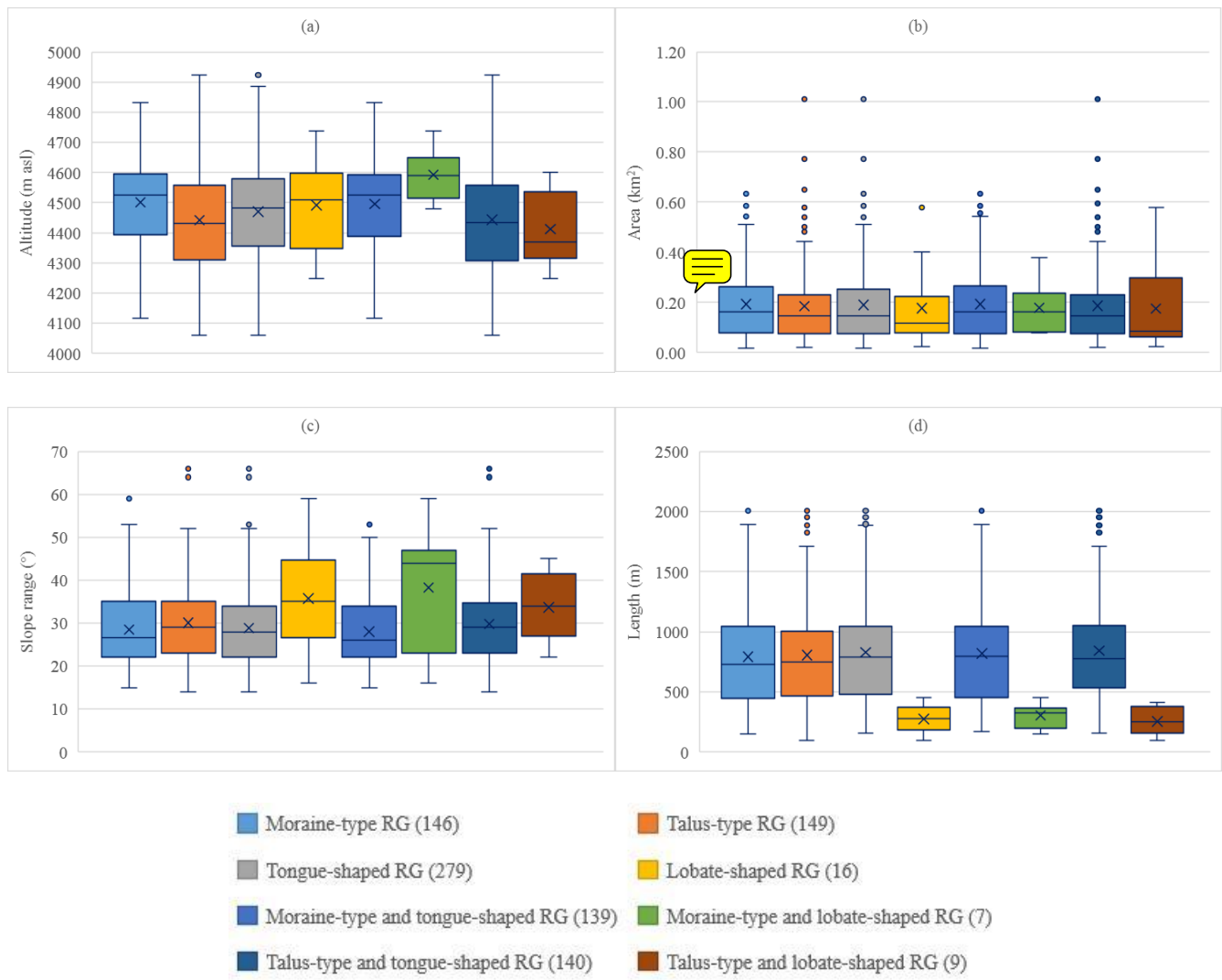
Figure 4: Boxplots illustrating the distributional characteristics of rock glaciers in Daxue Shan: (a) average altitude (m asl); (b) area (km 2 ); (c) range in the gradient of the slope (°); and (d) length (m). Boxplots represent 25-75% of all values, the caps at the ends of the vertical lines represent 10-90% of values, and the line in the center of each box indicates the median value. The number of the population of the different kinds of rock glacier is in the brackets of the legend.
