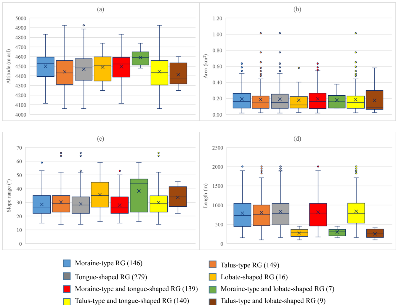
Figure 4: Boxplots illustrating the distributional characteristics of rock glaciers in Daxue Shan: (a) average altitude (m asl); (b) area (km 2 ); (c) range in the gradient of the slope (°); and (d) length (m). Boxplots represent 25–75 % of all values, the caps at the ends of the vertical lines represent 10–90 % of values, and the line in the center of each box indicates the median value. The number of the population of the different kinds of rock glacier is in the brackets of the legend.
